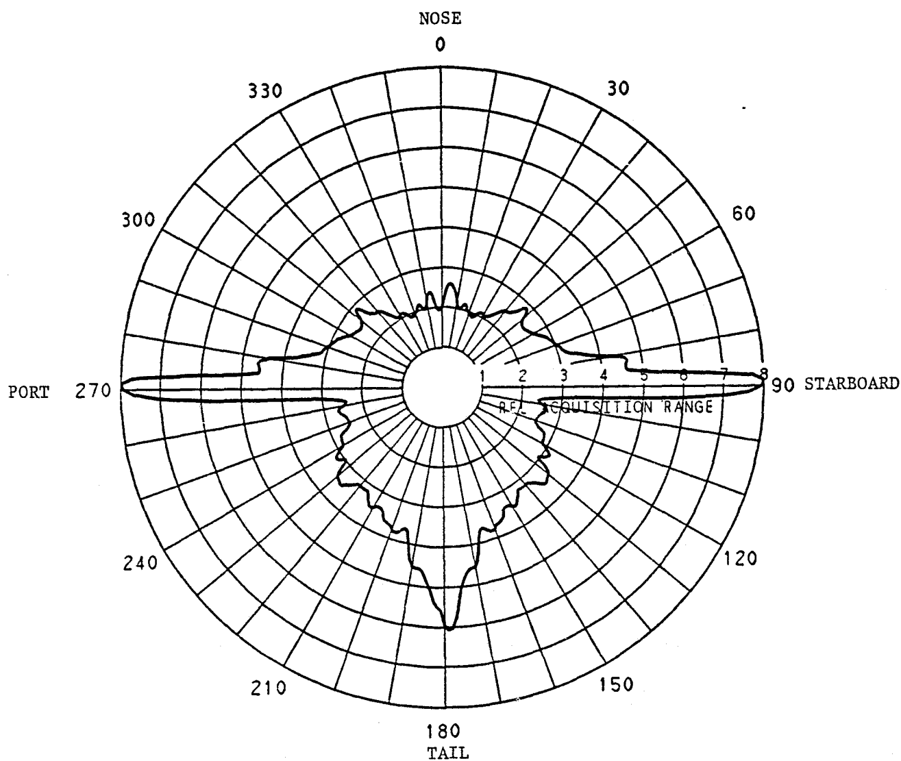
Figure 32. Fourth Root of Median Radar Cross Section of Space Shuttle Orbiter, +10 Degrees Tilt Angle.
