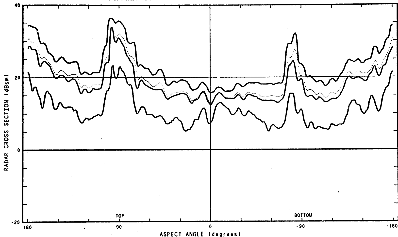
Figure 25. 10th, 50th, and 90th Percentiles and Mean of Radar Cross Section of Space Shuttle Orbiter, +70 Degrees Roll Angle.
