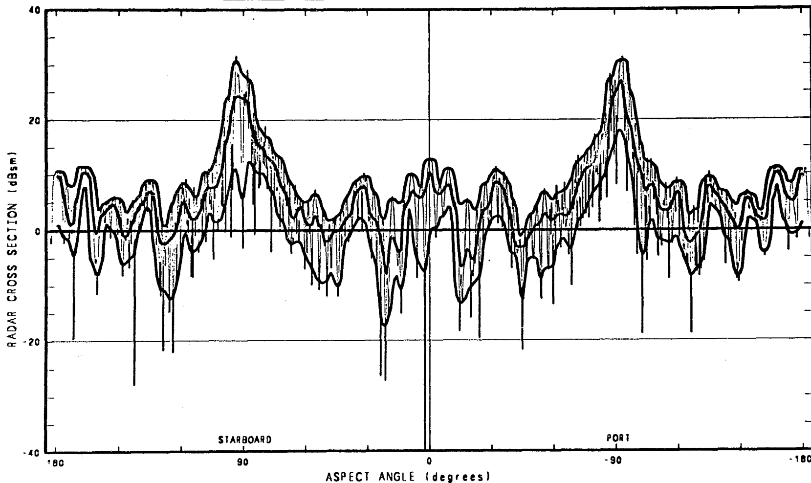
Figure 11. 10th, 50th, and 90th Percentiles Superimposed on Radar Cross Section Pattern.
