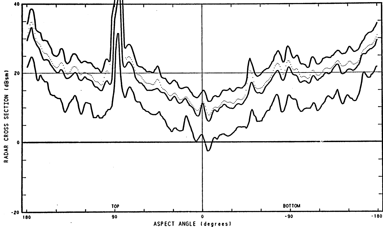
Figure 19. 10th, 50th, and 90th Percentiles and Mean of Radar Cross Section of Space Shuttle Orbiter, -10 Degrees Roll Angle.
