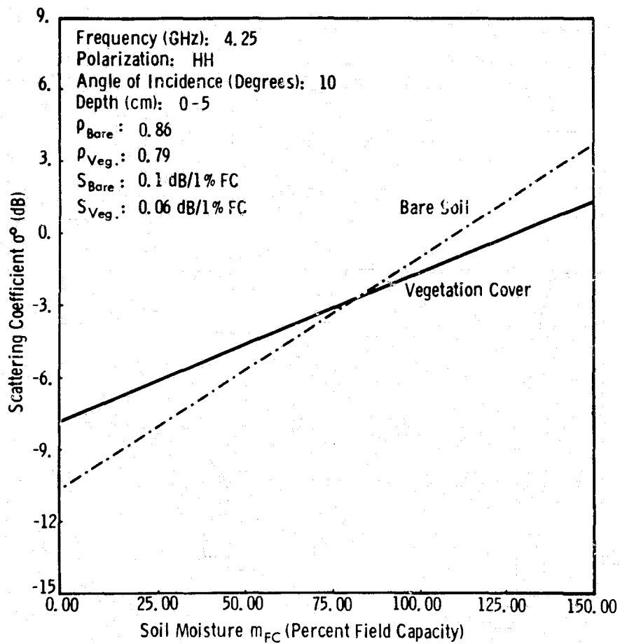
Fig. 5-9. Comparison of bare soil and vegetation cover \sigma^{\circ} dependence on soil moisture.
