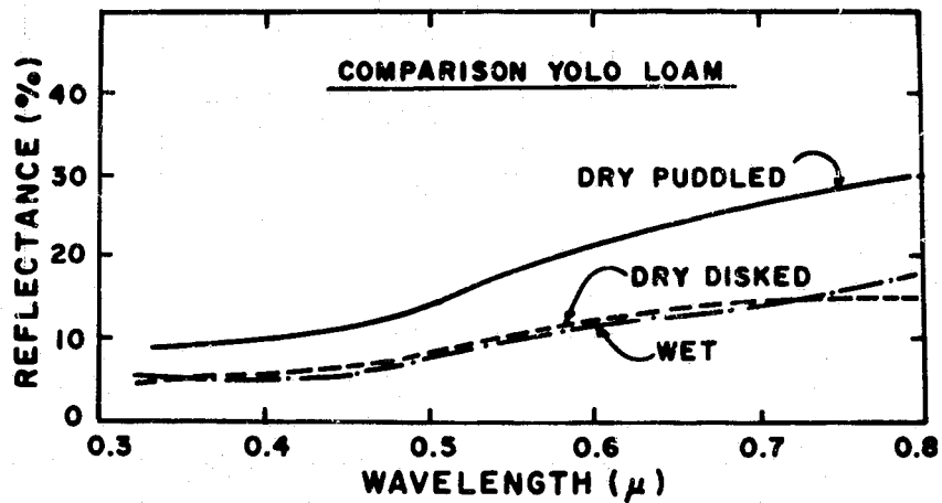
Fig. 4-4. Directional spectral reflectance of a bare Yolo loam field under three surface conditions. Measurements were made for a solar zenith angle \theta = 30^\circ (after Coulson and Reynolds, 1971).
