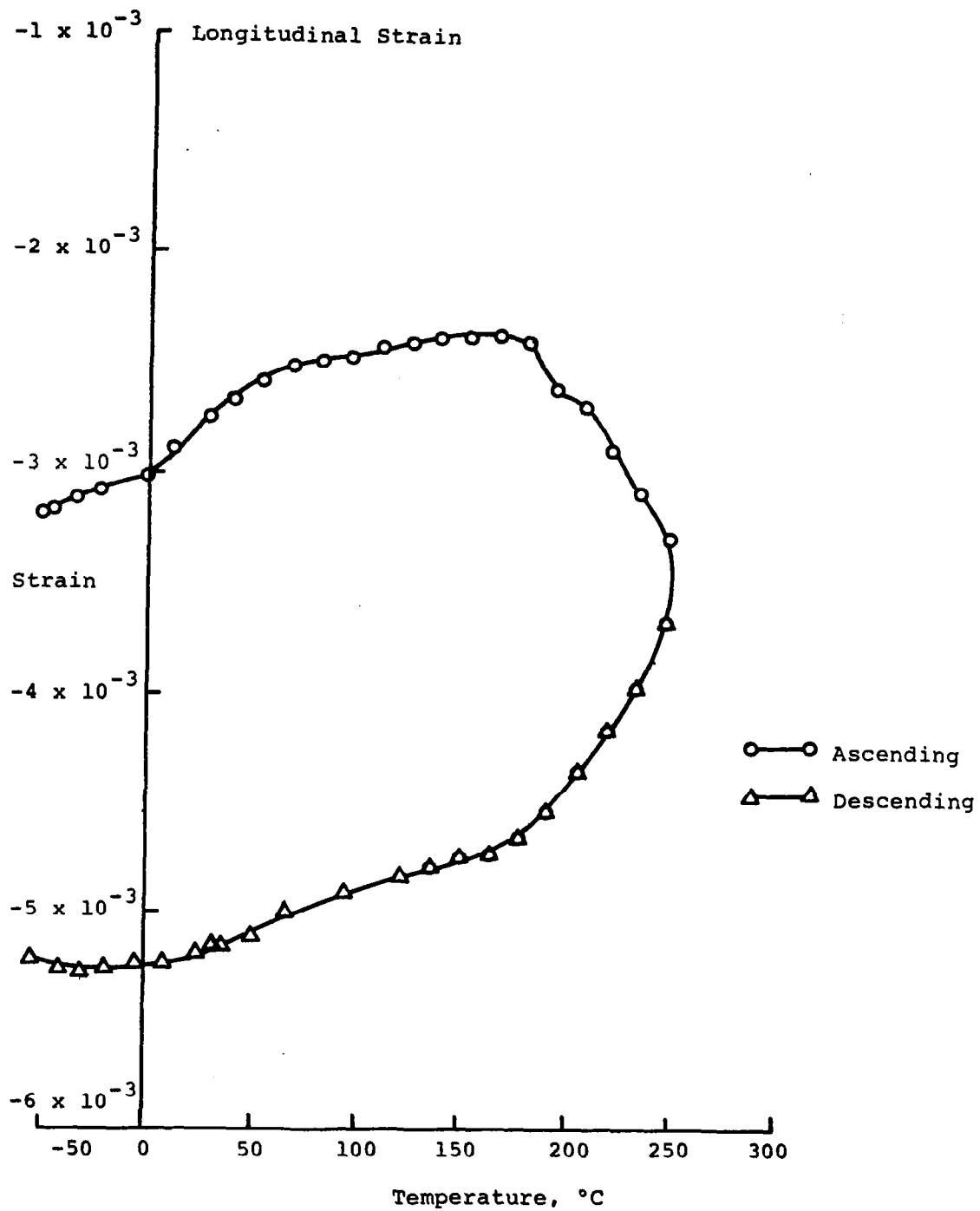
Figure 5. Longitudinal Strain ( \epsilon_p - \epsilon_q ) versus Temperature Load = -1473 \text{ N } (-150 \text{ kg}) \quad \sigma_{11} = -35.37 \text{ MPa}
