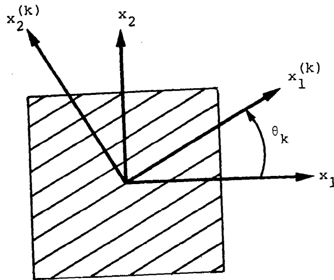
Figure 2. Laminate Coordinate System
