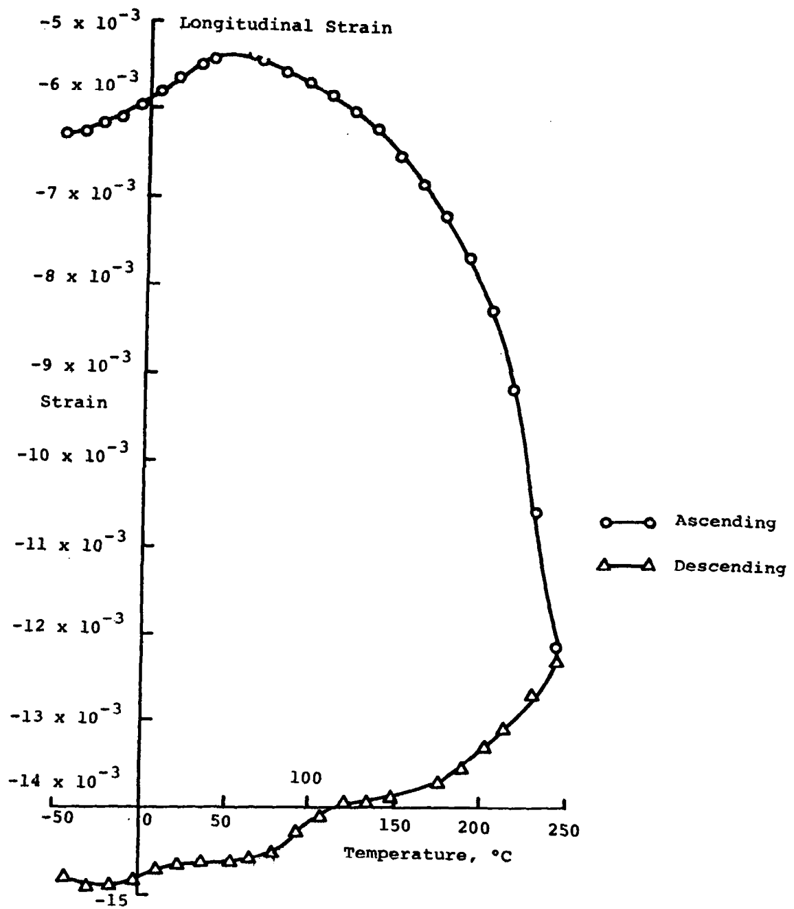
Figure 7. Longitudinal Strain versus Temperature Load = -2946 N (-300 kg) \sigma_{11} = -70.74 MPa
