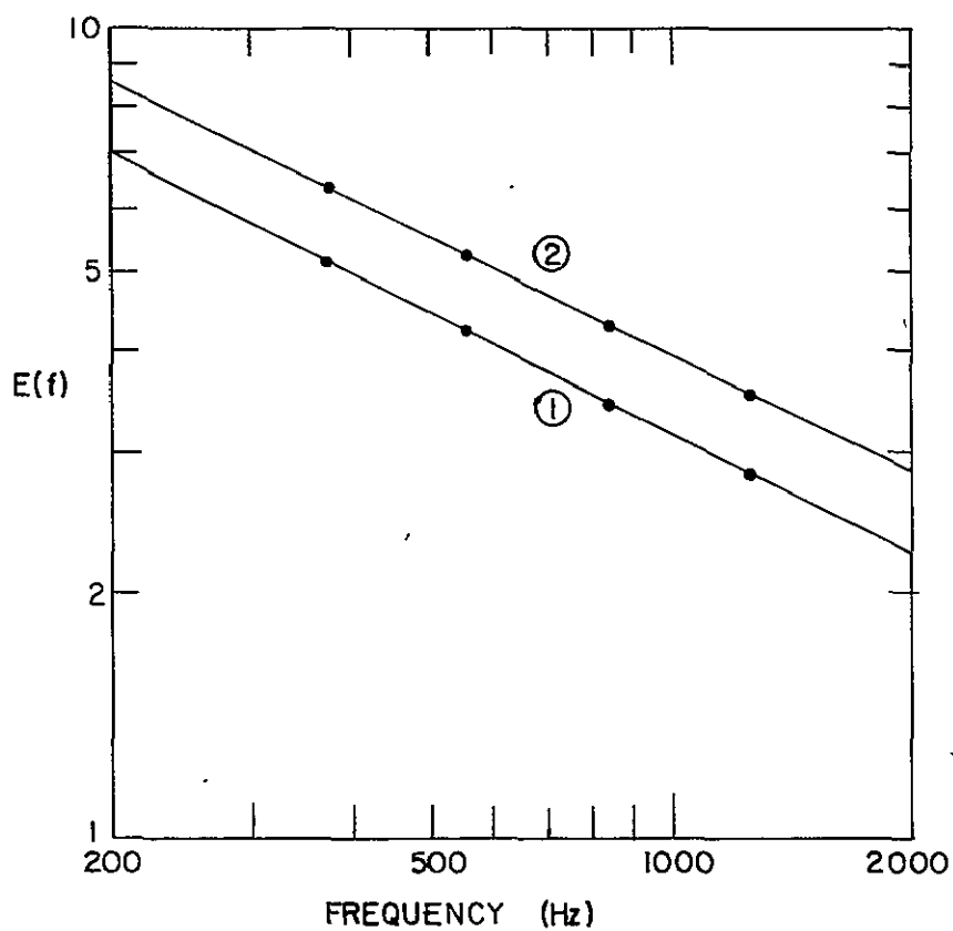
Figure 4.9 The effect of filter response on a spectrum having an index of -0.5 . Line 1 is the assumed spectrum; line 2 is the calculated spectrum resulting from non-ideal response of the band-pass filter.
