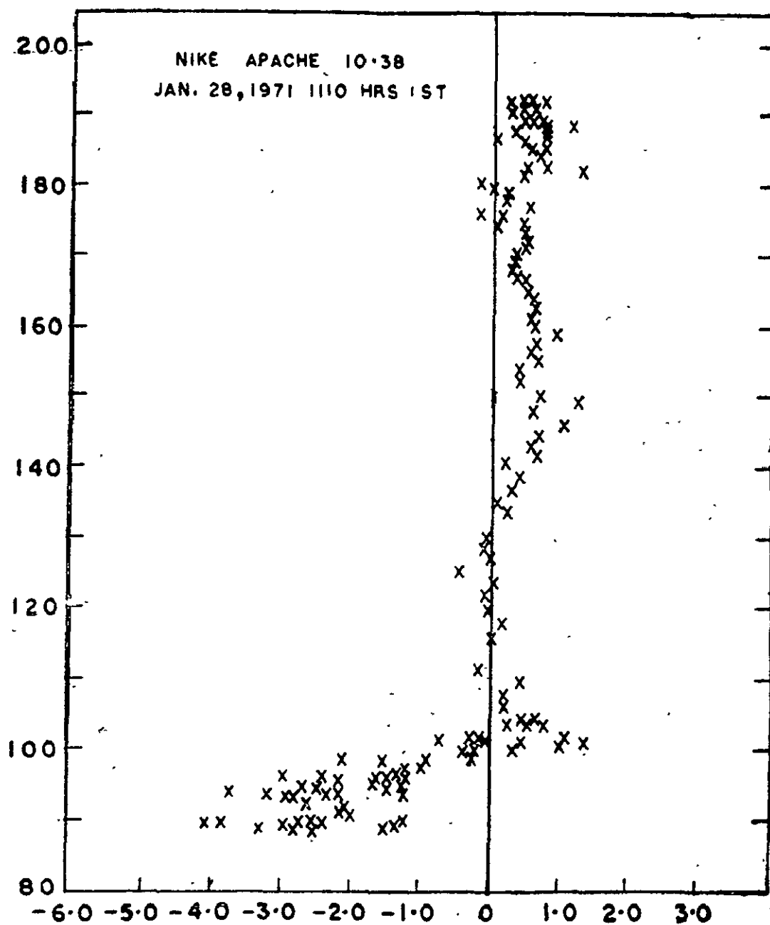
Figure 4.13 Spectral index n obtained from E(k) \propto k^n for the 1 to 15 m irregularities of flight 10.38. The results for flight 10.37 were similar to those of 10.38 [Prakash et al. , 1972].
