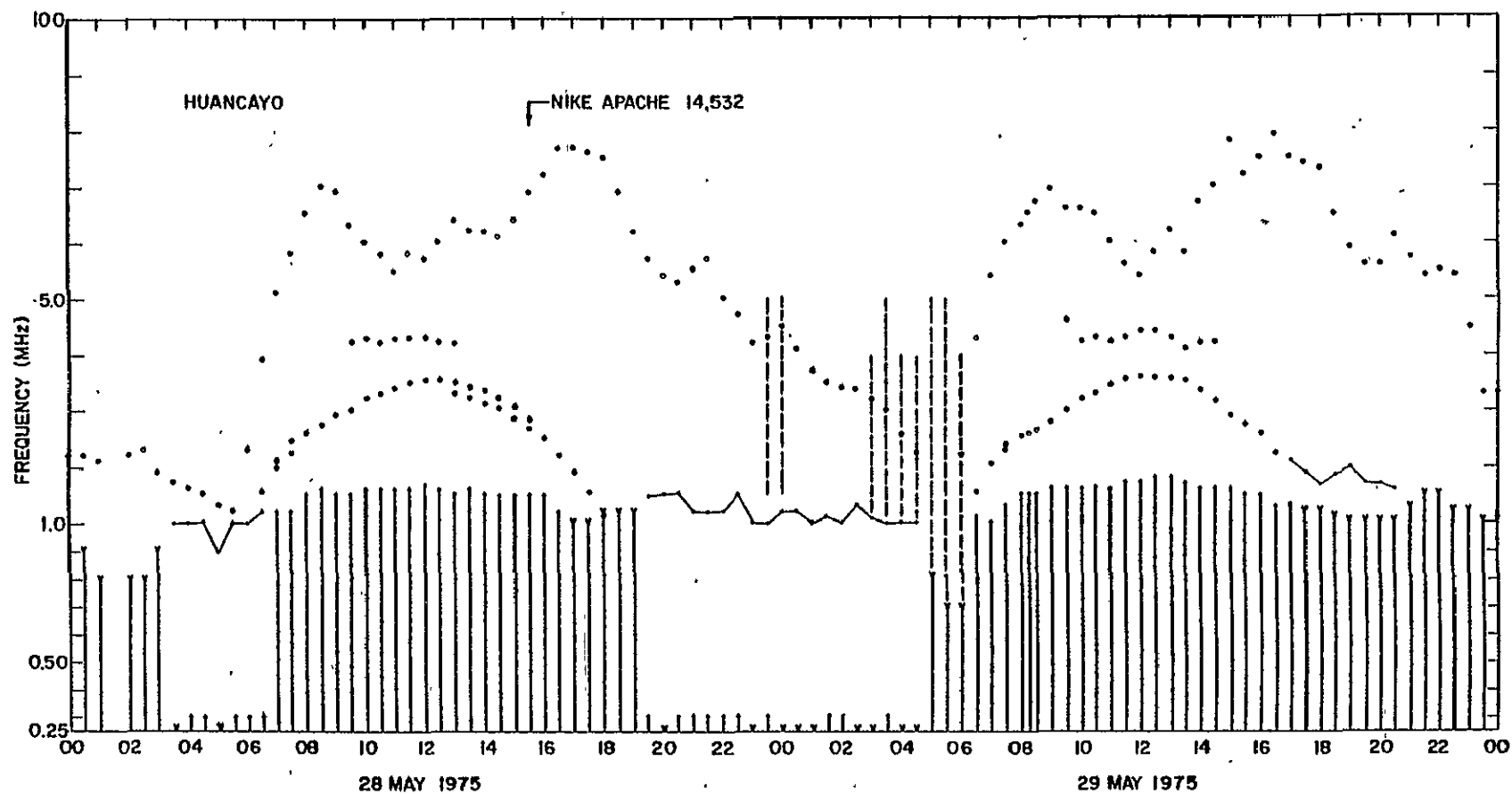
Figure 4.2 Huancayo f -plots for 28 and 29 May 1975. The launch time of Nike Apache 14.532 is indicated. [Data obtained from WDC-A for Solar-Terrestrial Physics].
