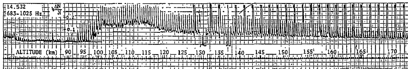
Figure 4.5 Amplitude of electron-density fluctuations in the size range 1.2 to 1.7 m observed on Nike Apache 14.532. The large vertical spikes result from interference from other instrumentation in the payload.
