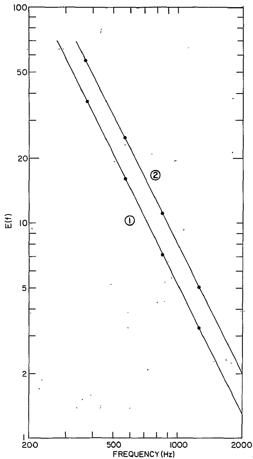
Figure 4.10 The effect of filter response on a spectrum having an index of -2.0. Line 1 is the assumed spectrum, line 2 is the calculated spectrum resulting from non-ideal response of the band-pass filter.
