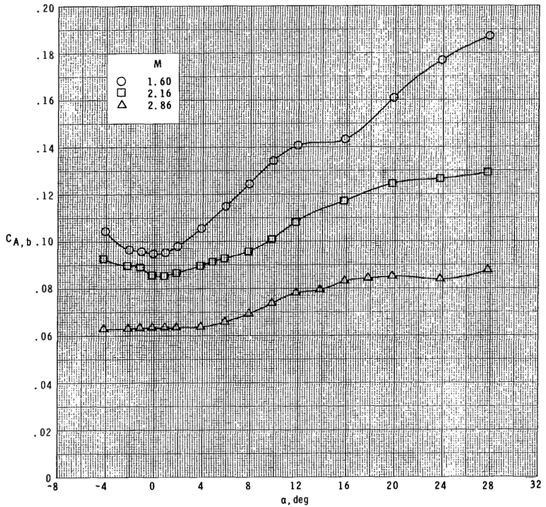
Figure 13.- Variation of base drag at angle of attack for body-tail, cranked wing, nose strakes, and radar nose configuration.
