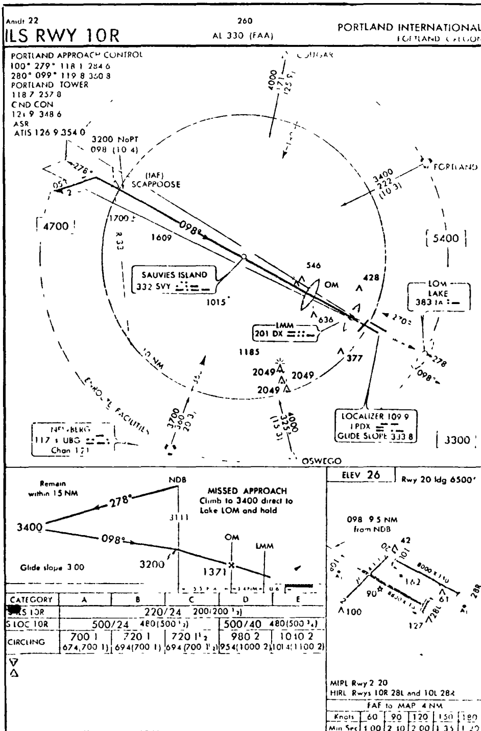
Figure 6.- Typical runway approach plate.
