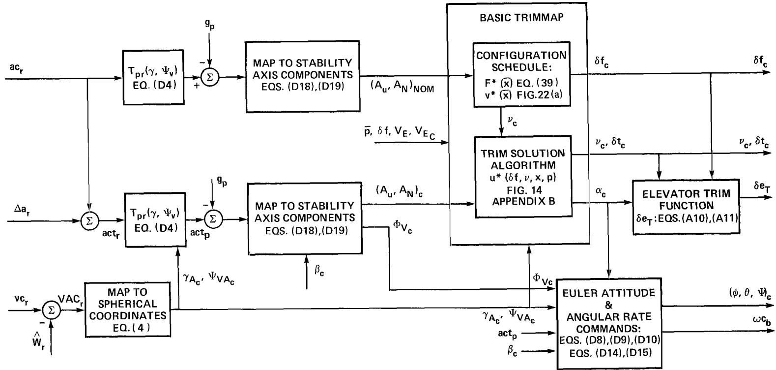
Figure 25.- AWJSRA Force Trimmap.
