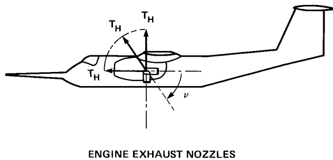
Figure 7.- Augmentor wing jet STOL research aircraft (AWJSRA).
