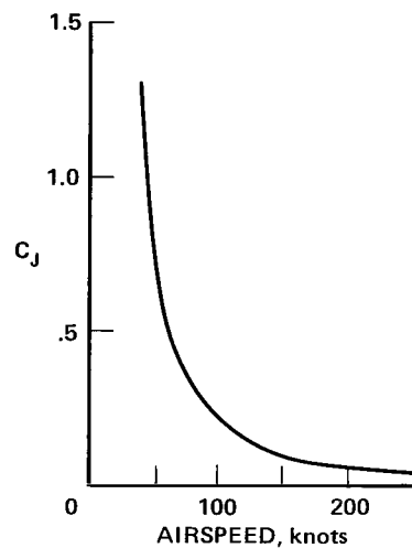
(c) Effect of airspeed on C_J at maximum continuous power.
