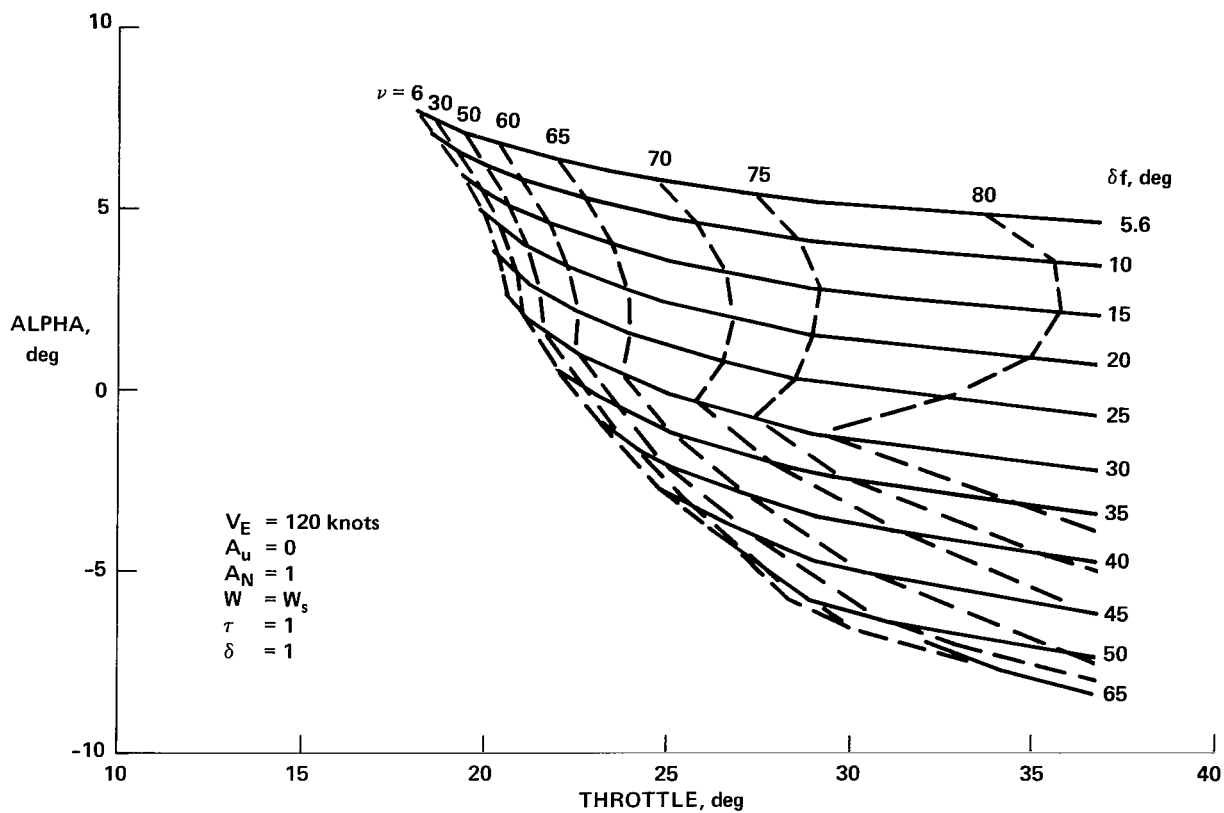
(a) Level flight.
