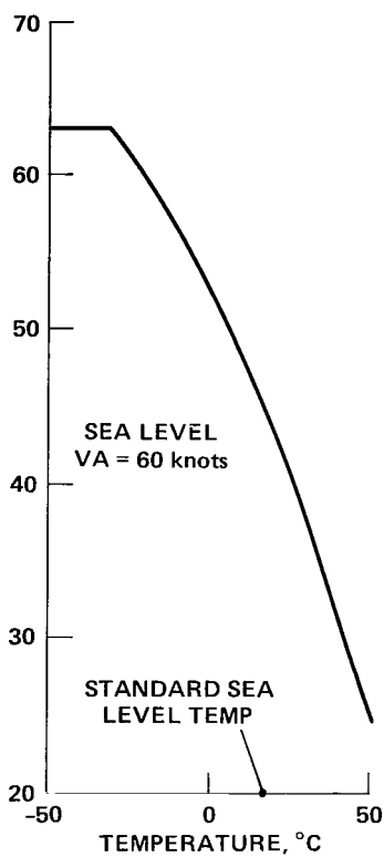
(b) Effect of temperature on maximum continuous hot thrust.
