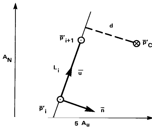
Figure 37.- Minimum distance from \bar{p}'_C to a line segment, L .
