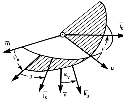
Sketch (e).- Stability and path axes.
