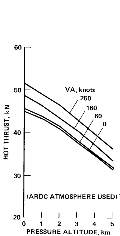
(a) Effect of altitude and airspeed on maximum continuous hot thrust.
