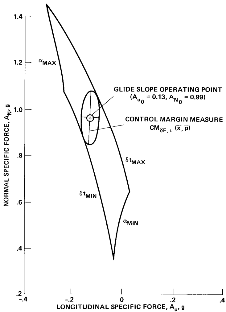
Figure 11.- Regulator control regime - fixed nozzle mode; V_E = 65 knots, \delta_f = 65^\circ , \nu = 84.2^\circ , p = p_s .
