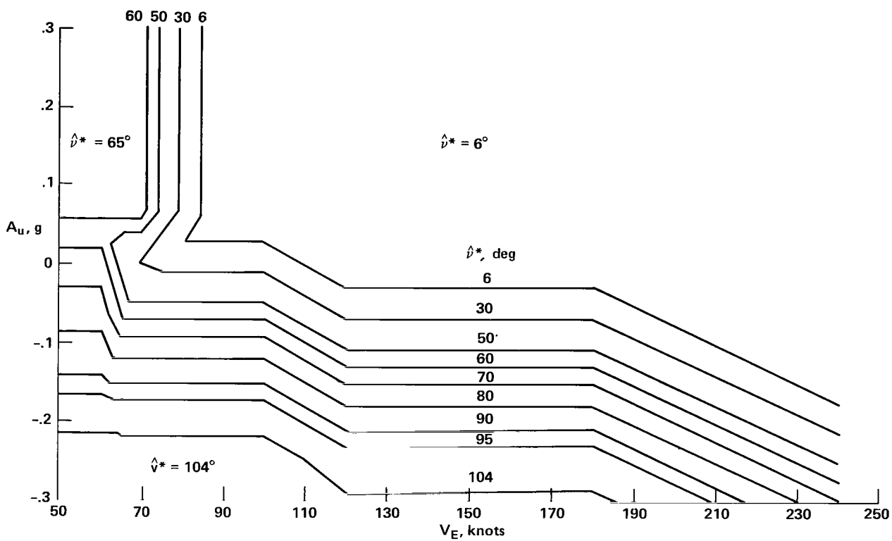
(b) Nozzle schedule - contour plot ( A_N = 1 ).
