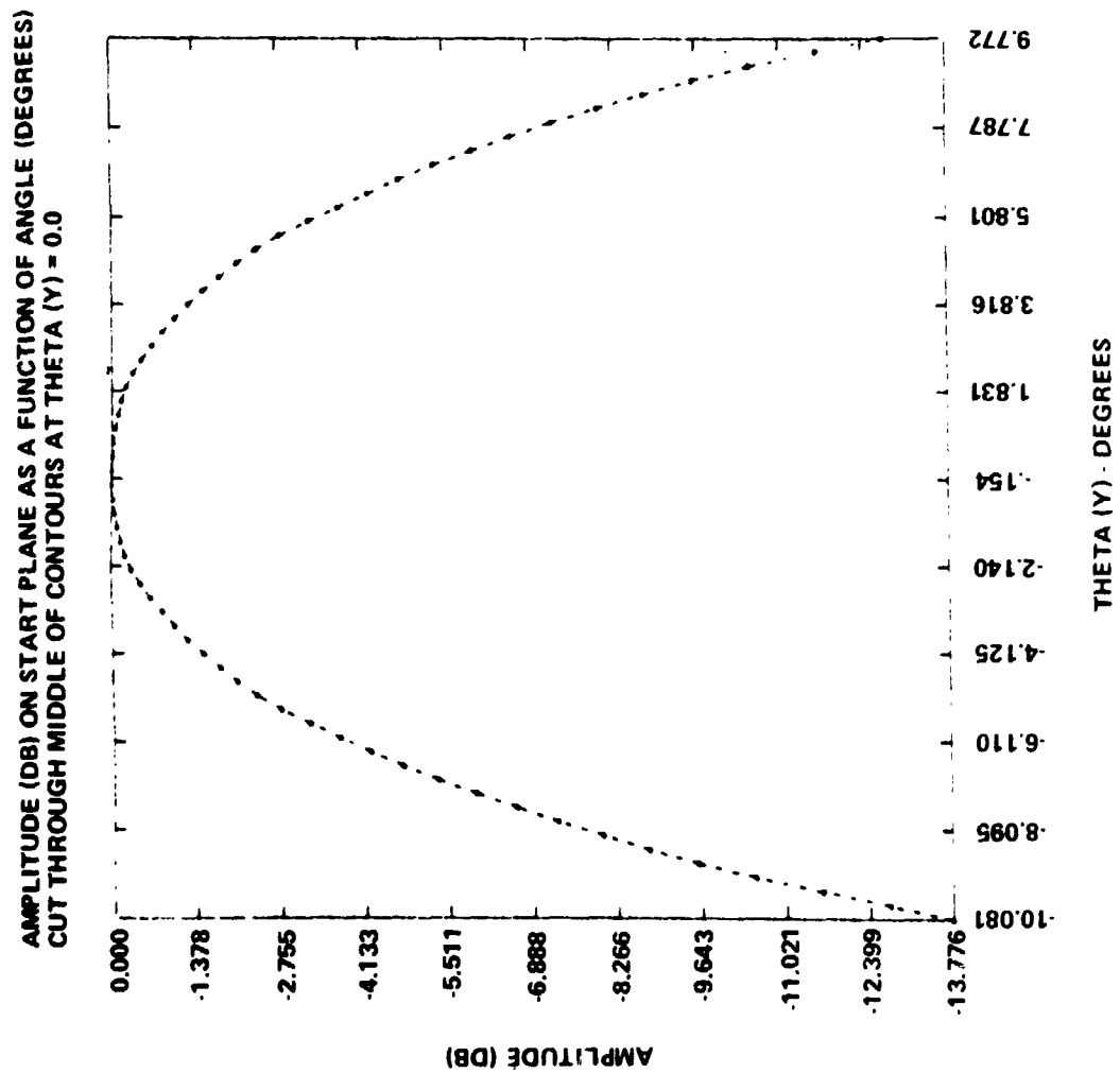
Figure 18. S-band antenna pattern (field amplitude |\psi| ) used in calculations.
