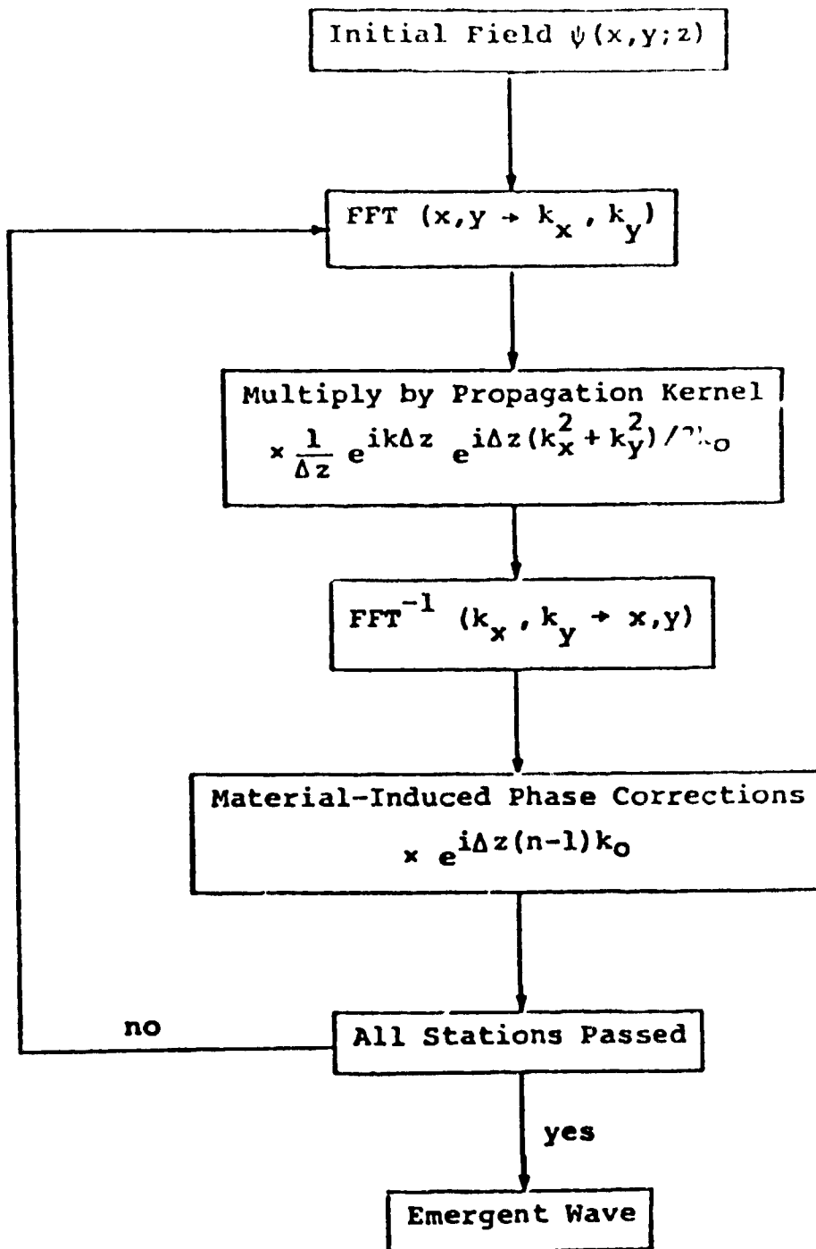
Figure 1. Schematic process of evaluation of signal propagation in an absorbing and refracting medium.
