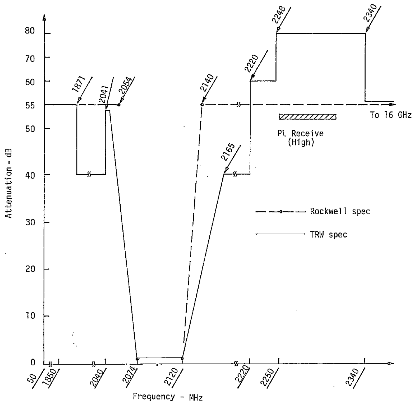
Figure 13. NASA High Mode Transmit Filter
