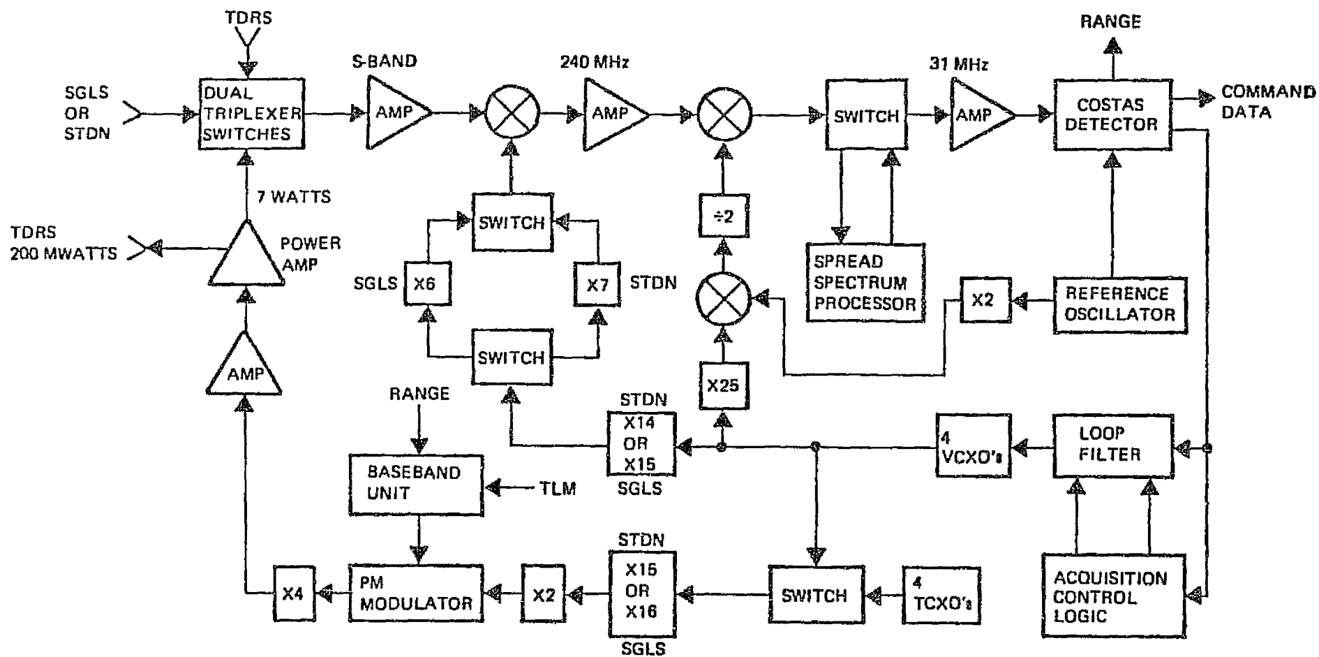
Figure 1. S-Band Network Transponder Block Diagram
