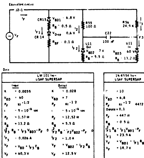
FIGURE 3. TYPICAL CIRCUIT FOR LIGHTNING TRANSIENT ANALYSIS.
