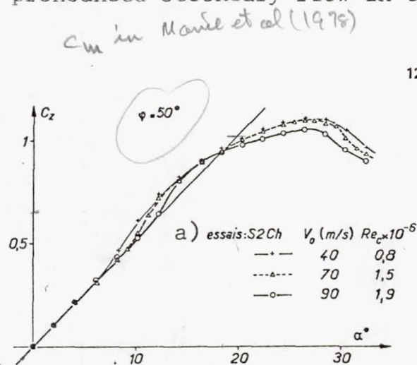
Fig. 8. - Influence of Reynolds Number on Lift Key: a) tests
