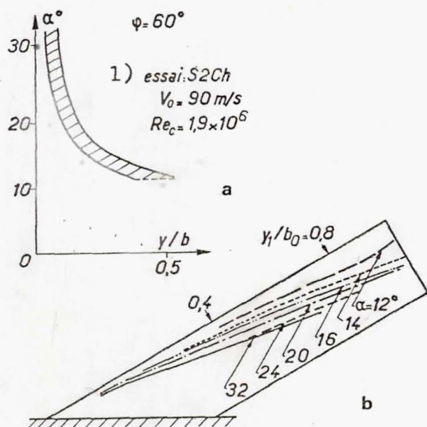
Fig. 6. - Vortex flow characteristics a) path depending on the dimensions of the origin of the vortexes b) approximate positions of the vortex axis as a function of the angle of attack Key: 1) test, S2Ch
