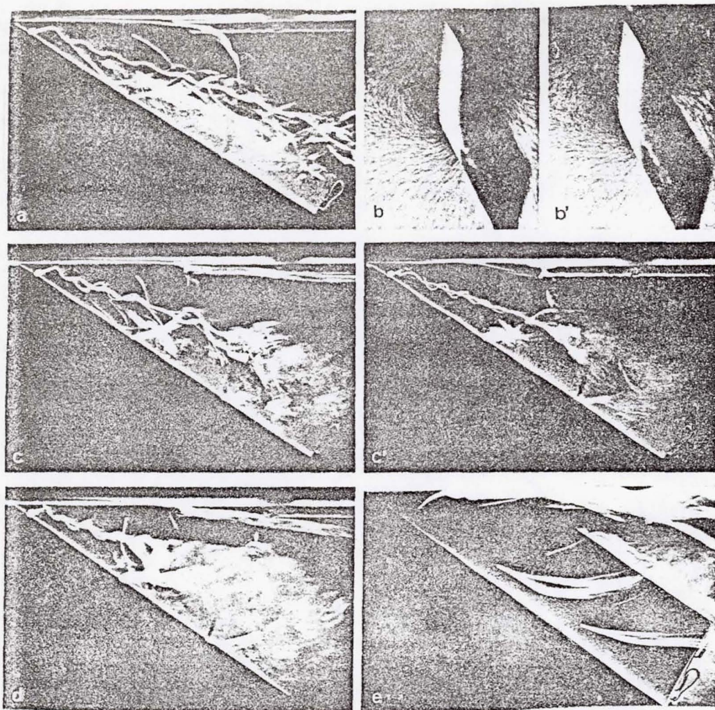
Fig. 12 - Flow around a model of a complete wing (water tunnel - Re \approx 0.5 \times 10^4 except when indicated otherwise). Views of the upper surface (a, c, c', d) and of the lower surface (e) cross-sections (b, b') - top \alpha = 20^\circ - middle \alpha = 25^\circ ( Re_c \approx 10^4 for b' and c') - bottom \alpha = 30^\circ .
