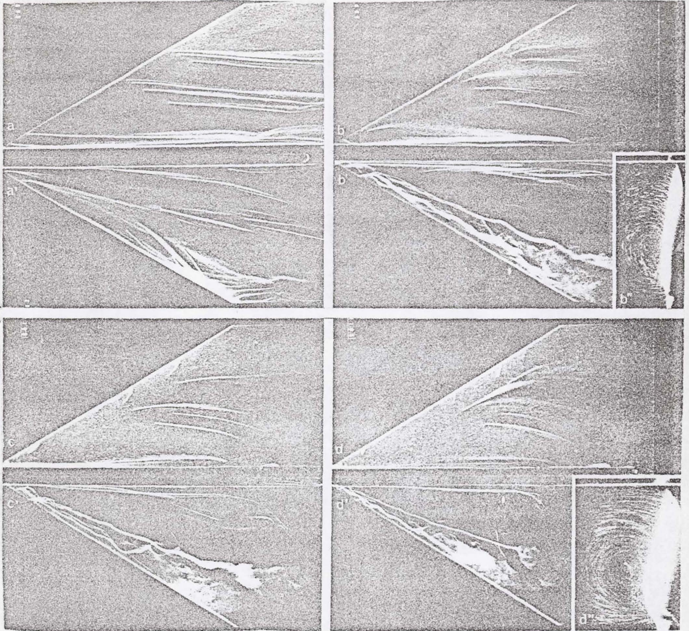
Fig. 16 - Effect of the angle of attack \alpha on the flow around /11 an enlarged wing model (water tunnel - Re \approx 10^4 ). Views of the lower surface (a, c, c, d) and the upper surface (a', b', c', d'). Cross-sections (b'', d'') downstream from the trailing edge of the socket section. \alpha = 5^\circ (a, a'), \alpha = 15^\circ (b, b', b''), \alpha = 20^\circ (c, c') and \alpha = 25^\circ (d, d', d'').
