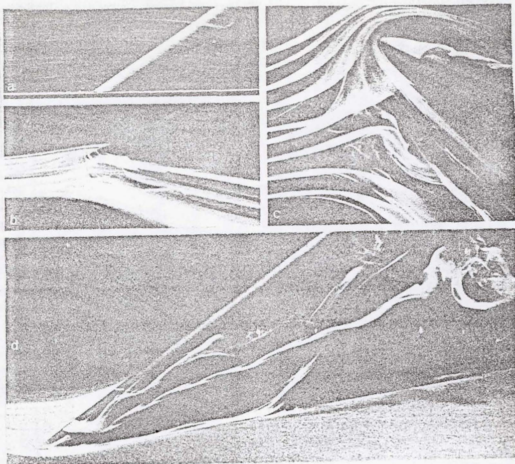
Fig. 17 - Flow around a model of an enlarged apex at a 25^\circ angle of attack (water tunnel Re_\infty \approx 0.5 \times 10^4 ). Views of the upper surface (d), of a wing c section (c), of the lower surface (b), a longitudinal section passing through the apex (a) visualized by air bubbles. /12
