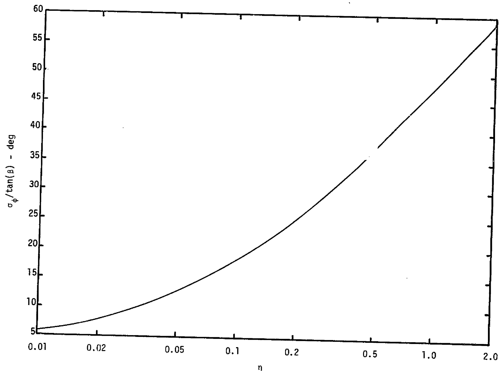
Figure 22. Tracking Loop Phase Noise
