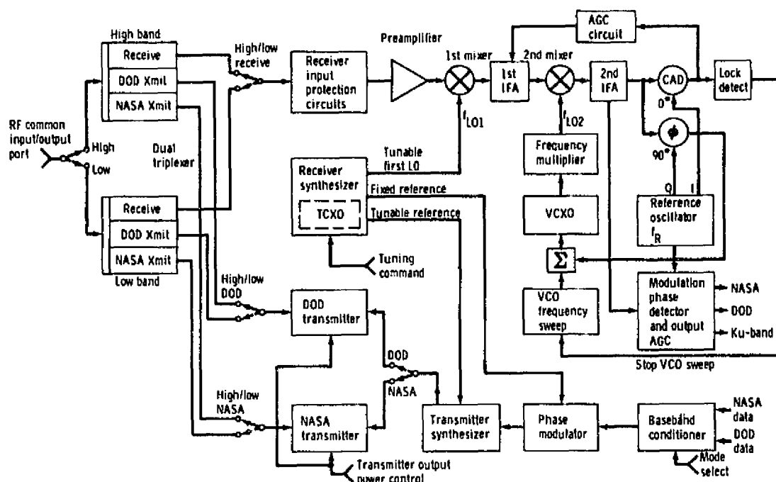
Figure 7. Payload Interrogator Functional Block Diagram
