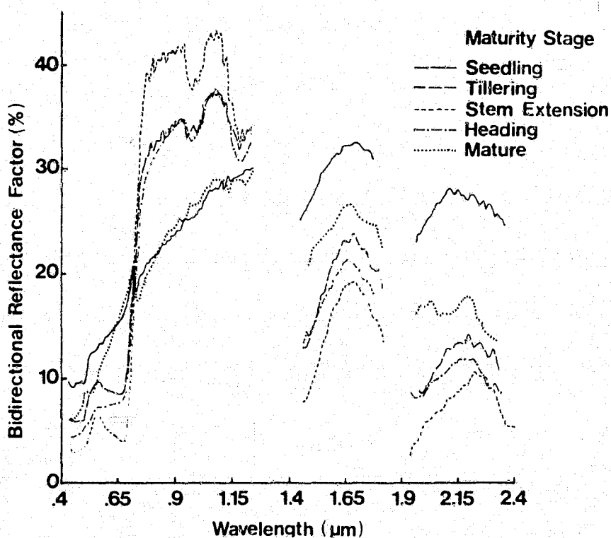
Figure A-6. Spectral reflectance of spring wheat canopies at several maturity stages. Measurements were made at Williston, North Dakota during May-August, 1976 and include plots with different soil moisture levels, planting dates, nitrogen fertilization and cultivars.
