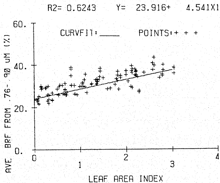
Figure B-5. Example of polynomial curve fitting using EXOSYDV software.
