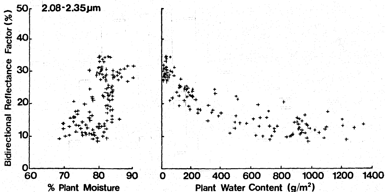
Figure A-5. Relationship of two measures of plant moisture, percent plant moisture and plant water content, to middle infrared reflectance of spring wheat canopies.
