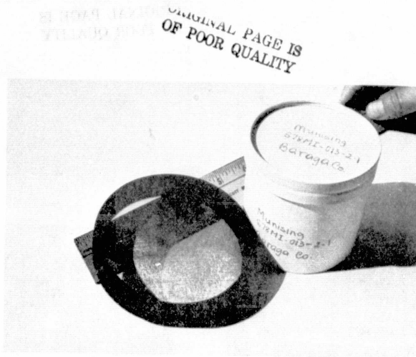
a. 10 cm diameter sample holder with soil container.
