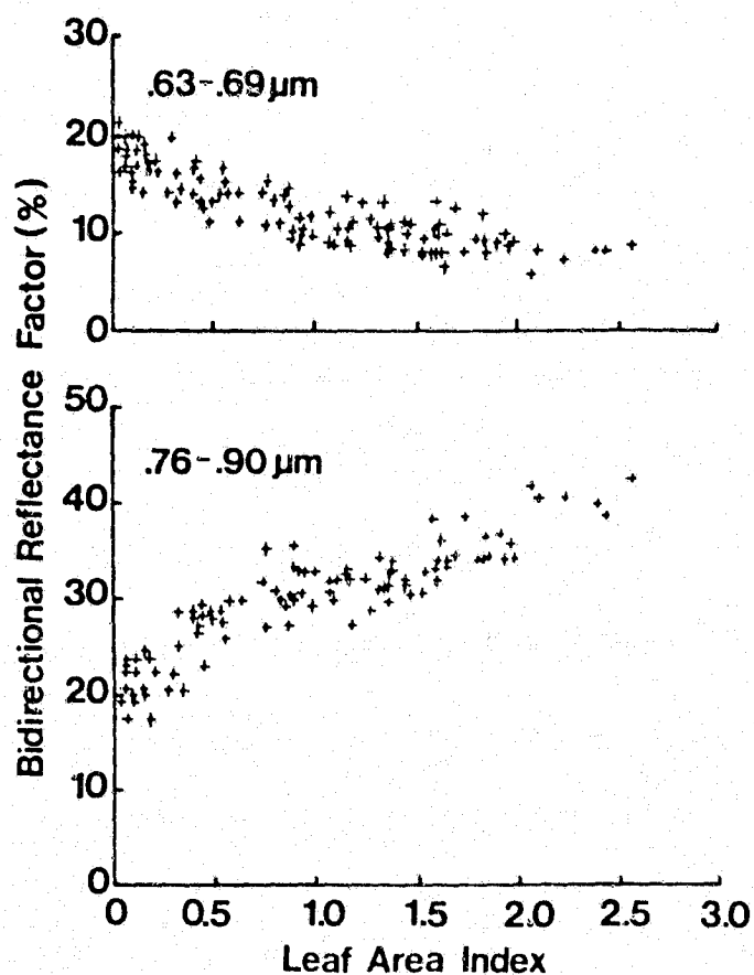
Figure A-2. Relationship of leaf area index to reflectances in the chlorophyll absorption (0.63-0.69 \mu\text{m} ) and near infrared (0.76-0.90 \mu\text{m} ) regions. Measurements for seedling through flowering stages of maturity are included for 16 treatments representing different levels of soil moisture availability, planting dates, nitrogen fertilization, and cultivar.
