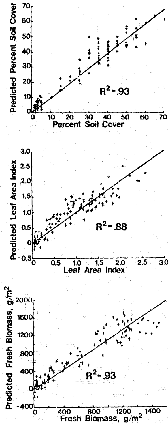
Figure A-8. Comparison of measured and predicted percent soil cover, leaf area index, and fresh biomass of spring wheat canopies.
