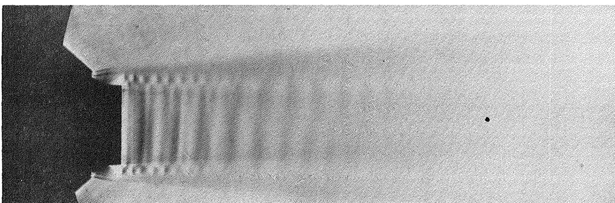
(e) \xi_p = 1.797
