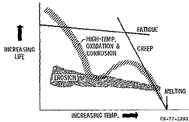
Figure 40. - Schematic of turbine blade life limits.
