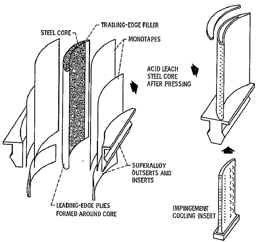
Figure 22. - Composite blade assembly schematic.
