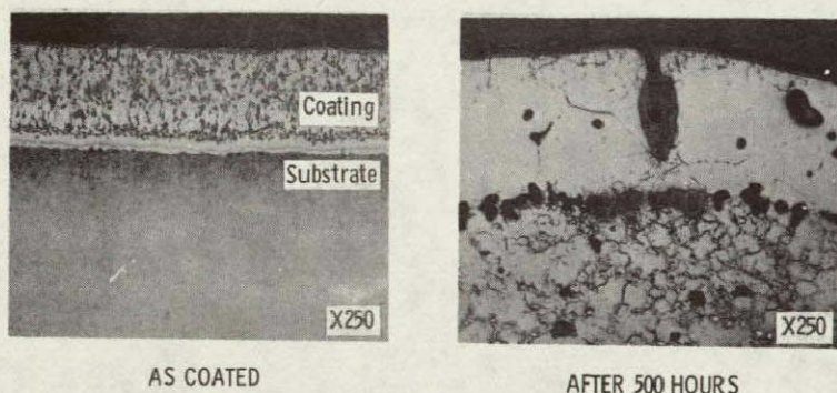
Figure 29. - Effect of ultrahigh-velocity, Mach 1 burner-rig oxidation of TD-NiCrAl + NiCrAlY overlay coating. Cycling conditions: 1100°C (2010°F) for 1 hr → RT for 3 min.
