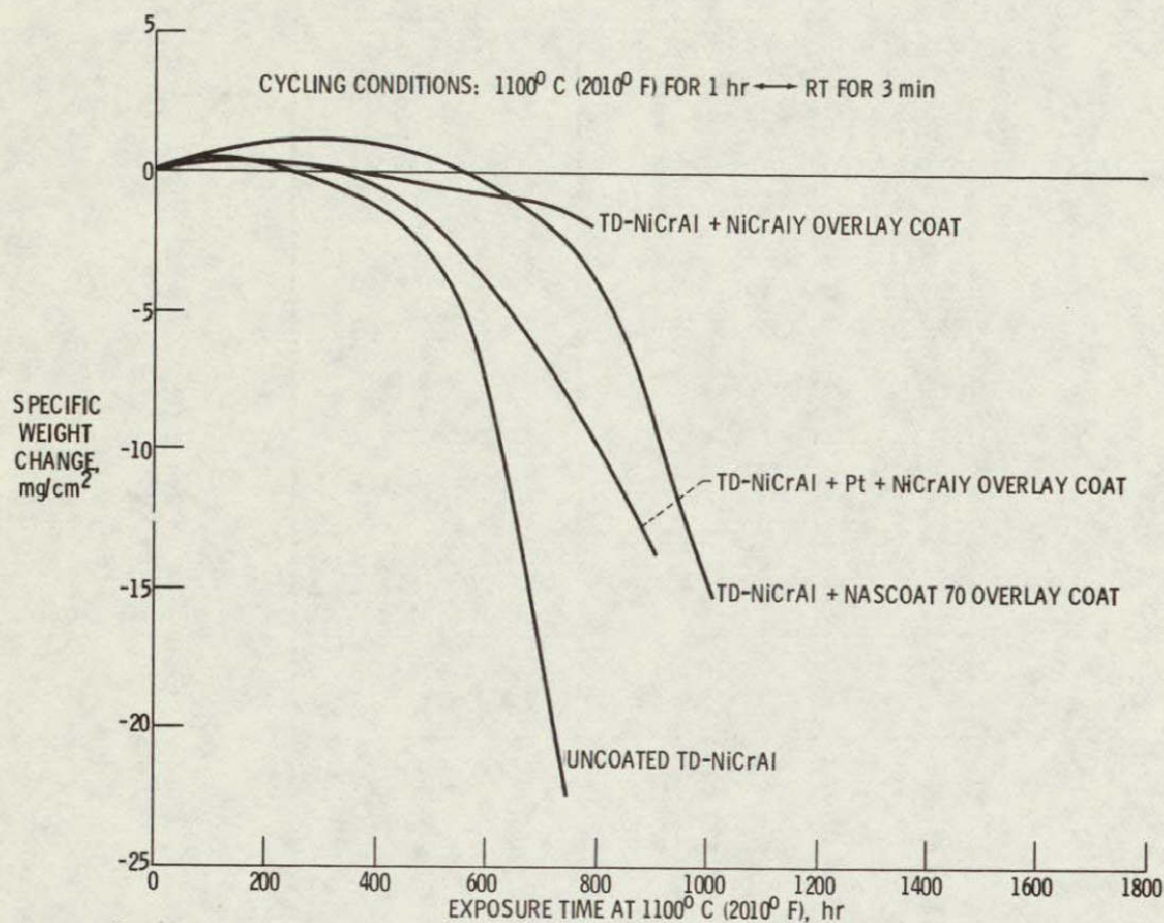
Figure 28. - Mach 1 burner rig oxidation of TD-NiCrAl at 1100°C (2010°F).
