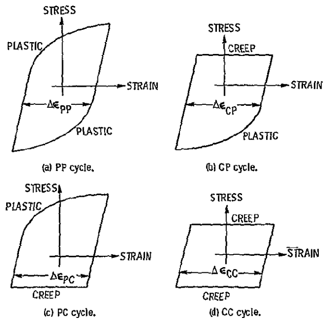
Figure 41. - Idealized hysteresis loops used in defining individually partitioned strainrange-life relationships.
