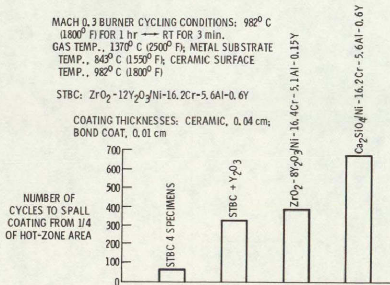
Figure 37. - Modifications to Standard Thermal Barrier Coating (STBC) improve tolerance to Na and V fuel contaminants (5 ppm Na + 2 ppm V).
