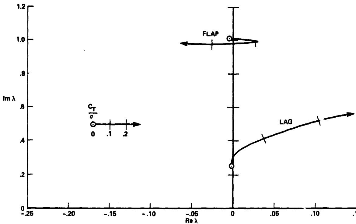
(a) Pitch-lag coupling R_{\zeta} = .3 .
