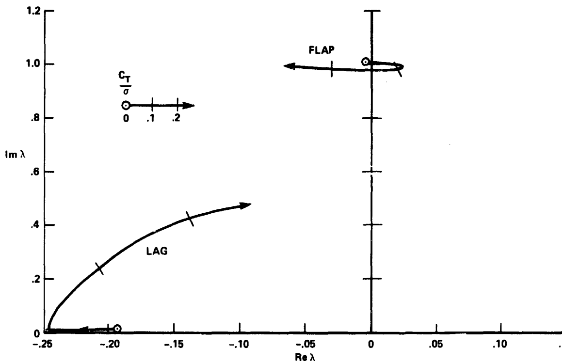
(b) Lag structural damping g_z = .5
