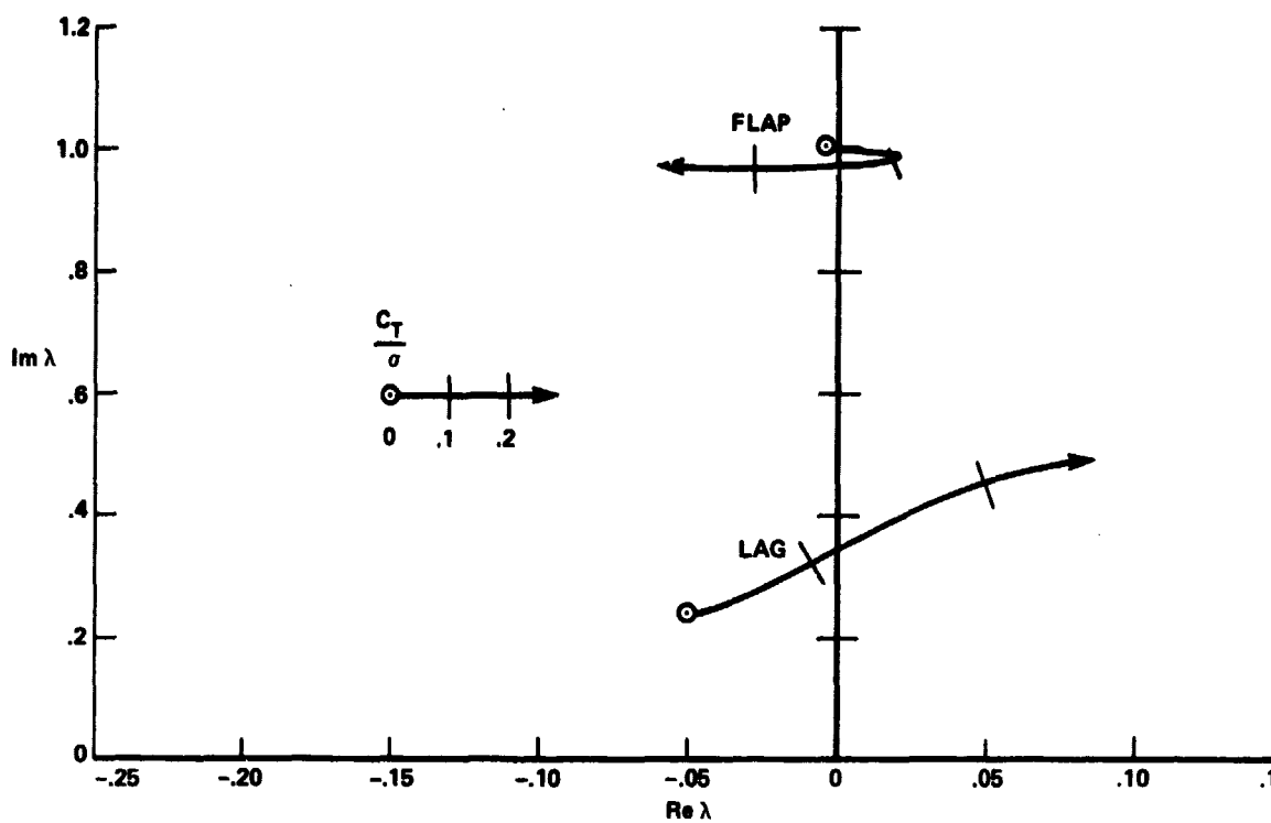
(a) Lag structural damping g_z = .1
