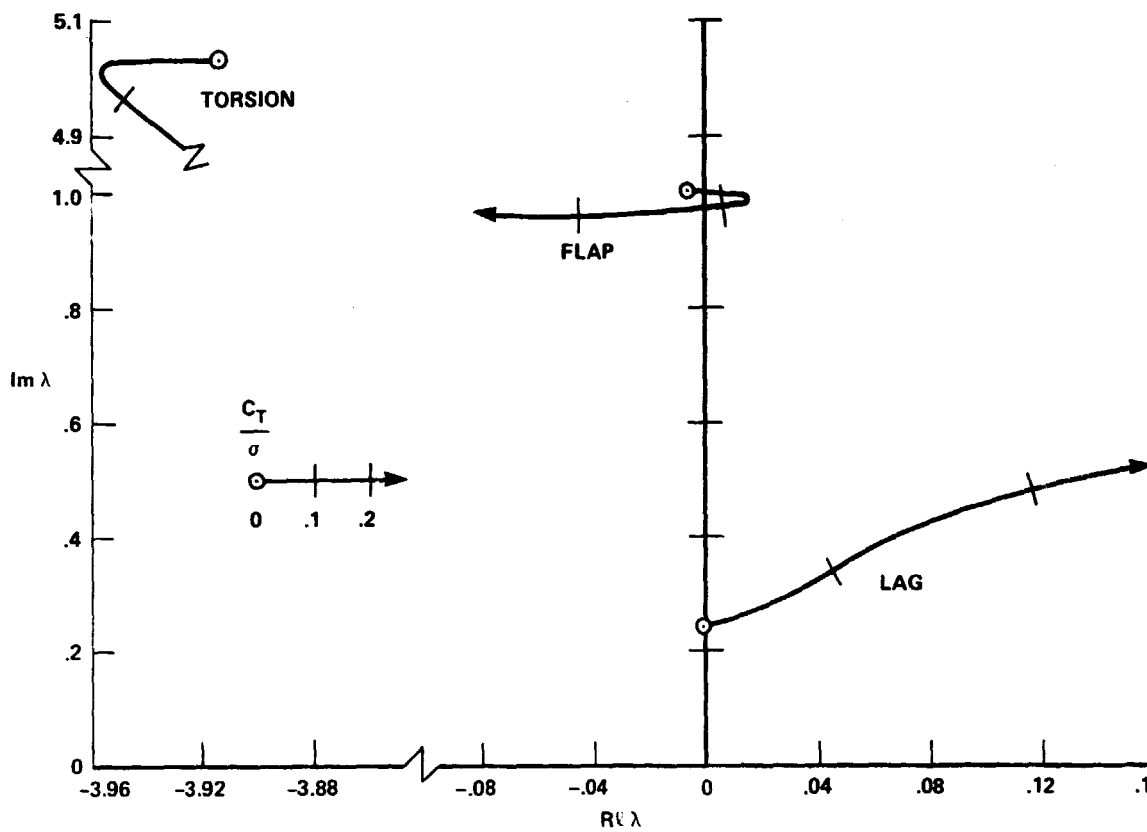
Figure 6.- Root loci for a single strip blade for \omega_\theta = 0 and X_{Ae} = .12
