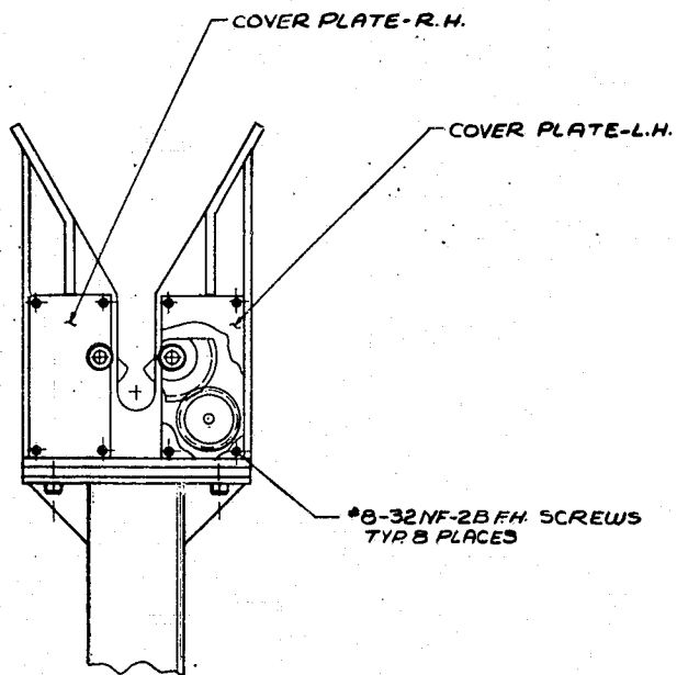
VIEW A-A 1/4 SCALE
