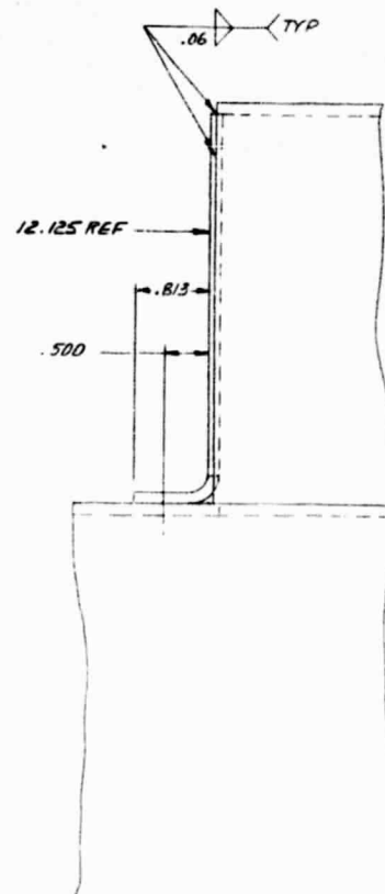
SECTION 13-13 SHOWN SECTION 13-13 OPPOSITE SCALE 1/1 SEE SECTION A-A FOR DIMENSIONS NOT SHOWN
