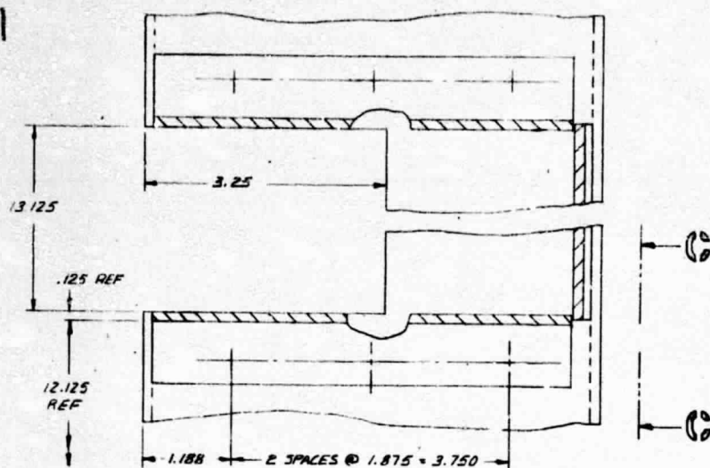
SECTION 13-13 SCALE 1/1
