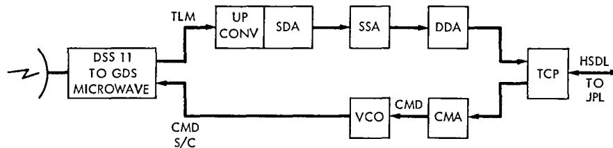
Fig. 3 DSS cross-support configuration
