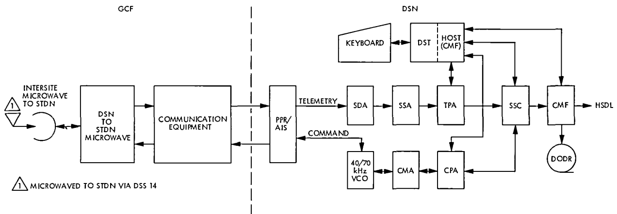
Fig. 5. DSN DSS 12 Helios cross-support configuration
