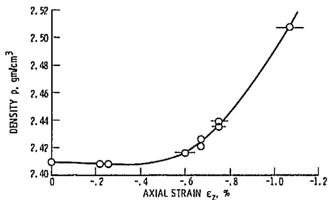
Figure 2. - Dependence of fiber density on the axial contraction produced in 203 \mu m boron on tungsten fibers by heat treatment under high vacuum.
