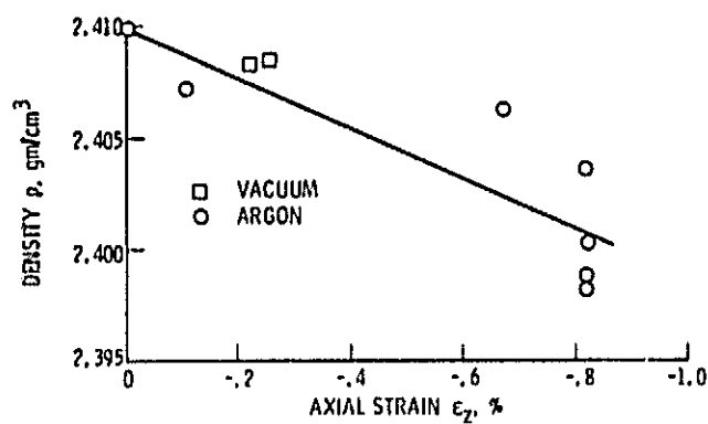
Figure 7. - Dependence of fiber density on the axial contraction produced in 203 \mu m boron on tungsten fibers by heat treatment under argon and high vacuum.
