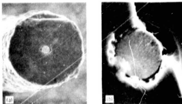
Figure 6. - Scanning electron microscope photographs of sheath voids near the cores of 203 \mu m boron on tungsten fibers after heat treatment (a) under high vacuum at 1320°C and (b) under argon at 900°C (axial contraction of 0.8%). Approximate magnification factors are (a) 300 and (b) 3000.
