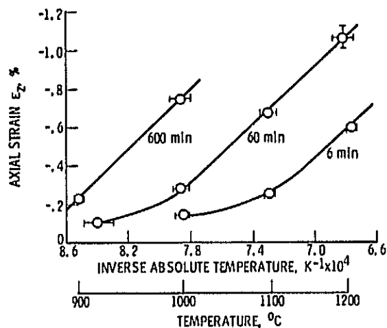
Figure 1. - Axial contraction produced in 203 \mu m boron on tungsten fibers by heat treatment under high vacuum.
