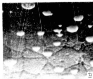
Figure 4. - Scanning electron microscope photographs of surface crystal growth on a boron fiber heat treated under vacuum for one hour at 1170°C. Approximate magnification factors are (a) 300, (b) 1000, and (c) 3000.
