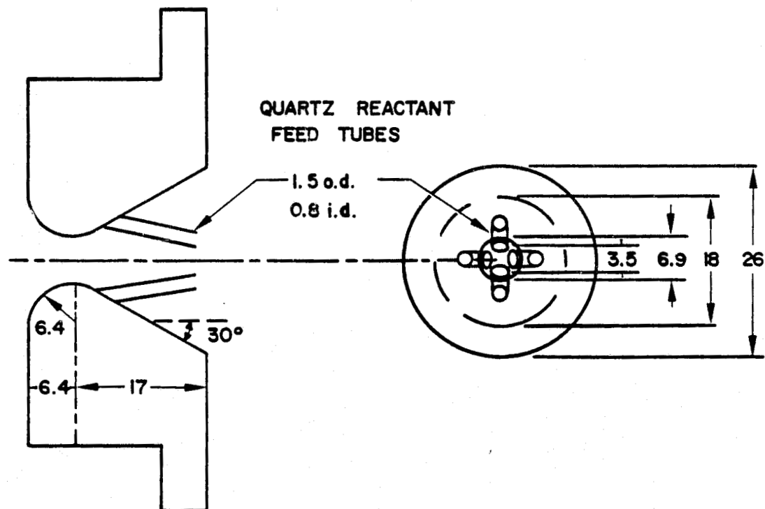
FIGURE 6 FLOWER-PETAL NOZZLE (NOZZLE NO. 5)
