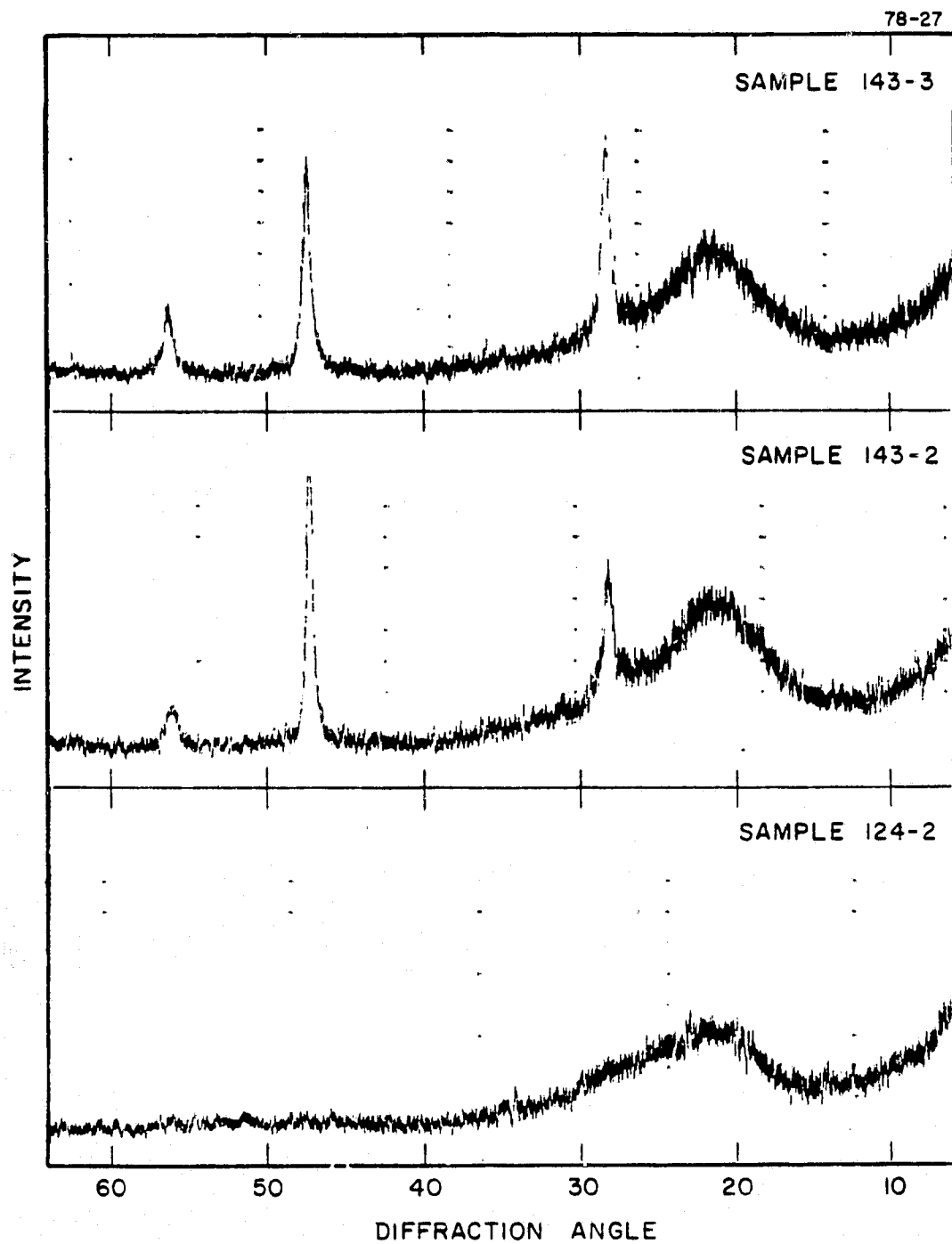
FIGURE 35 X-RAY DIFFRACTION PATTERNS FOR SILICON FILMS
