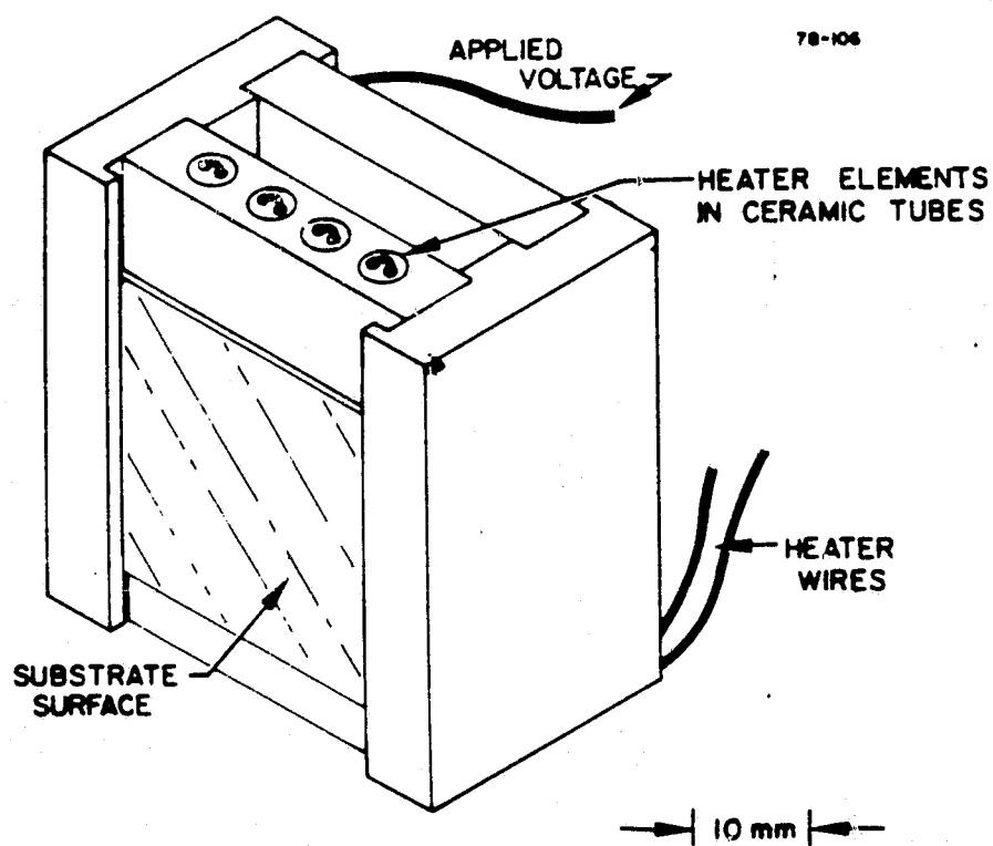
FIGURE 40 SUBSTRATE HOLDER
