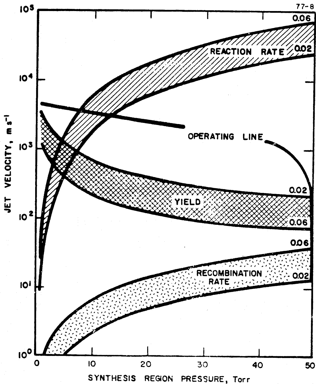
FIGURE 27 LIMITING PERFORMANCE CURVES
