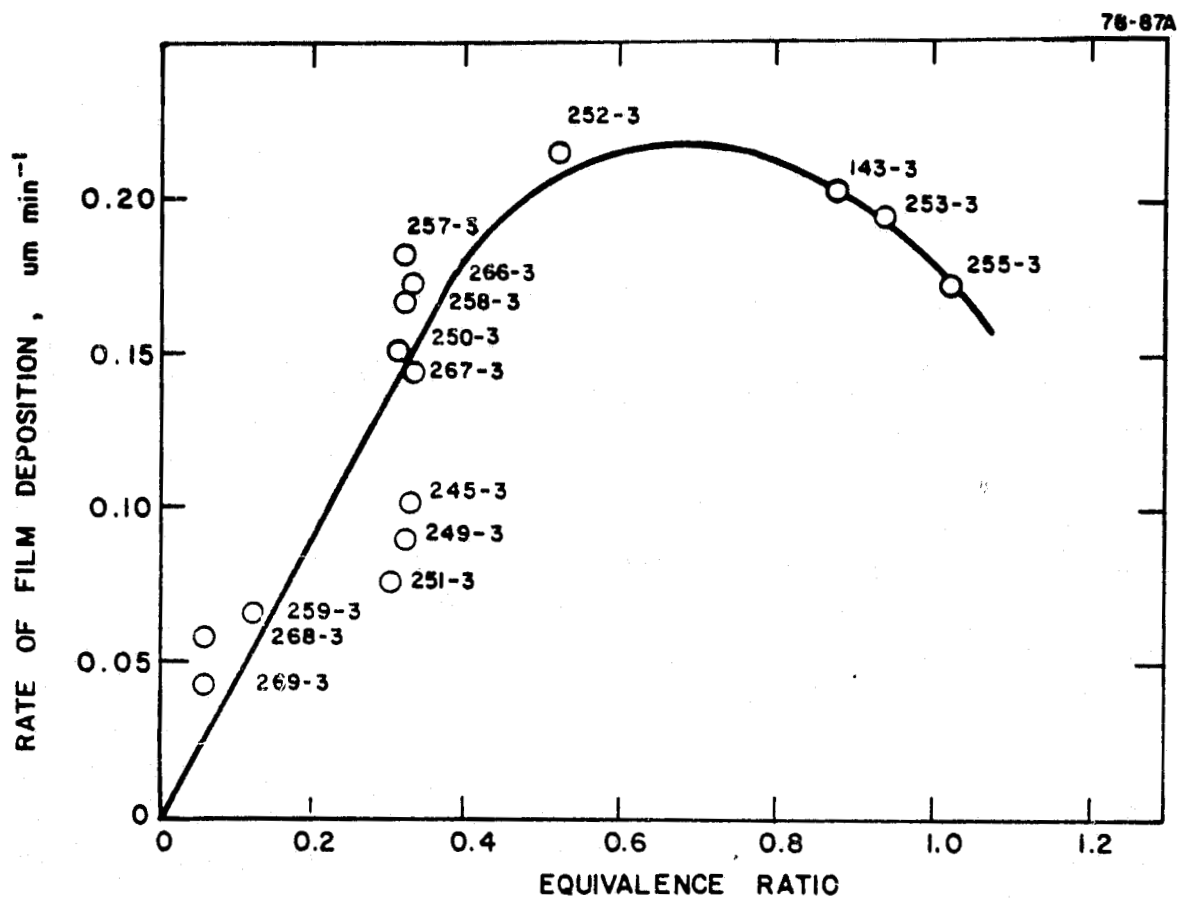
FIGURE 38 RATE OF FILM DEPOSITION FROM SiCl 4 Run numbers indicated above points.
