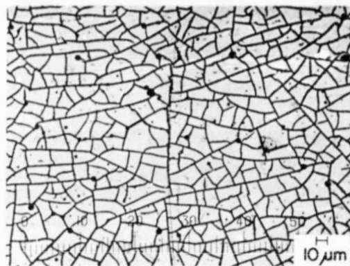
FIGURE 34 EFFECT OF EXPOSURE TIME ON SILICON FILMS DEPOSITED FROM \text{SiCl}_4
