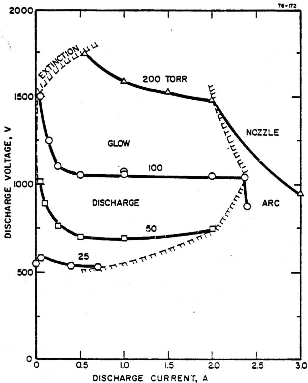
FIGURE 14 DISCHARGE STABILITY IN HYDROGEN
