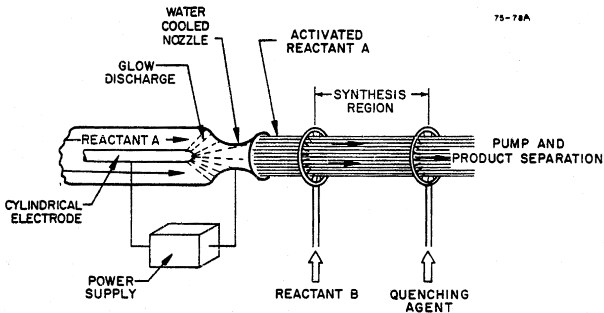
FIGURE 1 NON-EQUILIBRIUM PLASMA JET FOR CHEMICAL SYNTHESIS
