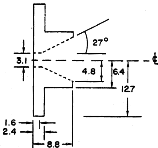
FIGURE 5 NOZZLE ELECTRODES NO. 1, 2, AND 3 FOR NON-EQUILIBRIUM PLASMA JET GENERATION OF HYDROGEN ATOMS
