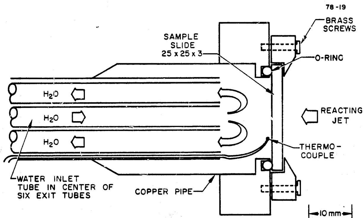
FIGURE 37 WATER-COOLED SAMPLE HOLDER Dimensions in mm.
