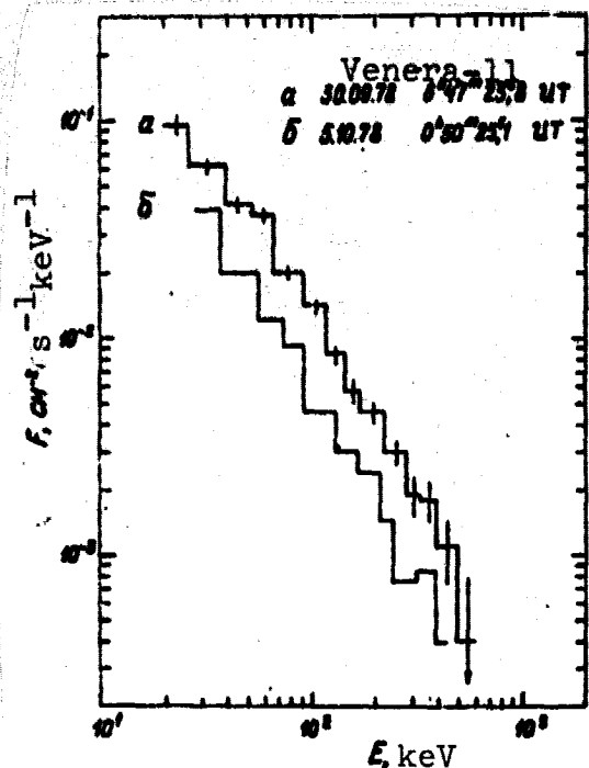
Figure 12. Energy spectra of 2 gamma-bursts close in shape
