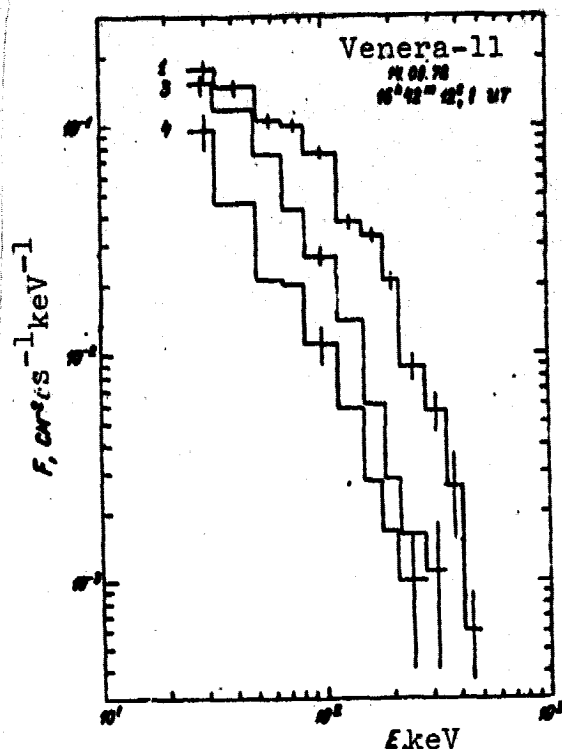
Figure 13. An example of observation of the evolution of the radiation spectrum during a burst. Spectra are presented measured in the 1st, 3rd and 4th 4-second intervals after T_0 .
