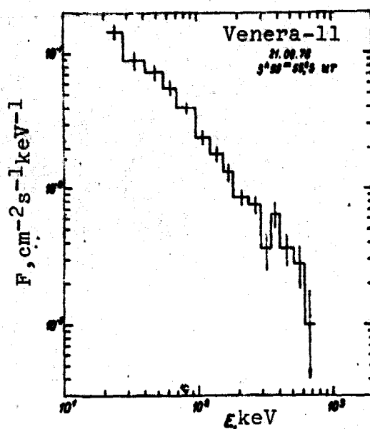
Figure 15. A spectrum of a gamma-burst 9/21/78 shows a similarity with the spectra of figure 14.
