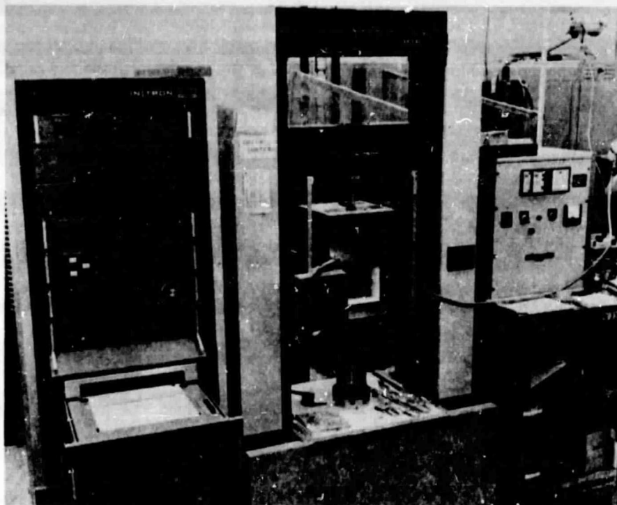
Figure 21 Room Temperature and Hot MOR Test Apparatus at Ford
