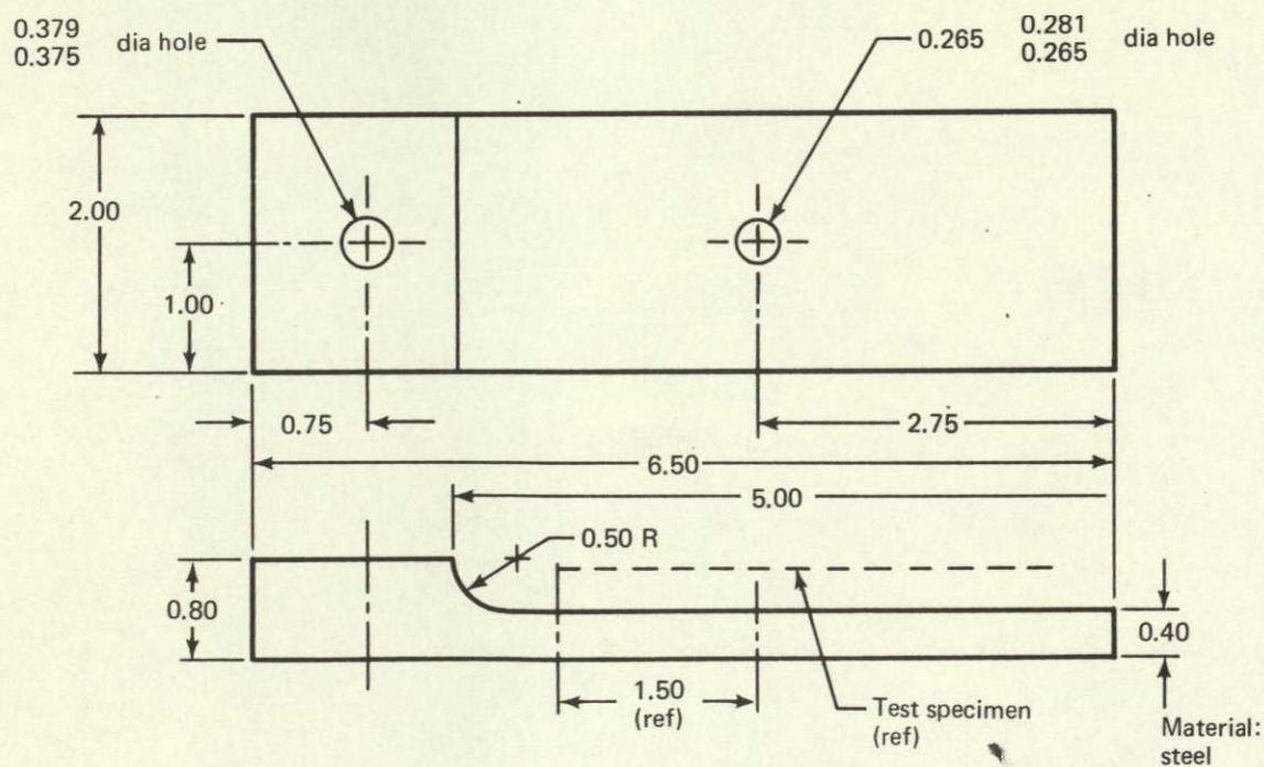
Insert Shear Test Fixture
