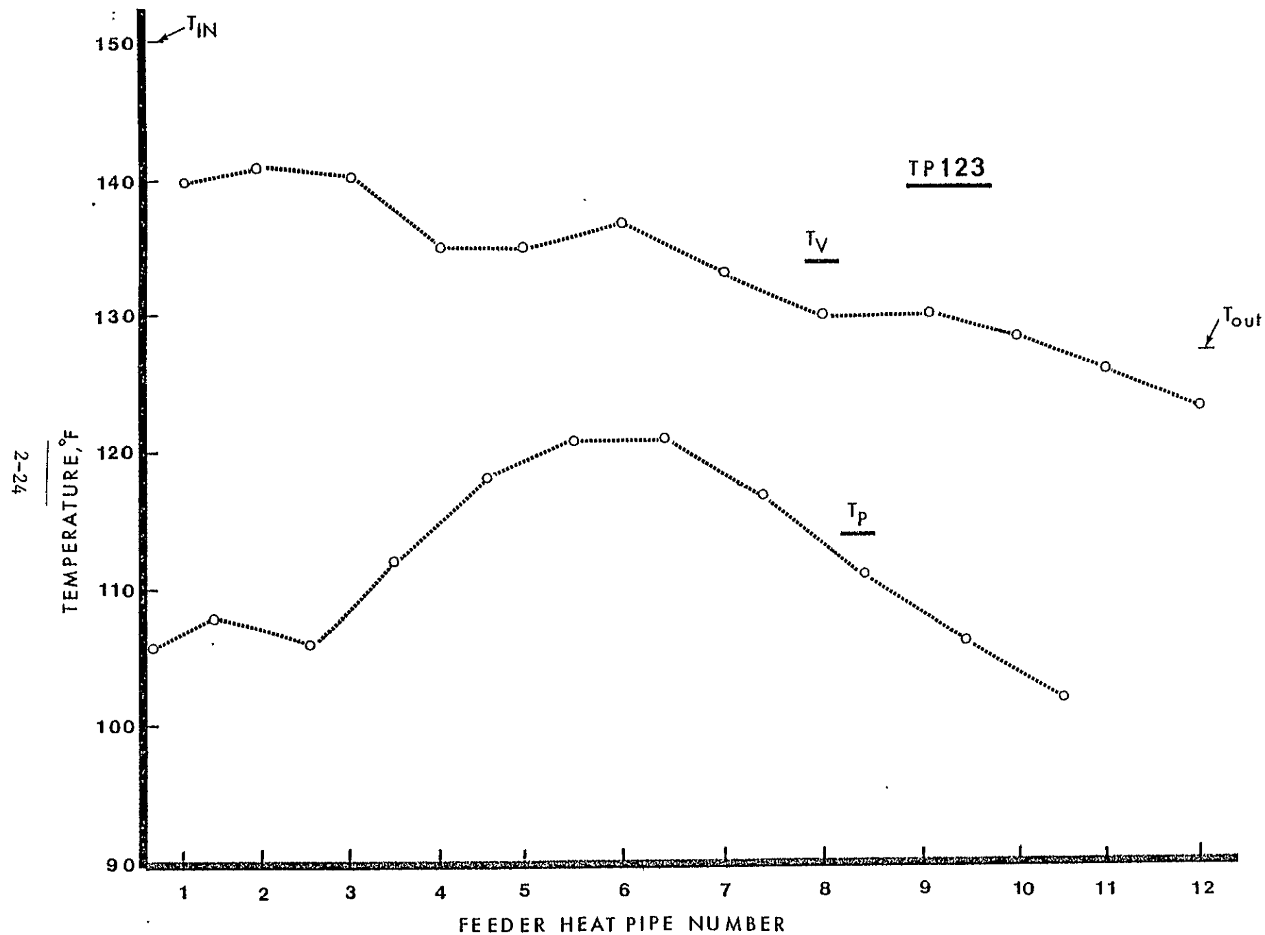
Figure 2.14. Panel temperature distribution for TP 123.
