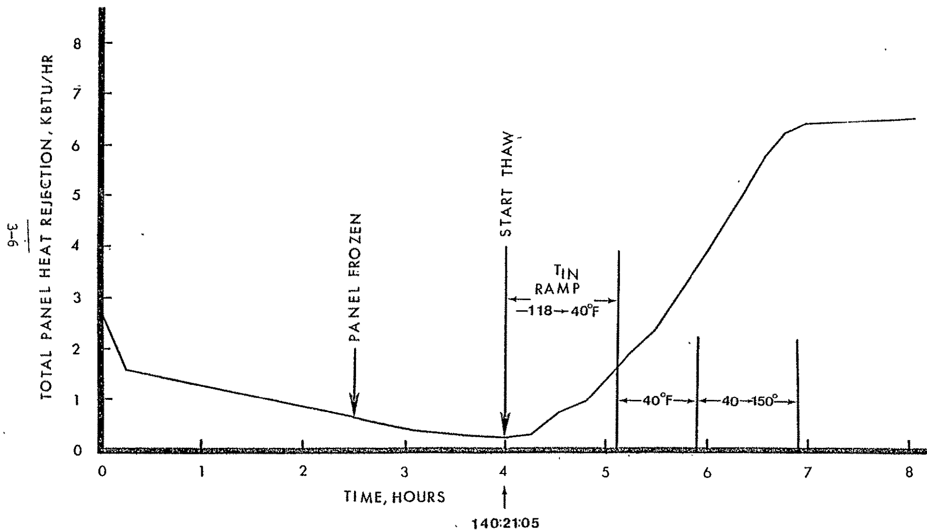
Figure 3.3b. Radiator freeze-thaw performance; TP 209B.
