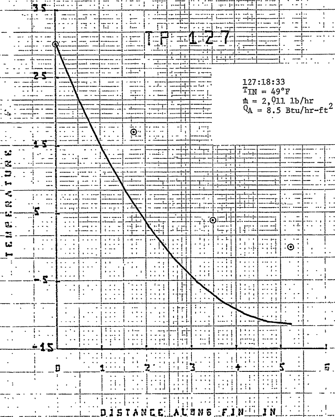
Figure 2.28. Fin temperatures for left fin of feeder No. 7; TP 127.
