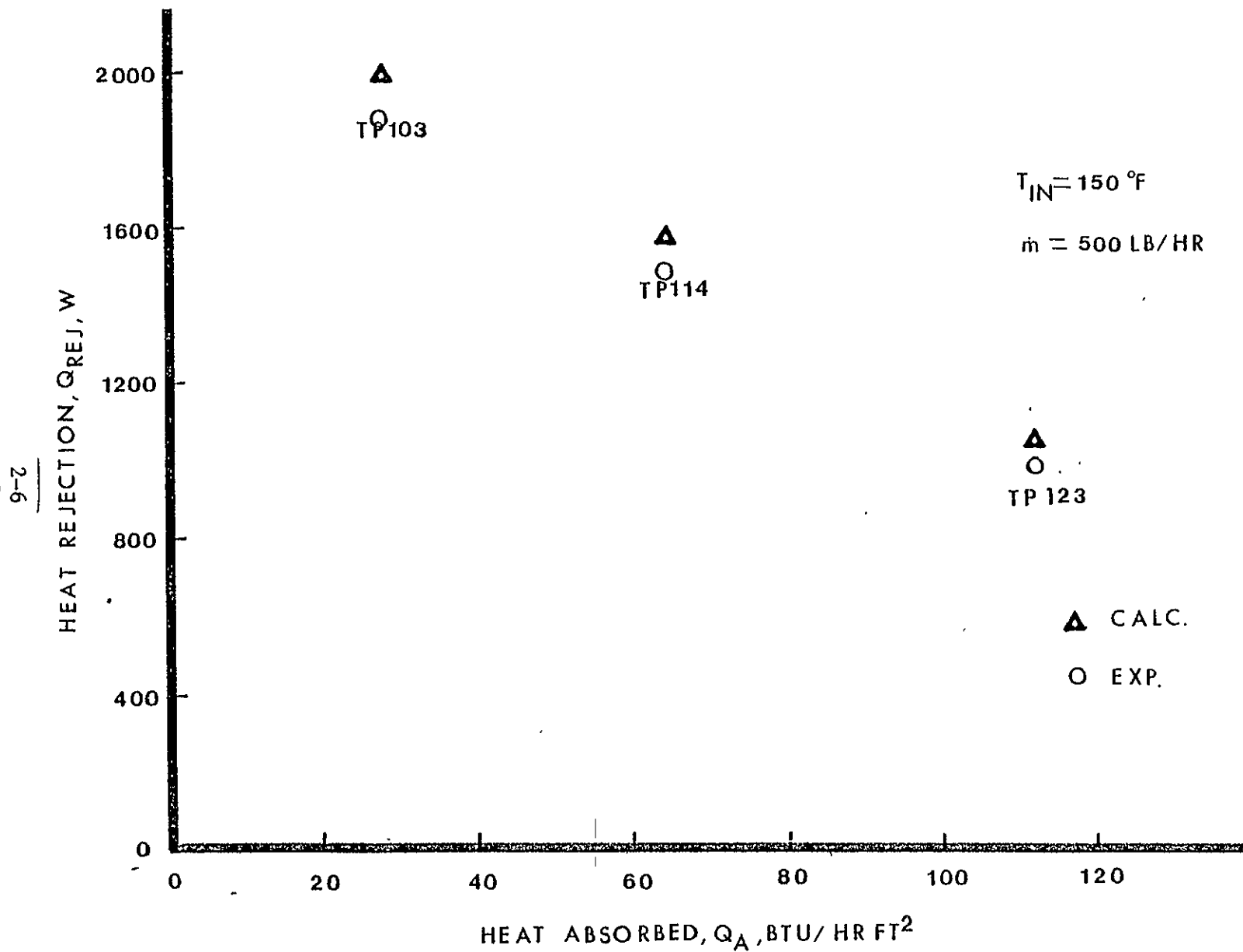
Figure 2.3 The effect of Q_A on Q_{REJ} : \dot{m} = 500\text{ LB/HR} .
