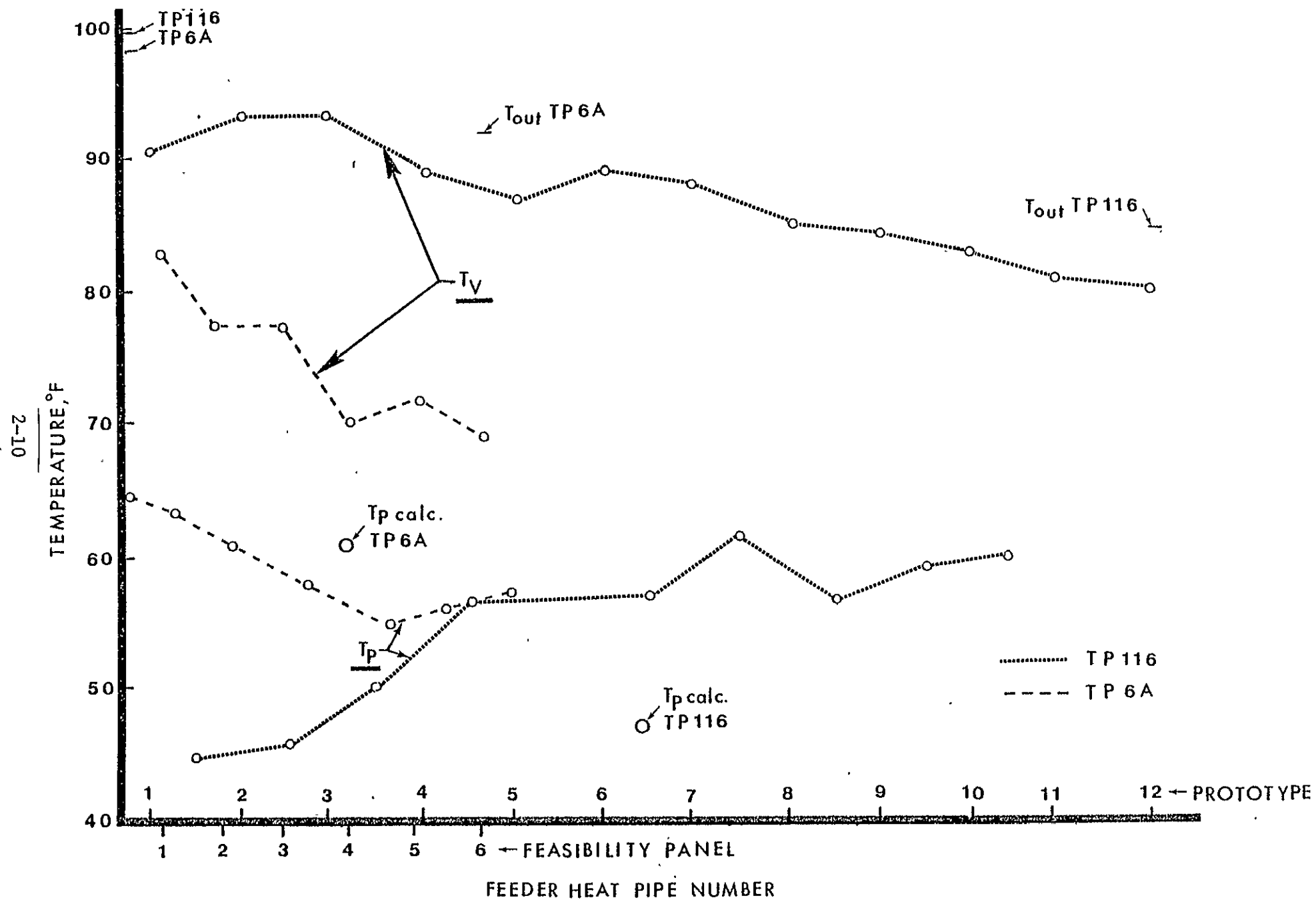
Figure 2.6 Temperature comparisons of TPs 116 and 6A.
