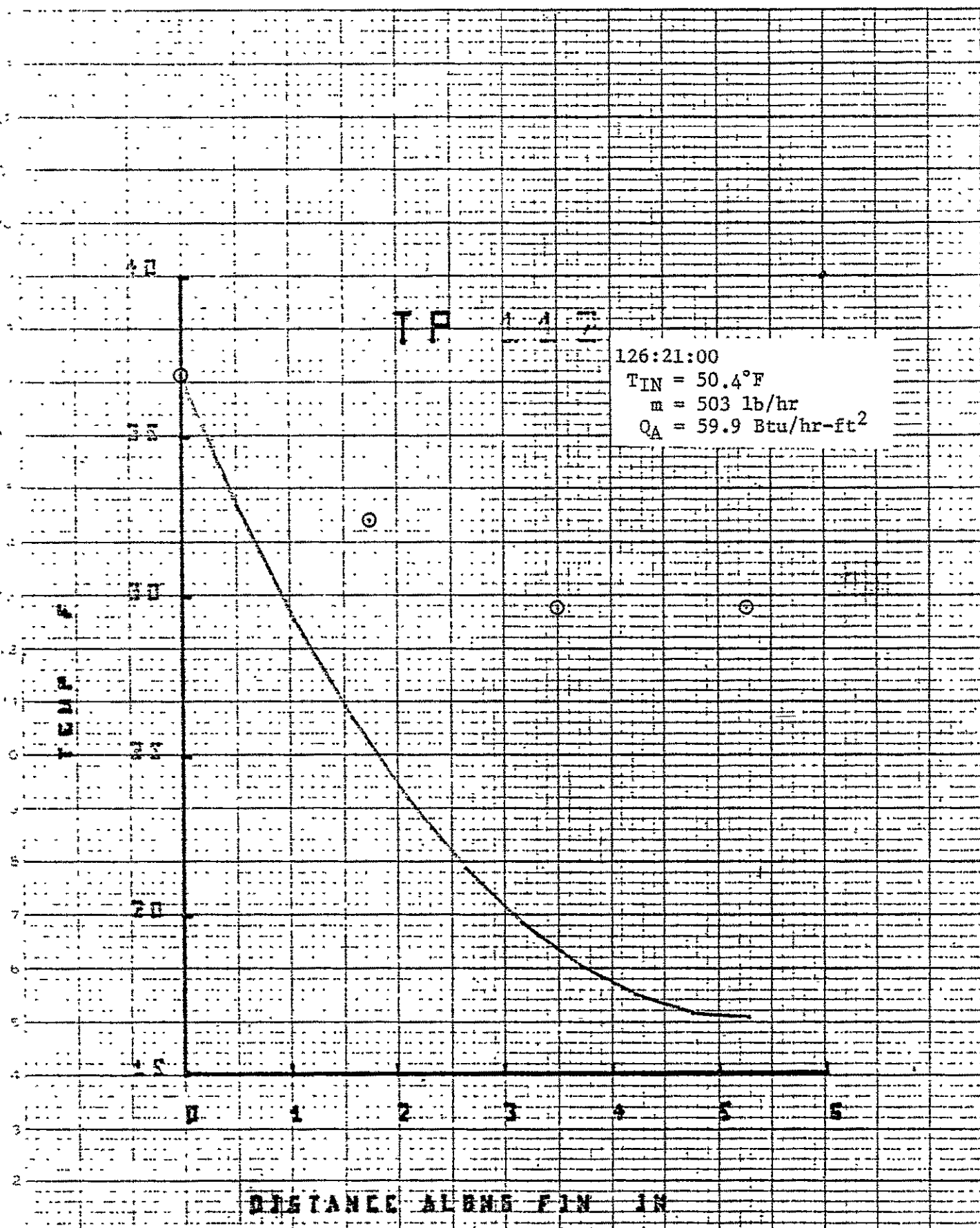
Figure 2.20. Fin temperatures for left fin of feeder No. 7; TP 112.
