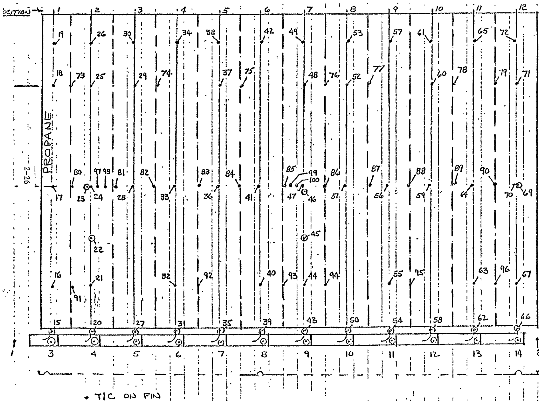
Figure 2.16. THERMAL MAP INSTRUMENTATION
