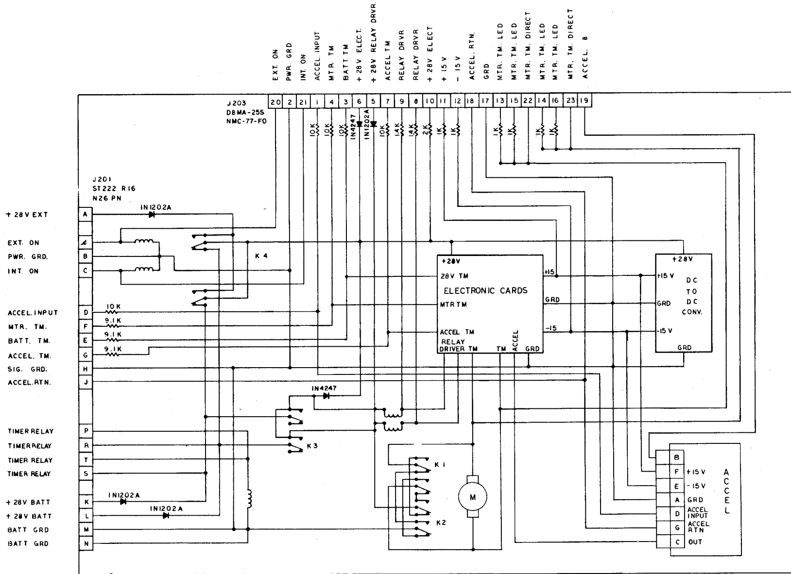
Figure 4. Wiring Diagram of the LAND System
