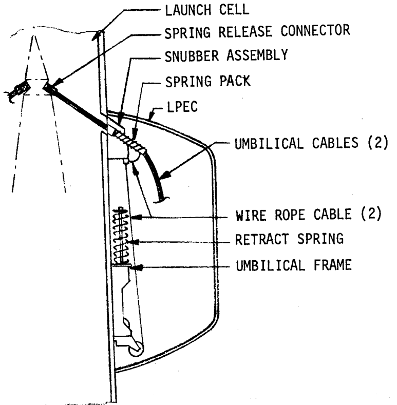
Figure 2. SPRINT II Umbilical Retract Mechanism
