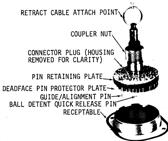
Figure 5. Flush Umbilical Connector Assembly
