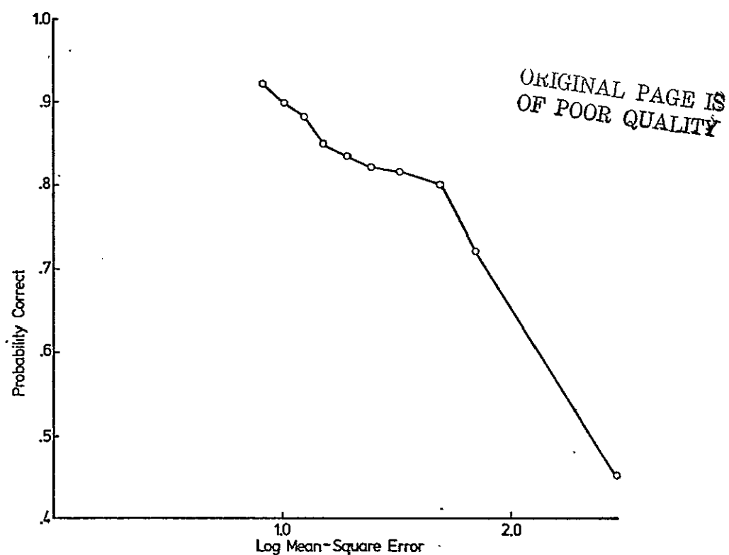
Figure 2C1-7. Probability of correct classification vs. representation error for the optimal basis functions.
