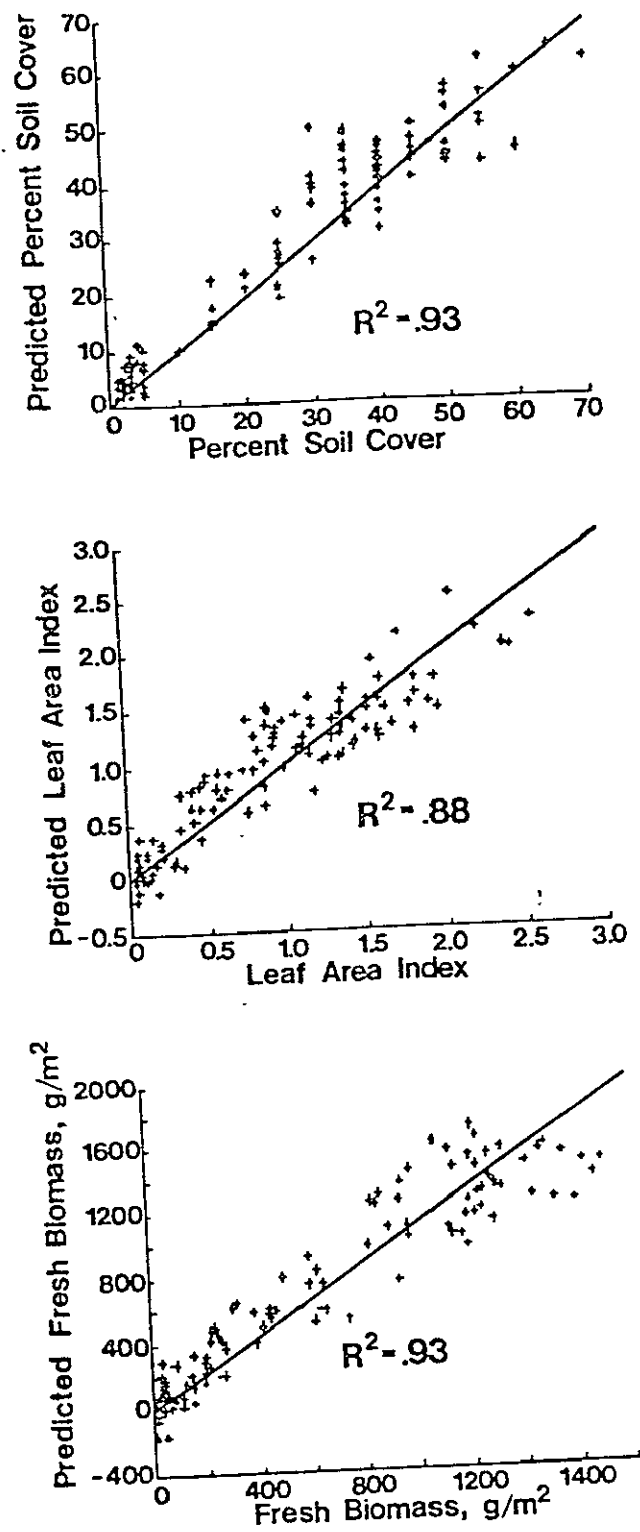
Figure 1A-3. Comparison of measured and predicted percent soil cover, leaf area index, and fresh biomass of spring wheat canopies.
