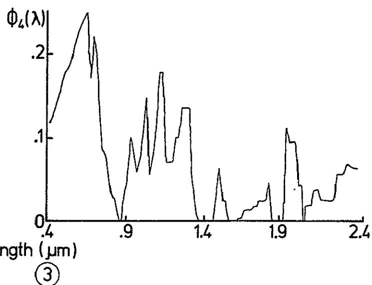
Figure 2C1-4. The magnitude of the first four optimal spectral basis functions for a data set from the Northern vs. Great Plains in early season (May). The data set contained spectra from wheat, fallow and pasture classes. A weighting function set to zero in the water absorption bands near 1.4 and 1.9 \mu\text{m} was used. The encircled number shows the order of selection by a feature selection algorithm for discriminating between the three classes.
