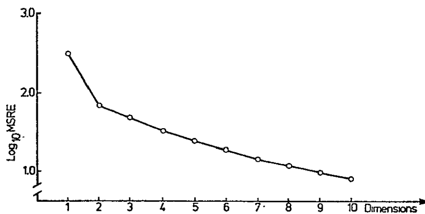
Figure 2C1-6. Log mean square representation error vs. the number of dimensions.
