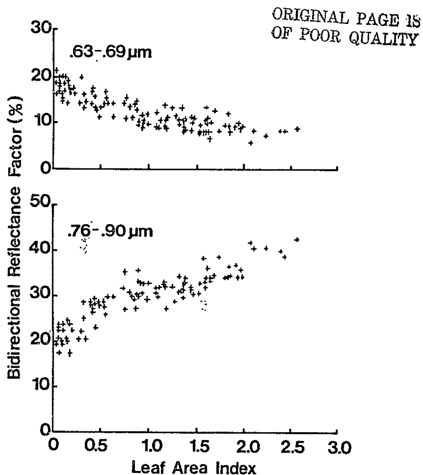
Figure 1A-2 Relationship of leaf area index to reflectances in the chlorophyll absorption (0.63-0.69 \mu\text{m} ) and near infrared (0.76-0.90 \mu\text{m} ) regions. Measurements for seedling through flowering stages of maturity are included for 16 treatments representing different levels of soil moisture availability, planting dates, nitrogen fertilization, and cultivar.
