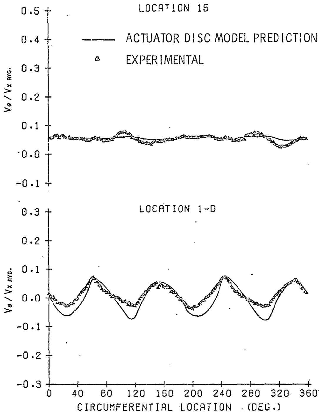
Figure 35. Sample V_0 distribution data and the actuator disc model predictions for a four-cycle sinusoidal distortion.
