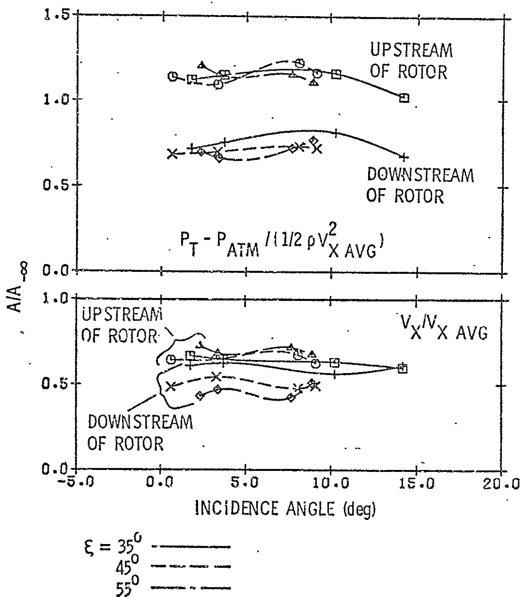
Figure 46. Amplitude ratio versus incidence for a 90^\circ square distortion.
