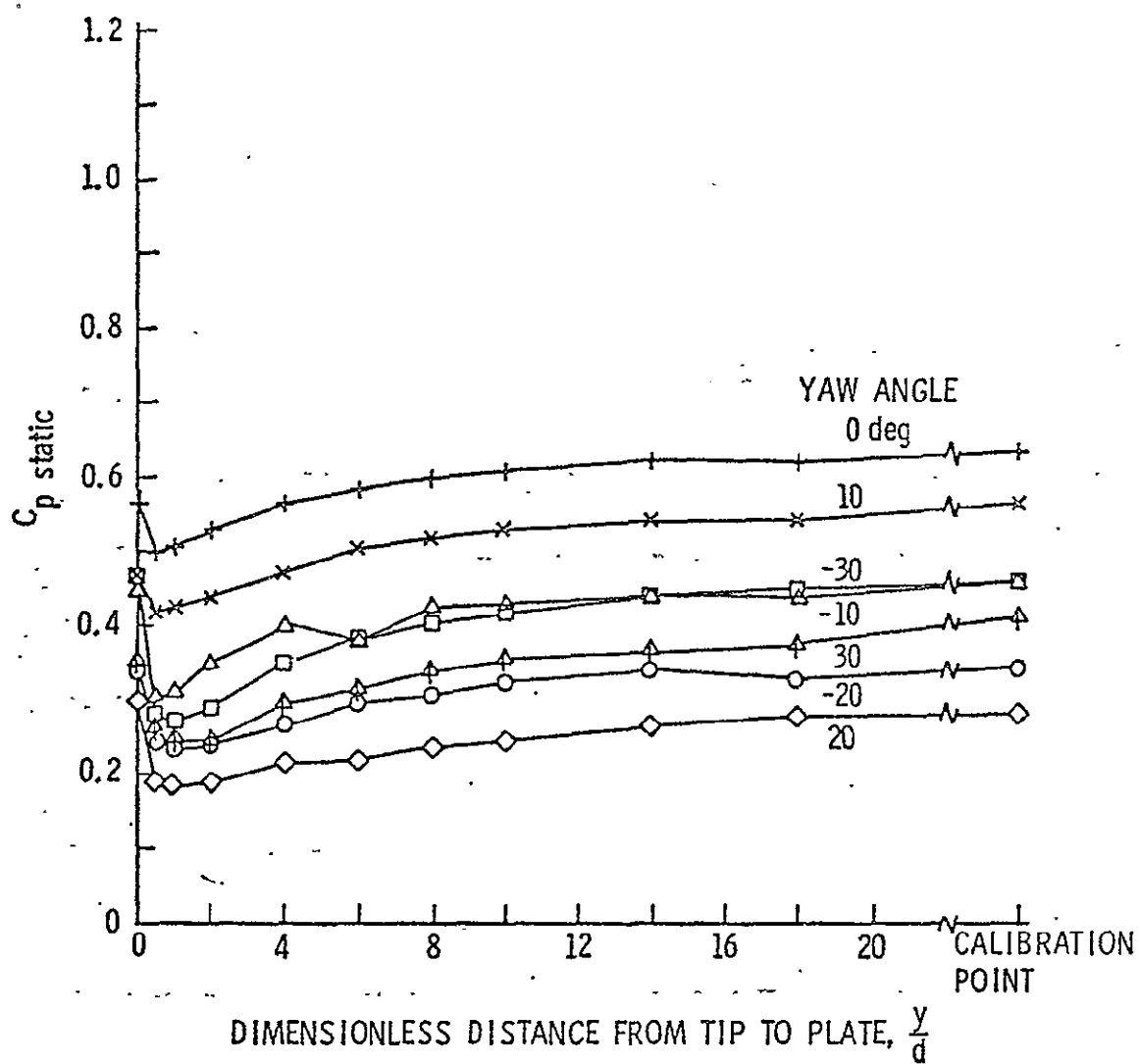
Figure A.15. C_{p \text{ static}} versus the dimensionless distance from the probe tip to the plate for Probe 1. The probe is approaching the plate.
