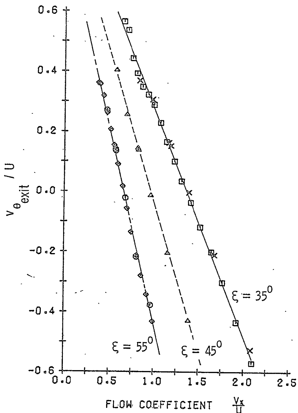
Figure 18. A comparison of v_{\theta \text{ exit}} / U versus v_x / U obtained experimentally and the straight line representation of the data used in the actuator disc analysis.
