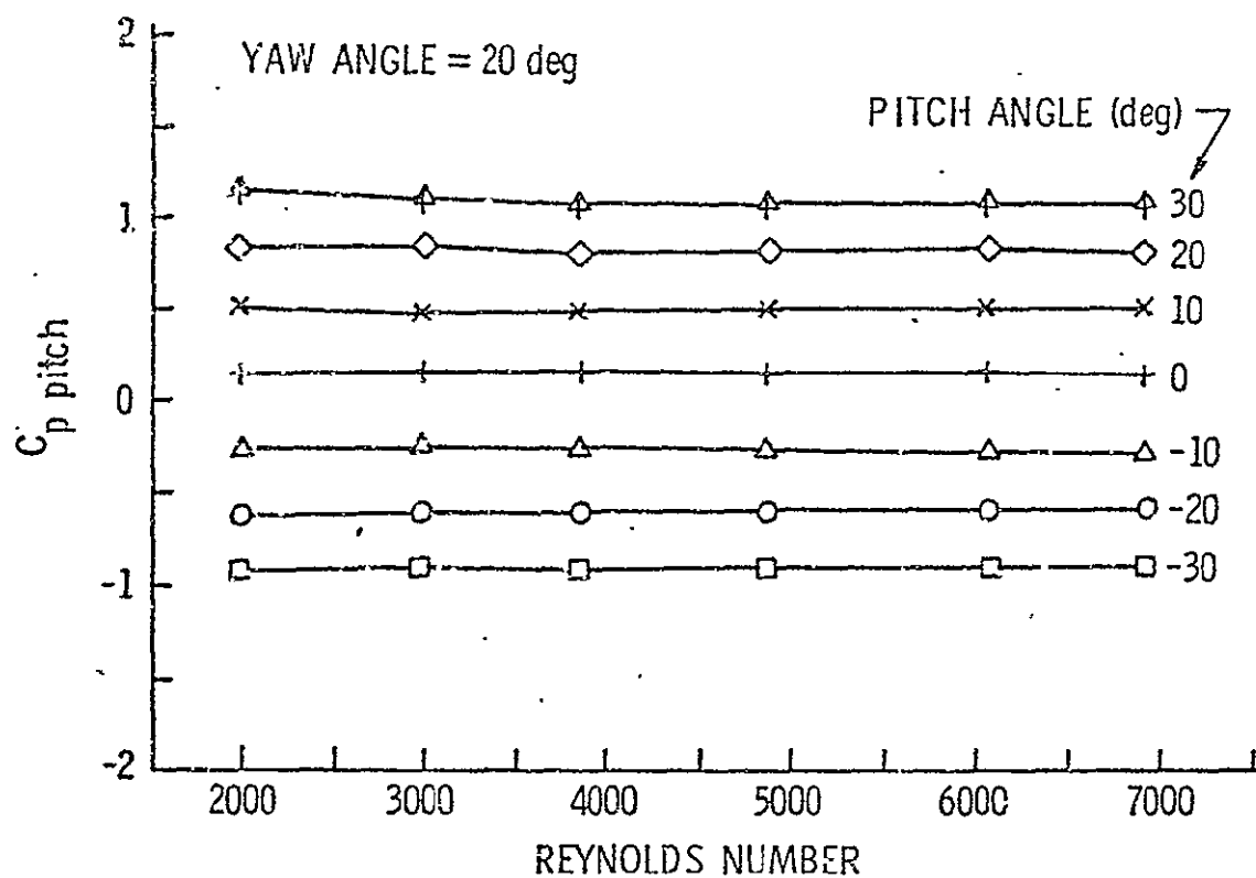
Figure A.9. C_{p \text{ pitch}} versus Reynolds Number for Probe 1 at a 20° yaw angle.
