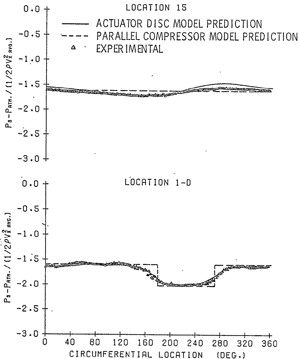
Figure 31. Sample static pressure distribution data for a 90° square distortion and the distributions predicted by the parallel compressor and actuator disc models.
