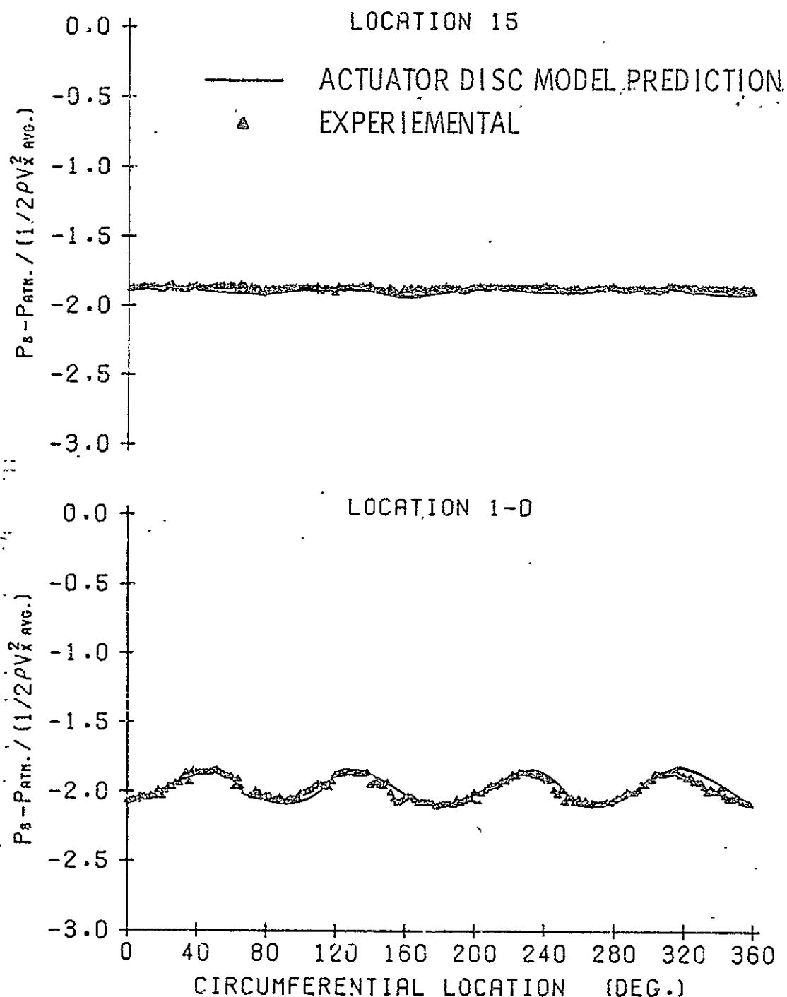
Figure 32. Sample static pressure distribution data for a four-cycle sinusoidal distortion and the distributions predicted by the actuator disc model.
