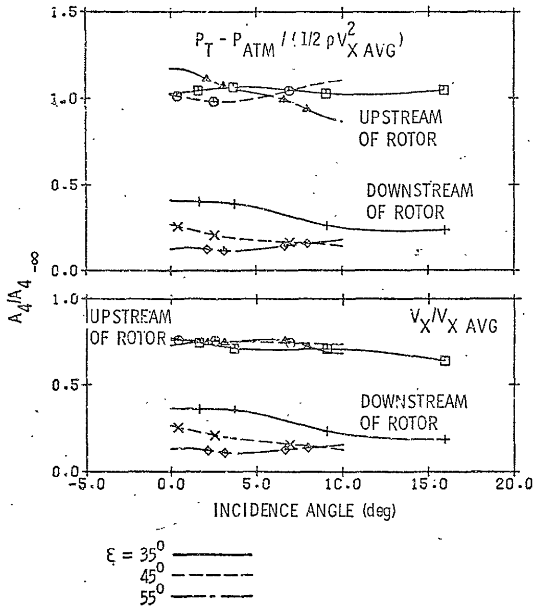
Figure 42. Measured axial velocity and total pressure distortion attenuation versus incidence angle for a four-cycle sinusoidal distortion.
