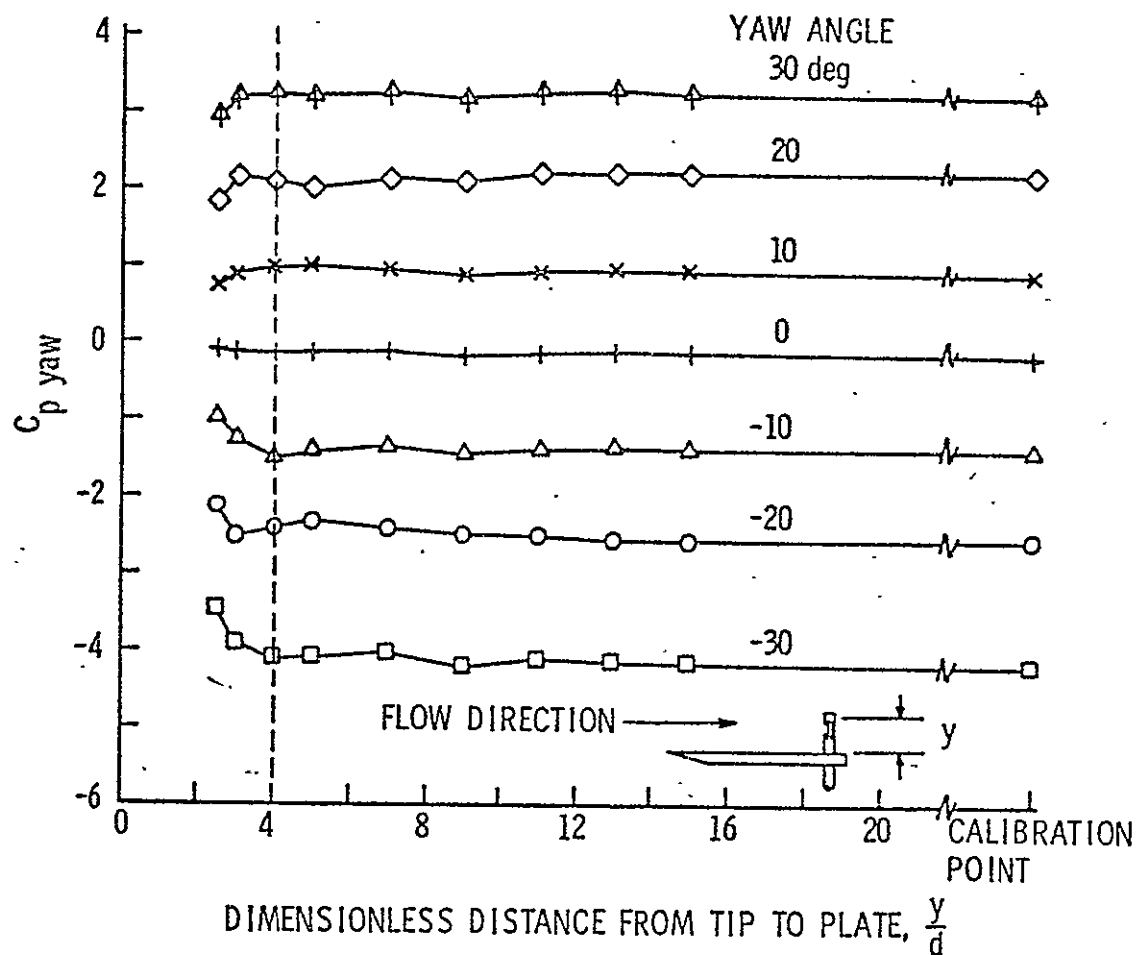
Figure A.16. C_{p \text{ yaw}} versus the dimensionless distance from the probe tip to the plate for Probe 1. The probe is drawn through a hole in the plate as shown by the accompanying sketch.
