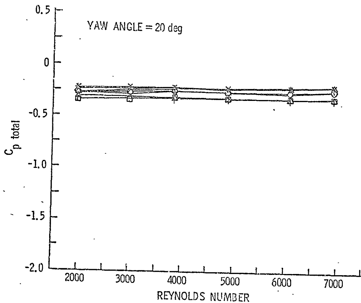
Figure A.11. C_{p \text{ total}} versus Reynolds Number for Probe 1 at a 20° yaw angle.
