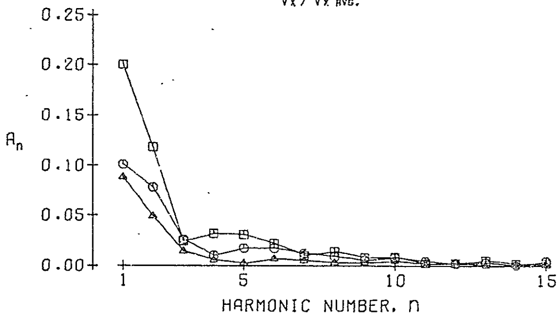
Figure 41. Dimensionless total pressure and axial velocity harmonic amplitudes as a function of the harmonic number, n , for a 90° square distortion.
