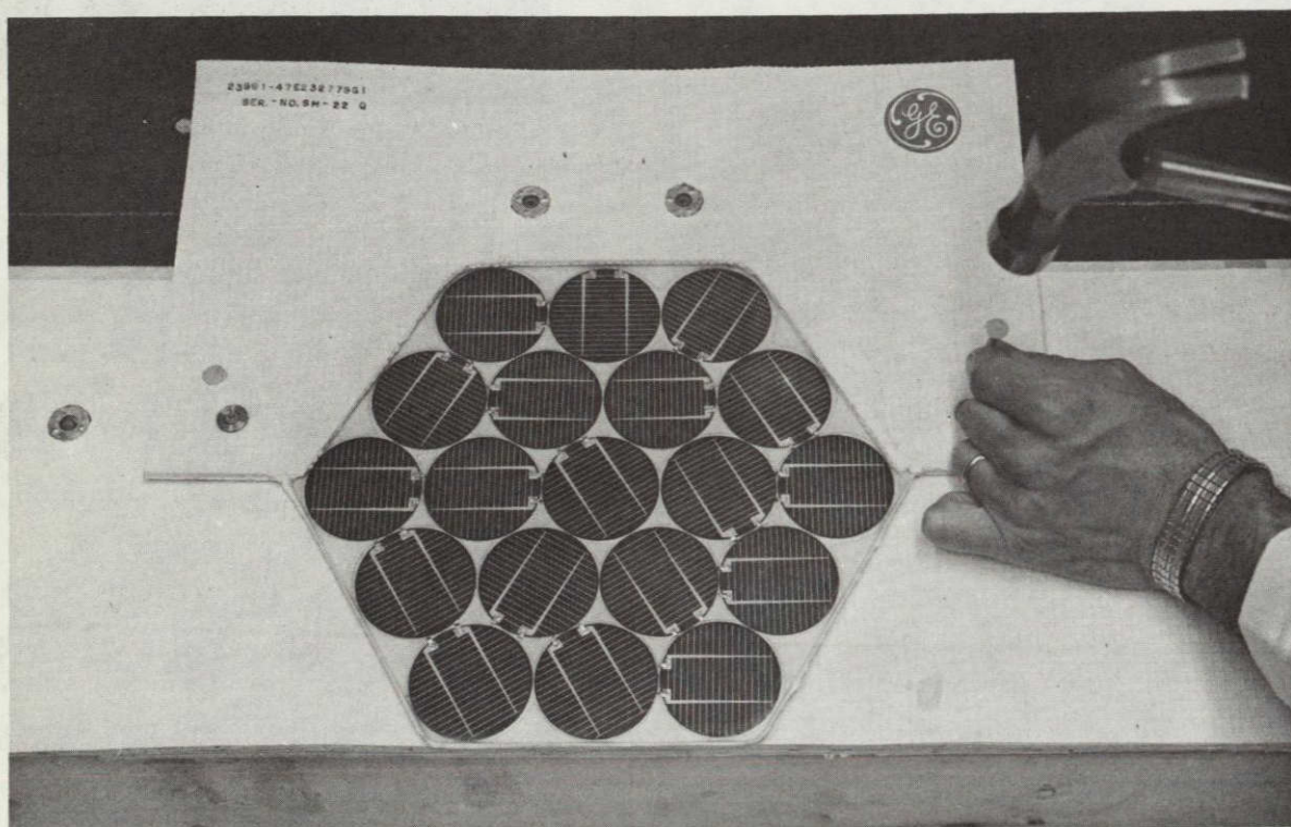
Figure 3-14. Nailing of Shingle Module to Roof Sheathing
