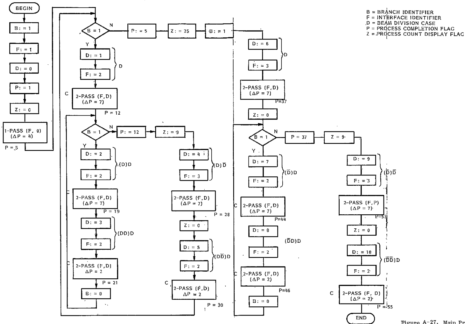
Figure A-27. Main Program Logic Flow Diagram
