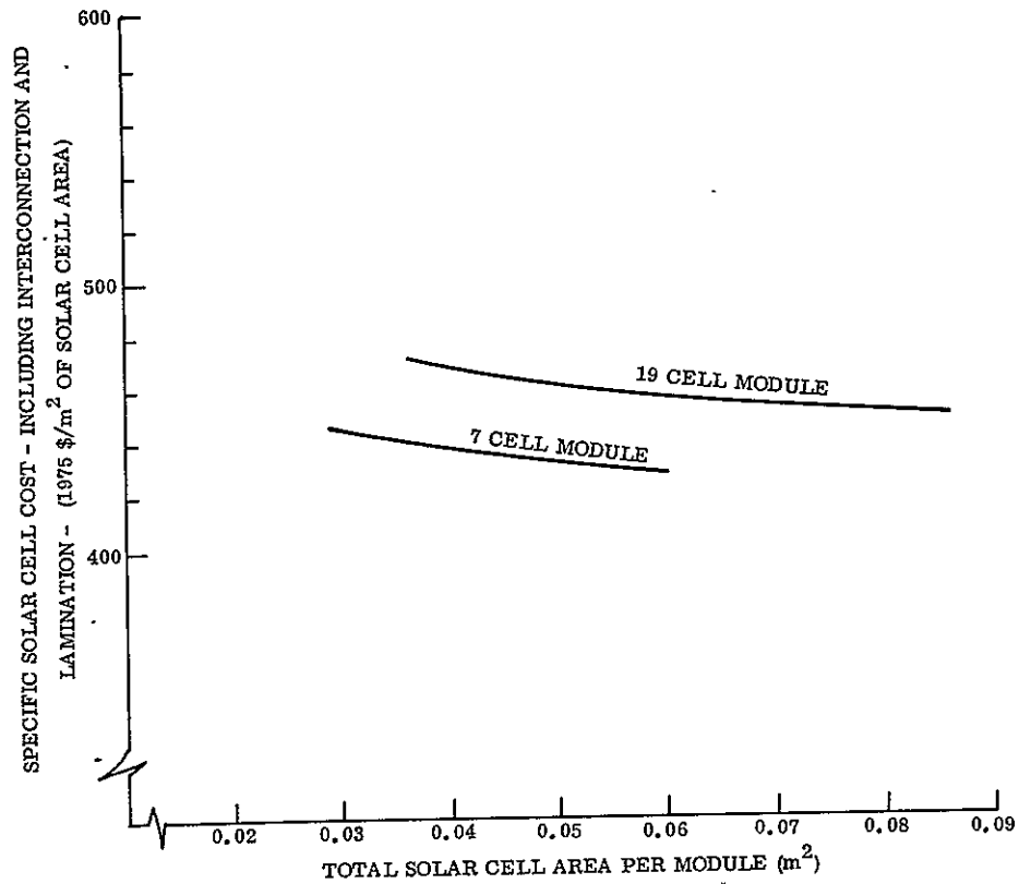
Figure A-38. Specific Solar Cell Cost
