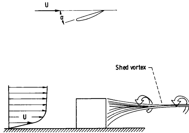
Figure 1. - The vortex generator.
