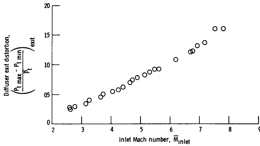
Figure 48 - Diffuser exit total pressure distortion with configuration II vortex generators installed
