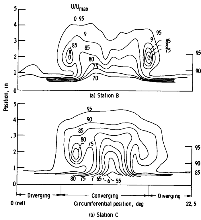
Figure 62 - Rake velocity contours for configuration I vortex generators installed, \bar{M}_{inlet} = 0.29
