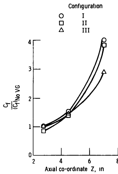
Figure 83 - Average skin friction coefficient variation
