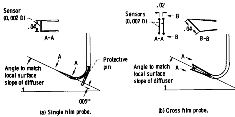
(a) Single film probe. (b) Cross film probe. Figure 30. - Hot film anemometry probe details (all dimensions shown are in in.).
