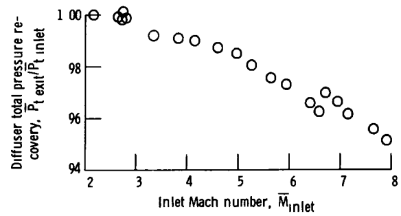
Figure 46 - Diffuser total pressure recovery with configuration III vortex generators installed
