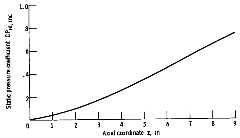
Figure 15 - Theoretical incompressible static pressure coefficient variation
