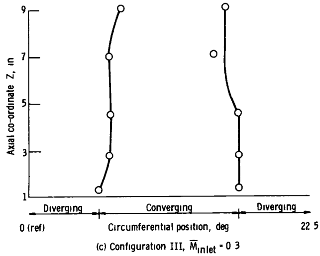
Figure 67 - Vortex axial location.
