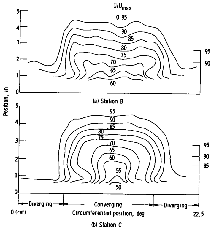
Figure 64 - Rake velocity contours for configuration I vortex generators installed, \bar{M}_{inlet} = 0.81
