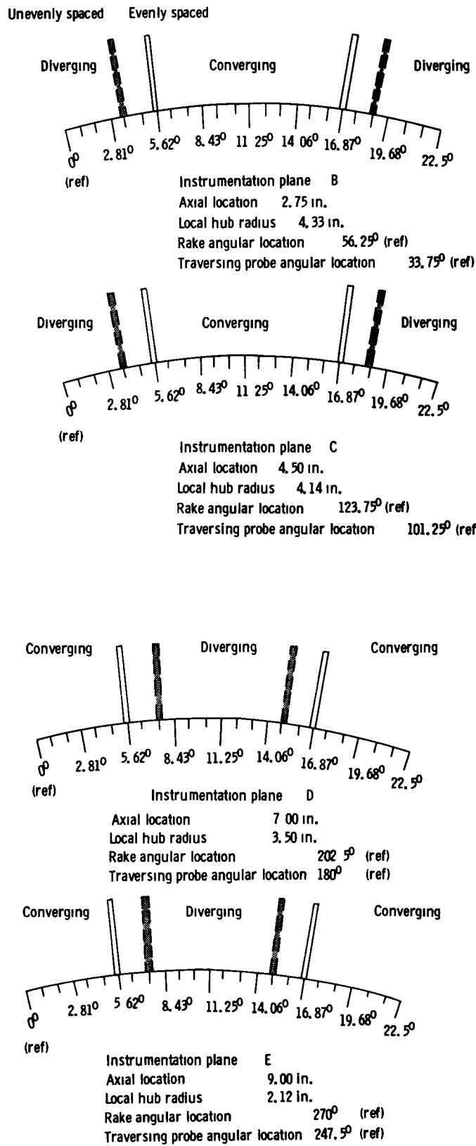
Figure 31. - Instrumentation locations relative to vortex generators.
