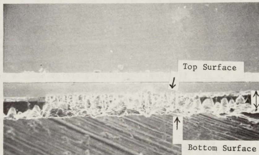
Fig. 28 2009 - 6LS Laser Scribed from back. Note total penetration after laser scribe dwell. Length of scale bar: 100 \mu\text{m} .
