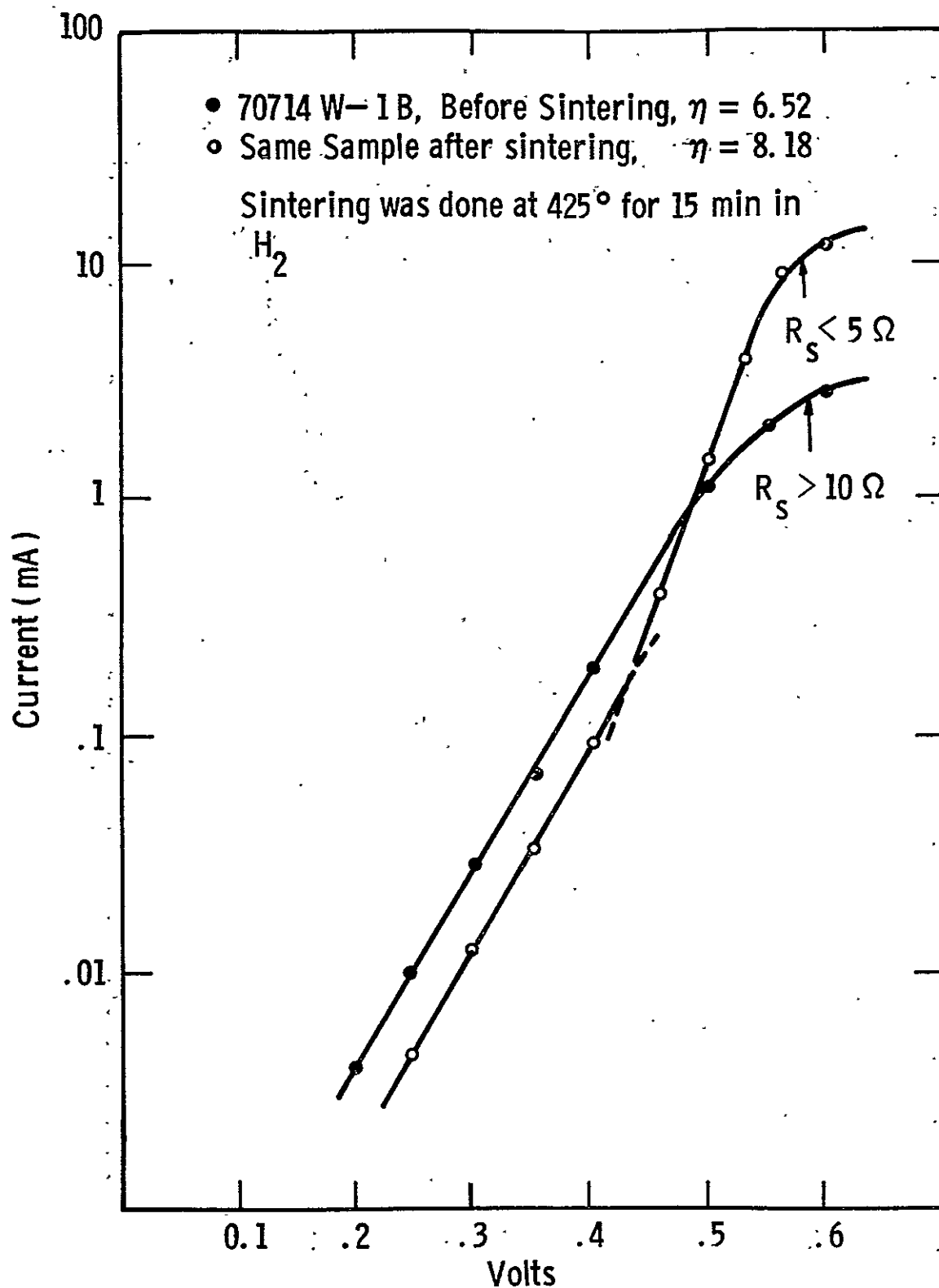
Fig. 30 Measured dark I-V curves for the sample 70714W-13: • Before Sintering, • After Sintering at 425^\circ\text{C} .
