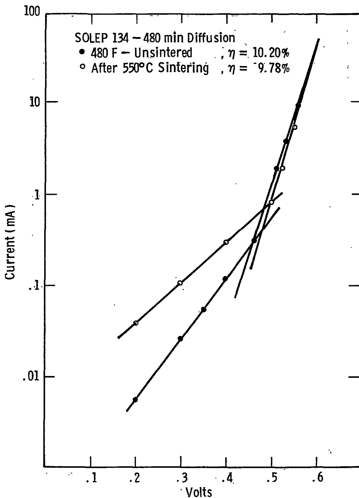
Fig. 32 Transformed Dark I-V Curves for the Sample SOLEP 134-480F: ● Before, ● After Sintering at 550°C.
