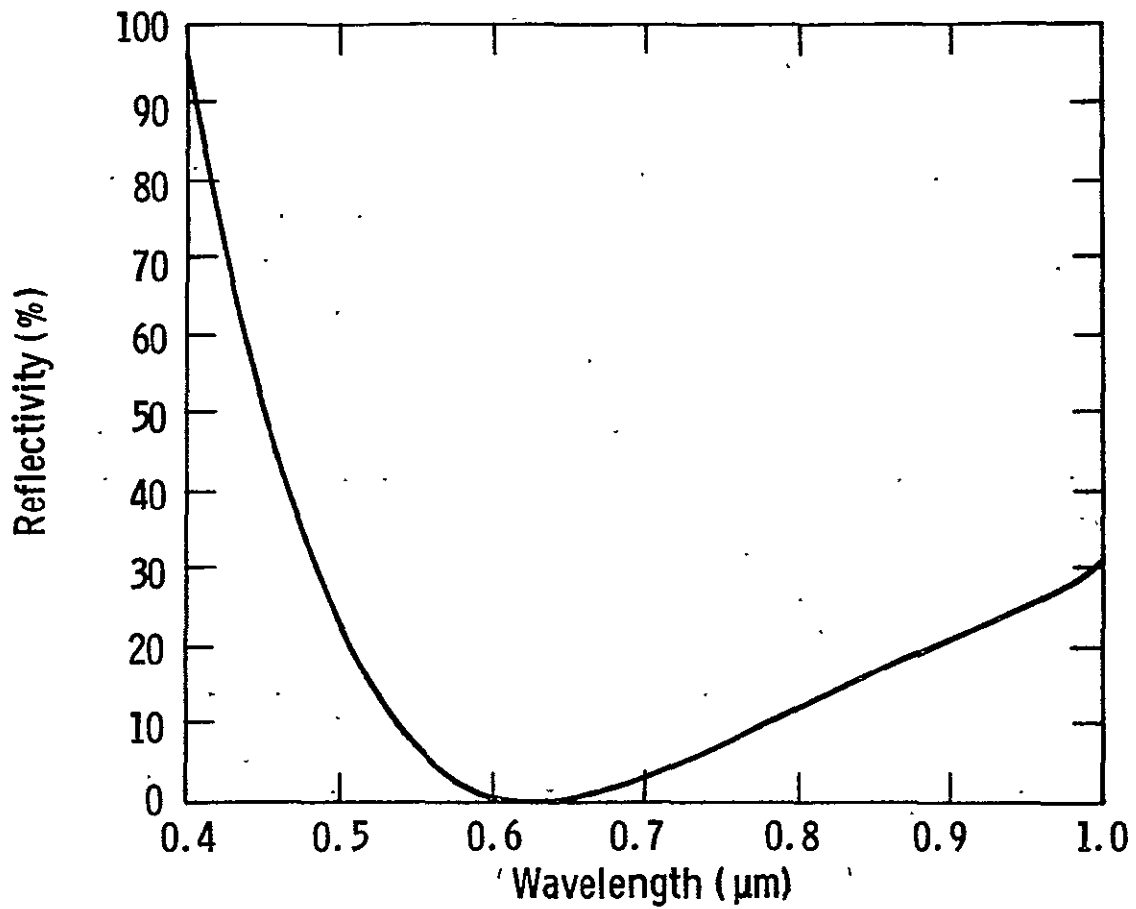
Fig. 6 Spectral reflectivity of a AR coating on a web silicon solar cell (composition 88% \text{TiO}_2 - 12% \text{SiO}_2 , heat treated at 450°C)..
