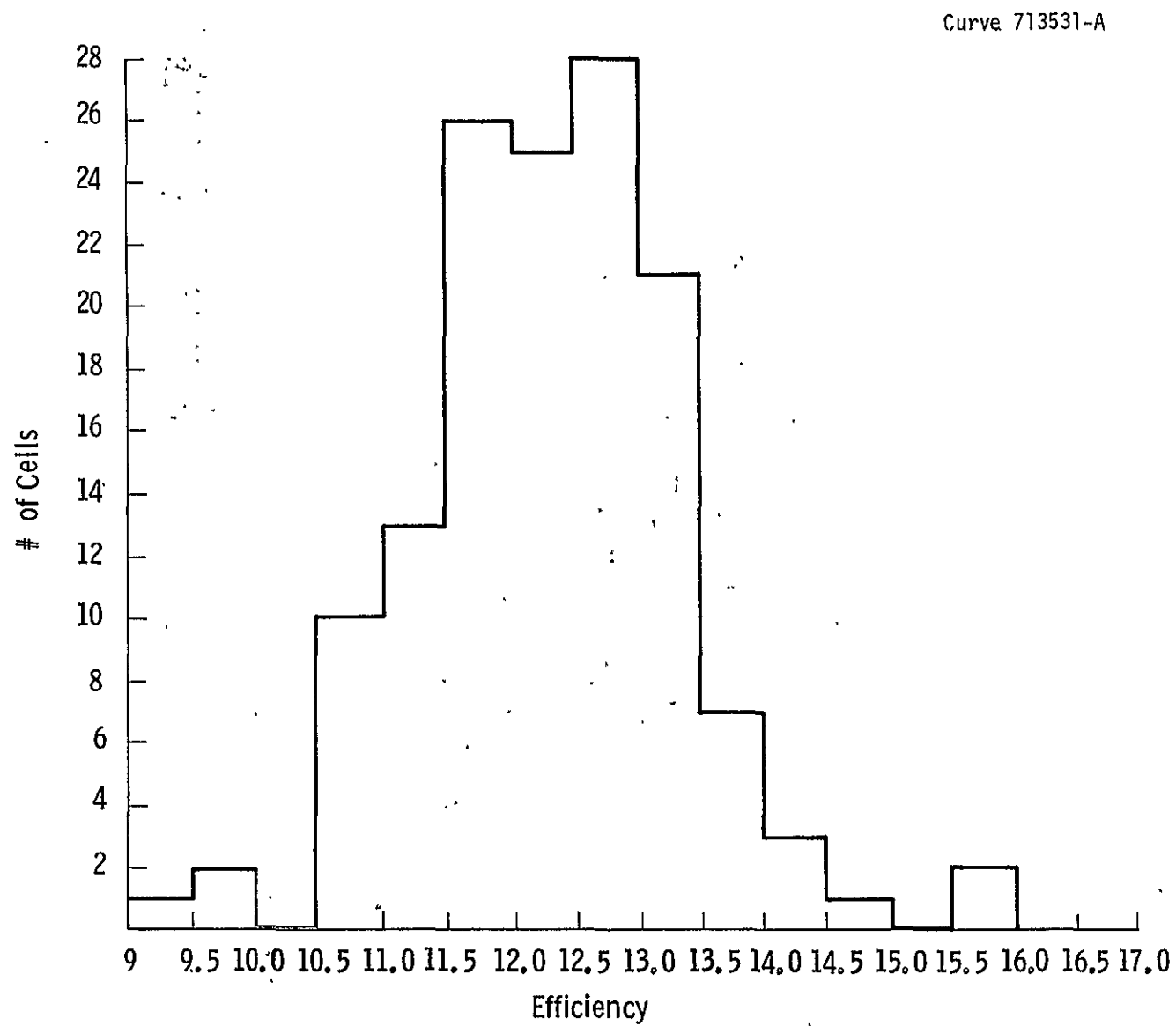
Fig. 20 — Cells fabricated by Array process AR coated
