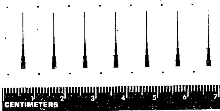
Fig. 17 Contact print of the grid electrode mask for a 2.0 cm x 7.0 cm dendritic web silicon cell.
