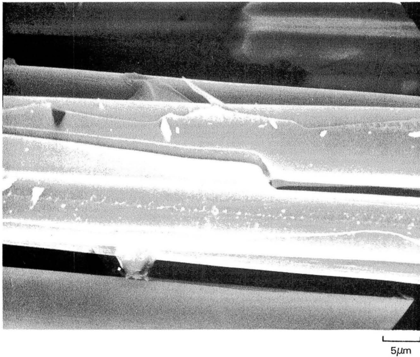
Fig. 40 SEM of Silica-Like Coated HTS From Continuous Coating Process, (Run SC 7)
