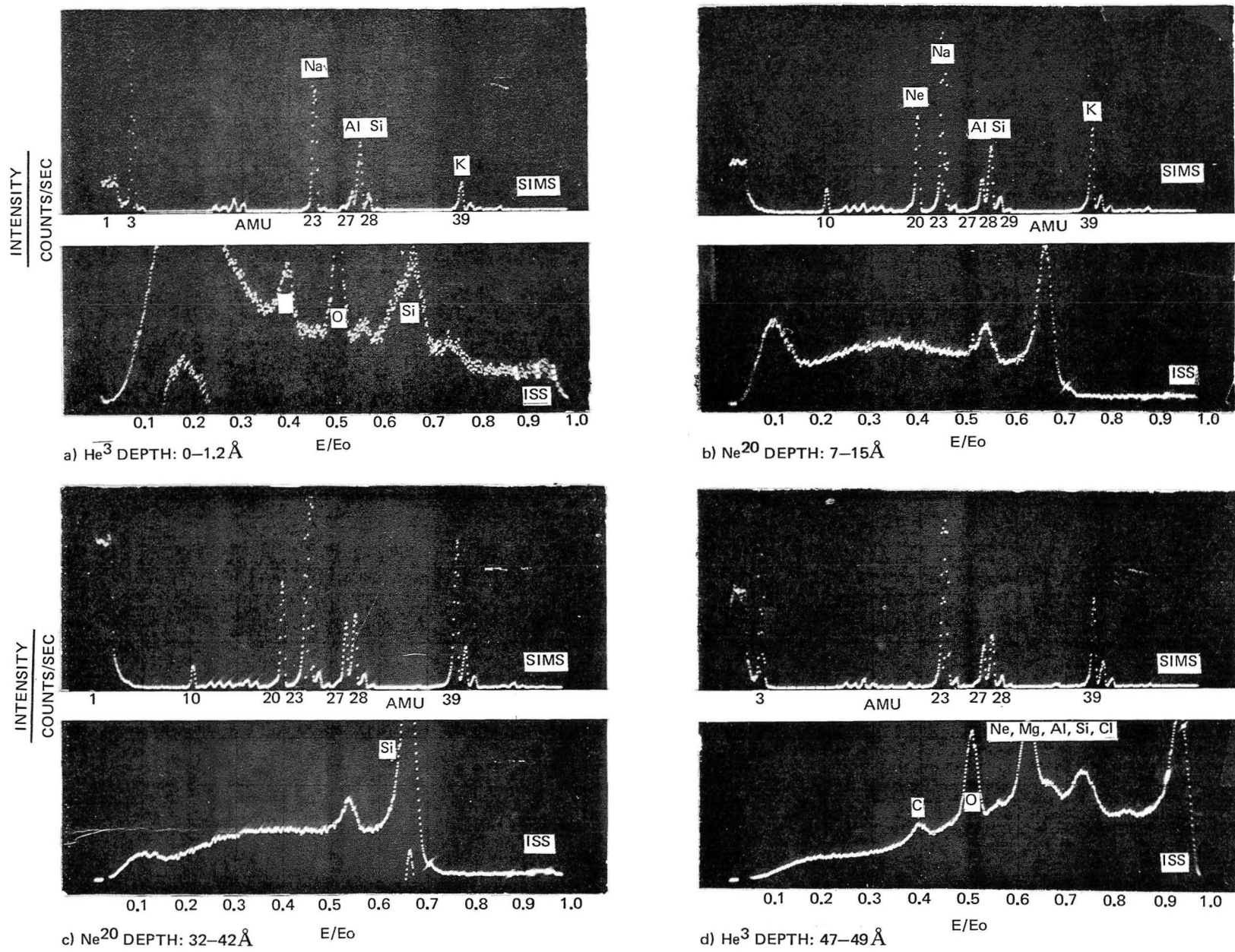
Fig. 35 Ion Scattering Spectroscopy/Scattered Ion Mass Spectrometry (ISS/SIMS) Spectra of "As Received" HTS Graphite Fibers (1500 Volts)
