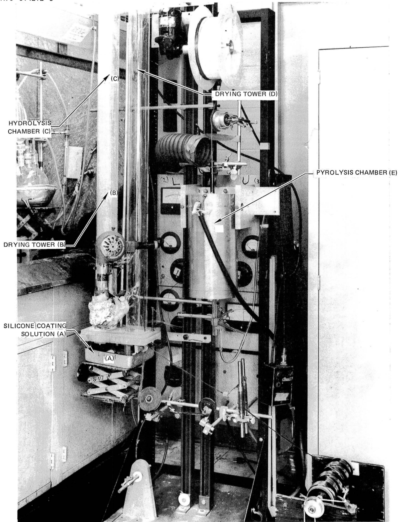
Fig. 6 Photograph of Organo-Silicone Coating Apparatus for Continuous Processing
