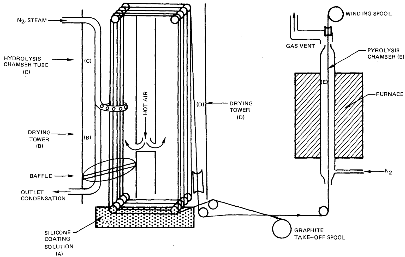
Fig. 7 Schematic of Organo-Silicone Coating Apparatus for Continuous Processing
