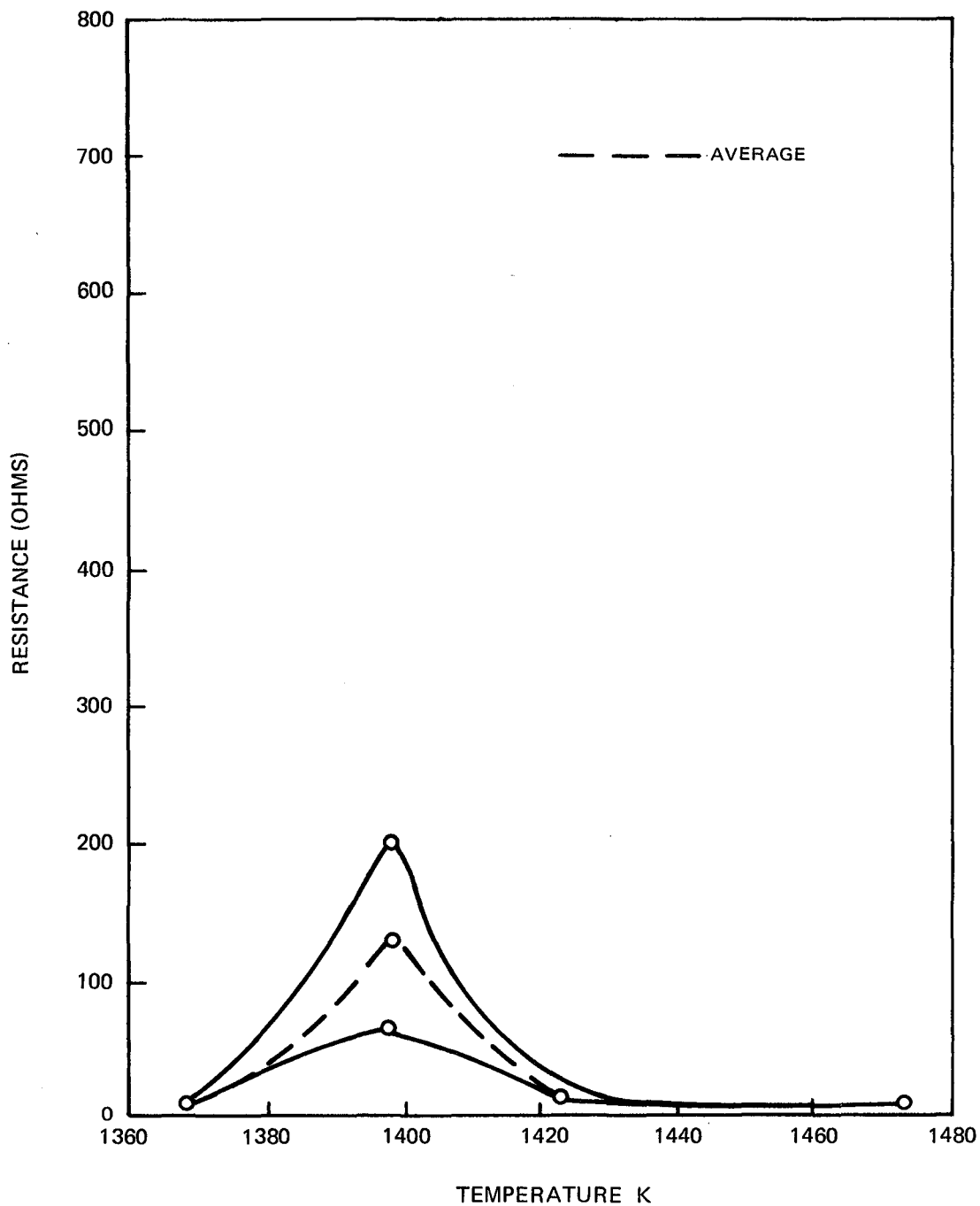
Fig. 17 Resistance vs Temperature for SiC Coated Graphite Yarn
