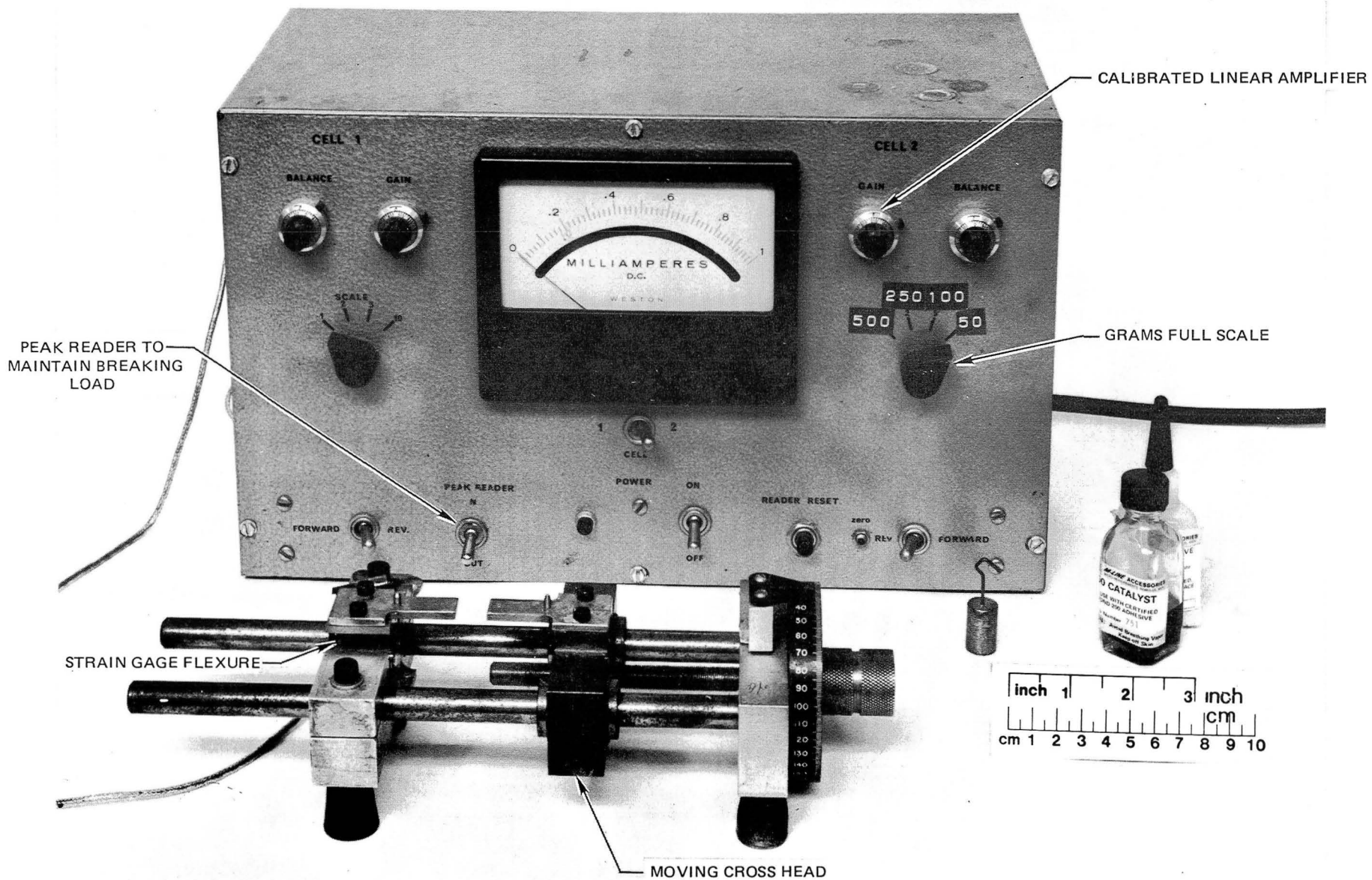
Fig. 10 Single Filament Tensile Tester
