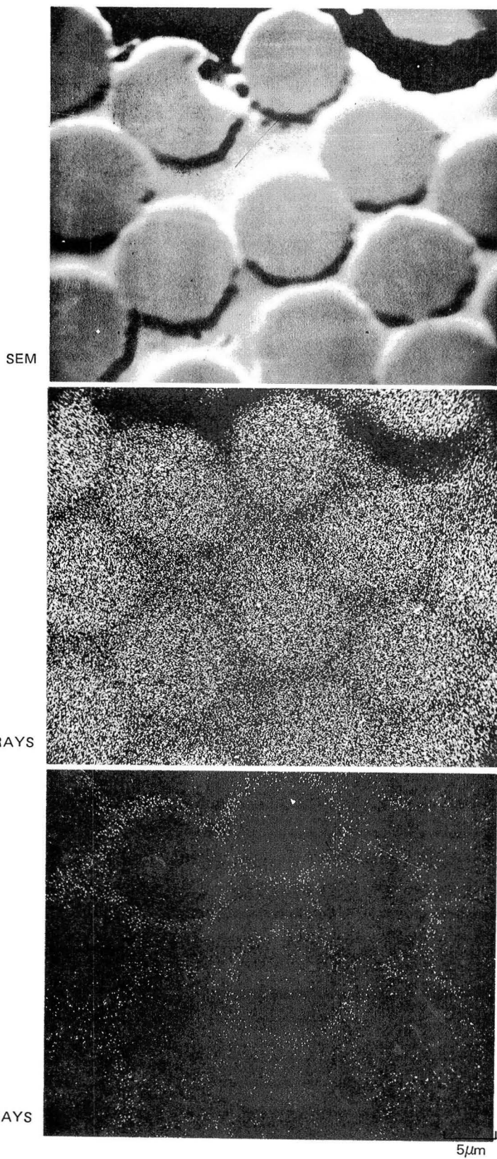
Fig. A-3 SEM and X-Ray Maps of the B Coated HTS Graphite Fibers
