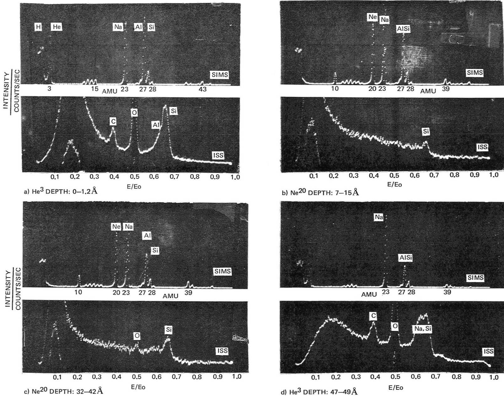
Fig. 37 Ion Scattering Spectroscopy/Scattered Ion Mass Spectrometry (ISS/SIMS) Spectra of Pyrolyzed Ethyl Silicate Coated HTS Graphite Fibers (1500 Volts)
