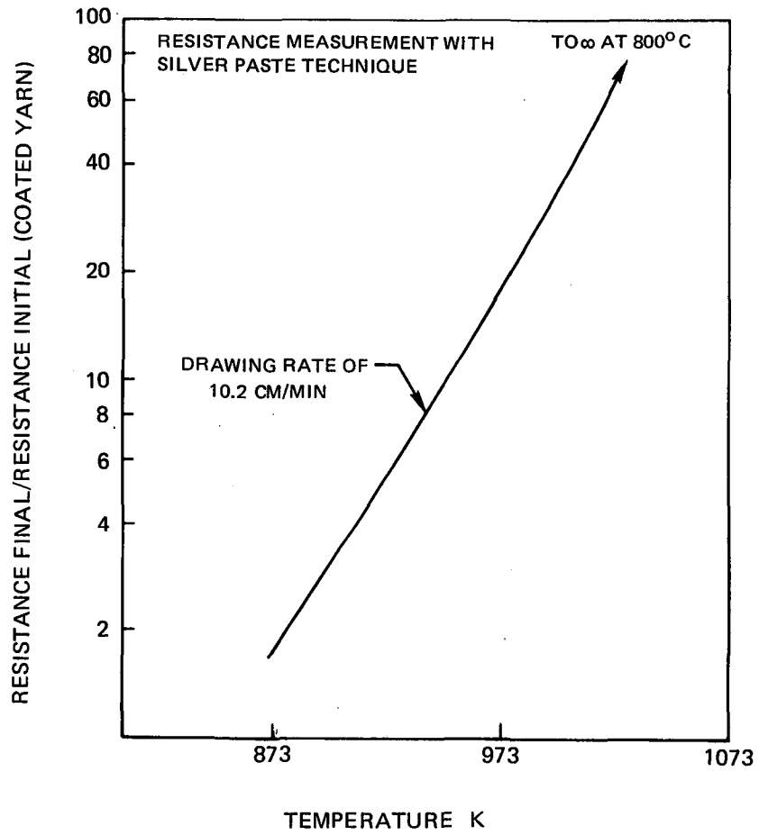
Fig. 16 Final to Initial Resistance Ratio for SiC Coated HTS Fiber Heated in Air
