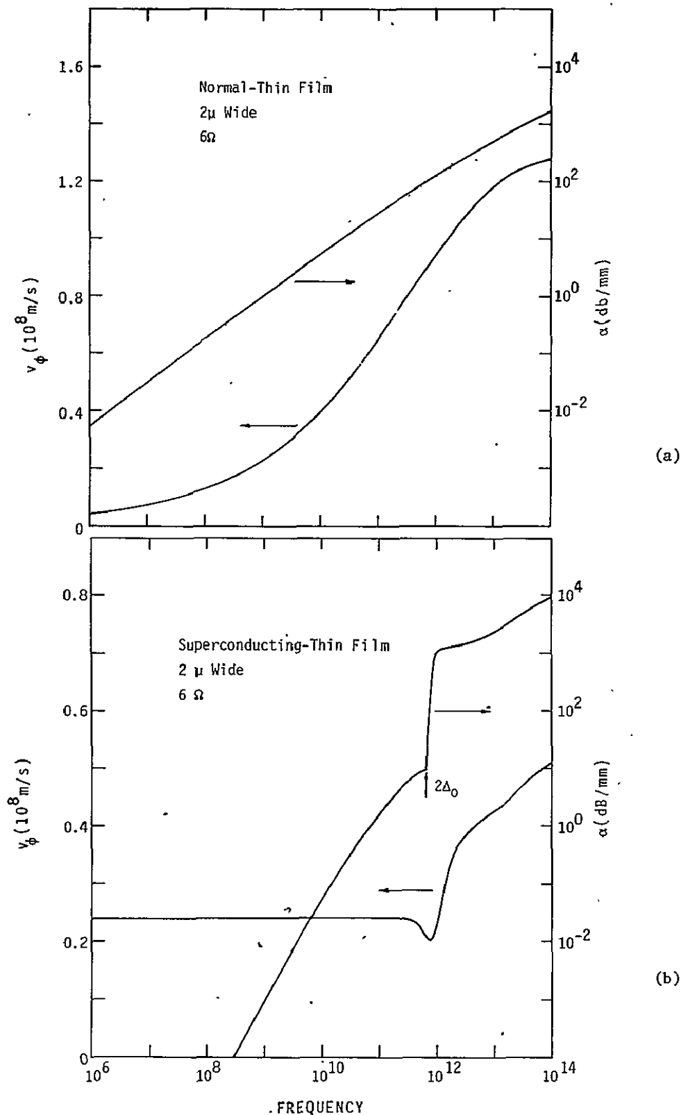
Figure IV-7. Phase velocity v_\phi and attenuation \alpha for normal and superconducting thin-film striplines. (a) is for a room-temperature copper line and (b) is for a superconducting line. Each has impedance 6 \Omega . Details are given in the text.
