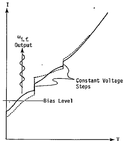
Figure V-4. The I-V curve of a Josephson mixer with externally applied local oscillator power. Application of signal power causes the curve to vary between the solid and dashed lines at the difference frequency ( f_{i.f.} ).
