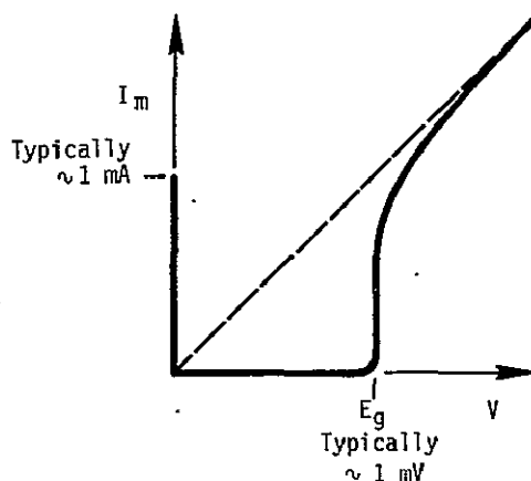
Figure IV.A-1. Time-averaged current-voltage characteristic of a Josephson junction. the dashed line is the I-V curve of the junction when it is not superconducting.
