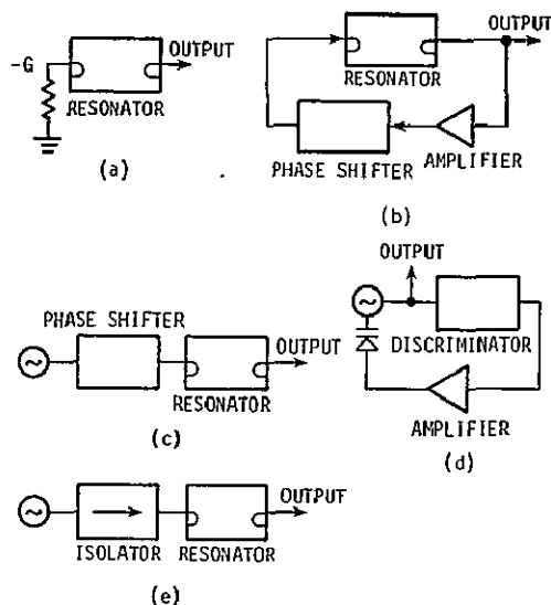
Figure VII-2. Block diagram illustrating several superconducting frequency sources: (a) negative resistance oscillator, (b) loop oscillator, (c) cavity-stabilized oscillator, (d) stabilized-voltage-controlled oscillator, and (e) passive filter.
