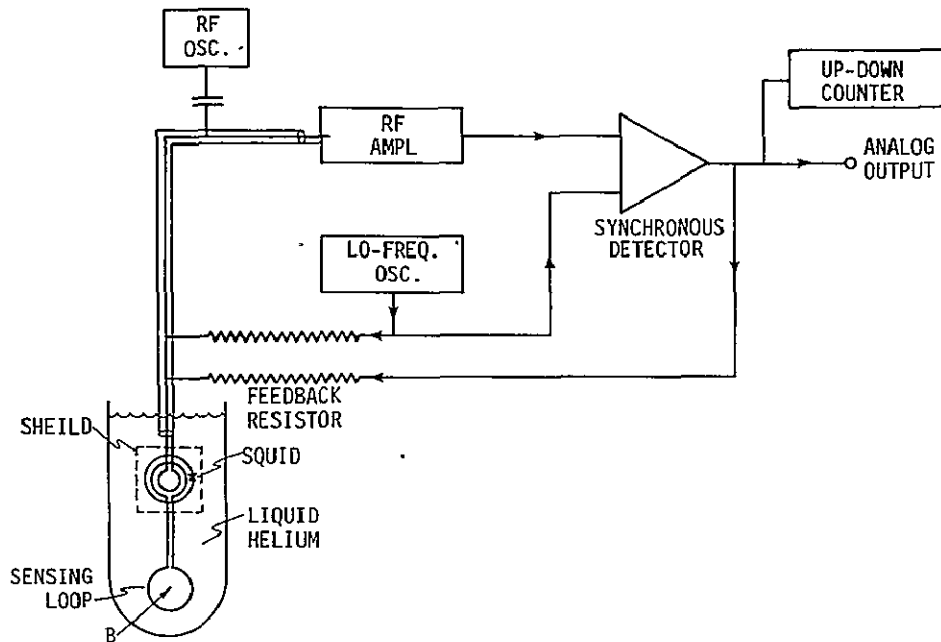
Figure III-5. Block diagram of complete single-component magnetometer, with digital readout and analog output.
