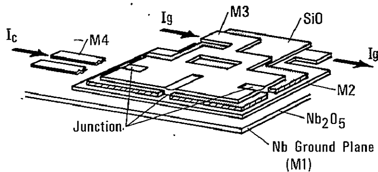
Figure IV-4. Quantum interference Josephson gate composed of three junctions in parallel. The labels M_n refer to different layers of metallization. Two control lines are shown at the left. They are not drawn across the top of the device so as to reveal junction structure. I_c is a control current, and I_g is the bias current for the gate.
