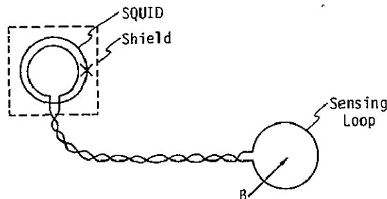
Figure III-3. Schematic representation of a shielded SQUID coupled to the field B through a flux transformer. Bias and amplifier circuit is not shown. The SQUID is shown here symbolically as a circle with a small cross representing the junction. The entire transformer, including the sensing loop is superconducting.
