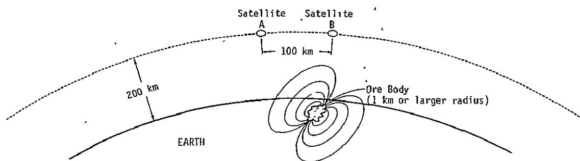
Figure III-7. Suggested system for magnetic survey of the earth. Magnetometers are located in each of the two satellites. The system acts as a very long baseline gradiometer, thus discriminating against interference from distant sources.
