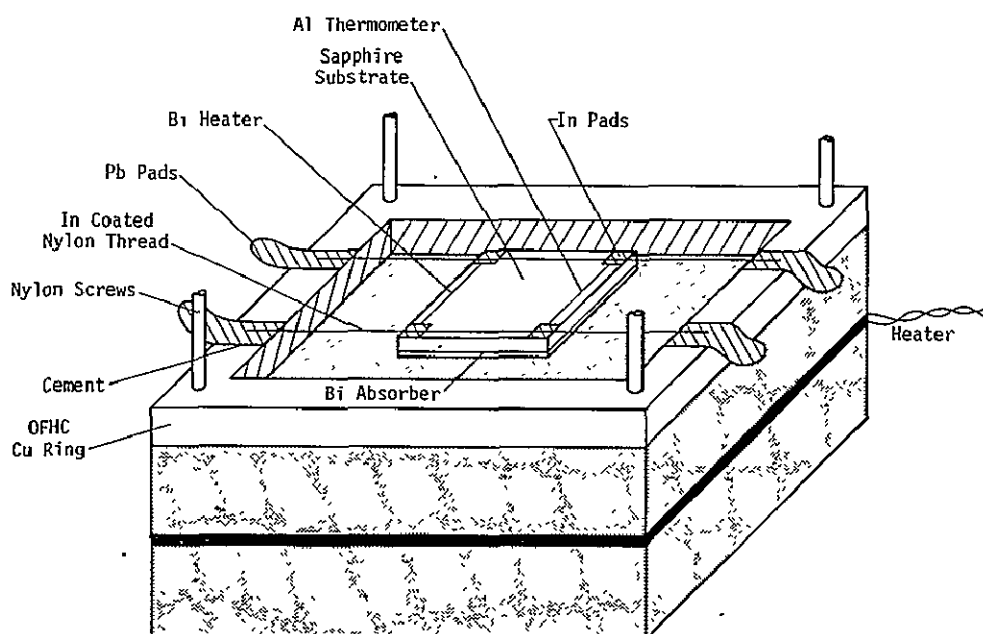
Figure V-1. Typical structure for a composite bolometer (after Clarke, et al., 1978). Radiation absorbed in the bismuth film heats the sapphire substrate causing a change in the resistance of the aluminum superconducting transition edge thermometer.
