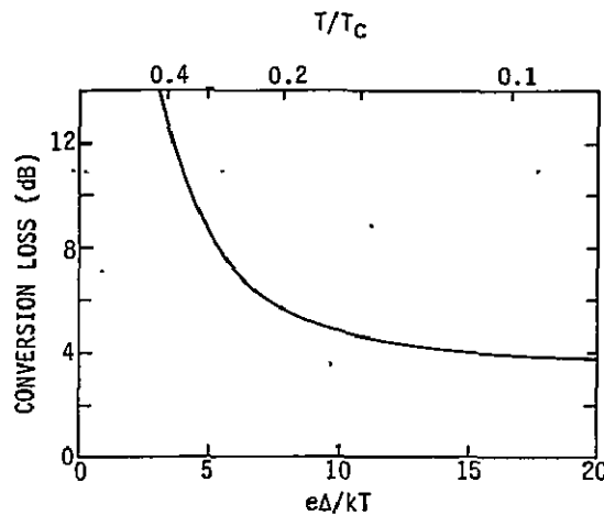
Figure V-2. Intrinsic conversion loss of a super-Schottky diode as a function of the ratio of the energy gap e\Delta to the thermal energy kT (after Vernon, et al., 1977). In practice parasitic losses often considerably increase this loss.
