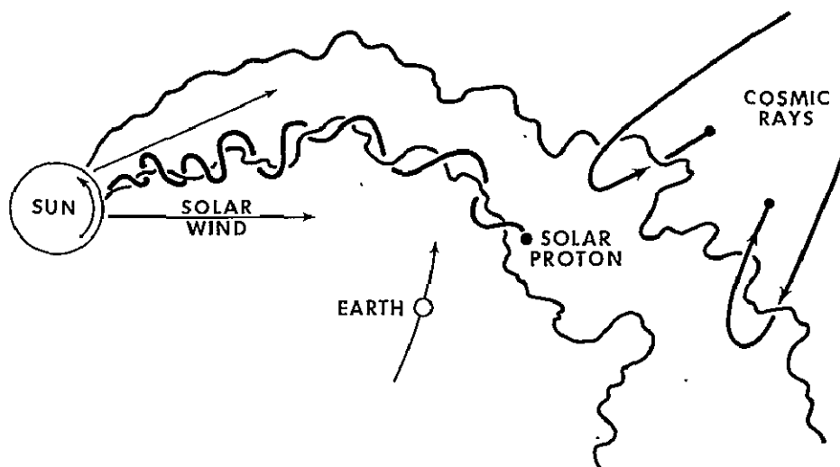
Figure III-8. Hypothetical instantaneous picture of two representative field lines. The path of a high-energy proton spiraling around a field line is indicated, and also the paths of charged particles (cosmic rays) from outer space (from Smith and Sonett).
