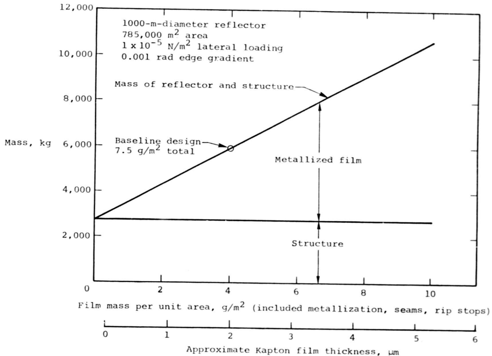
Figure 12. Variation of structure and reflector mass with film thickness (mass) for a 1000-m circular satellite.
