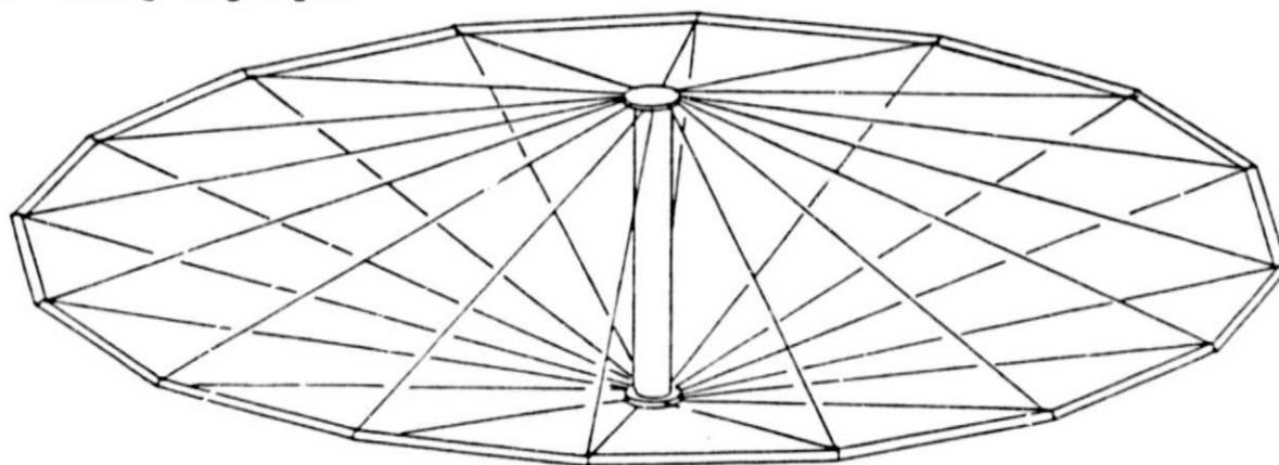
Figure 10. Segmented rim structure for deploying space equipment. (This Astro figure was published in NASA CR-2347, "Spoked Wheels to Deploy Large Surfaces in Space - Weight Estimates for Solar Arrays.")
