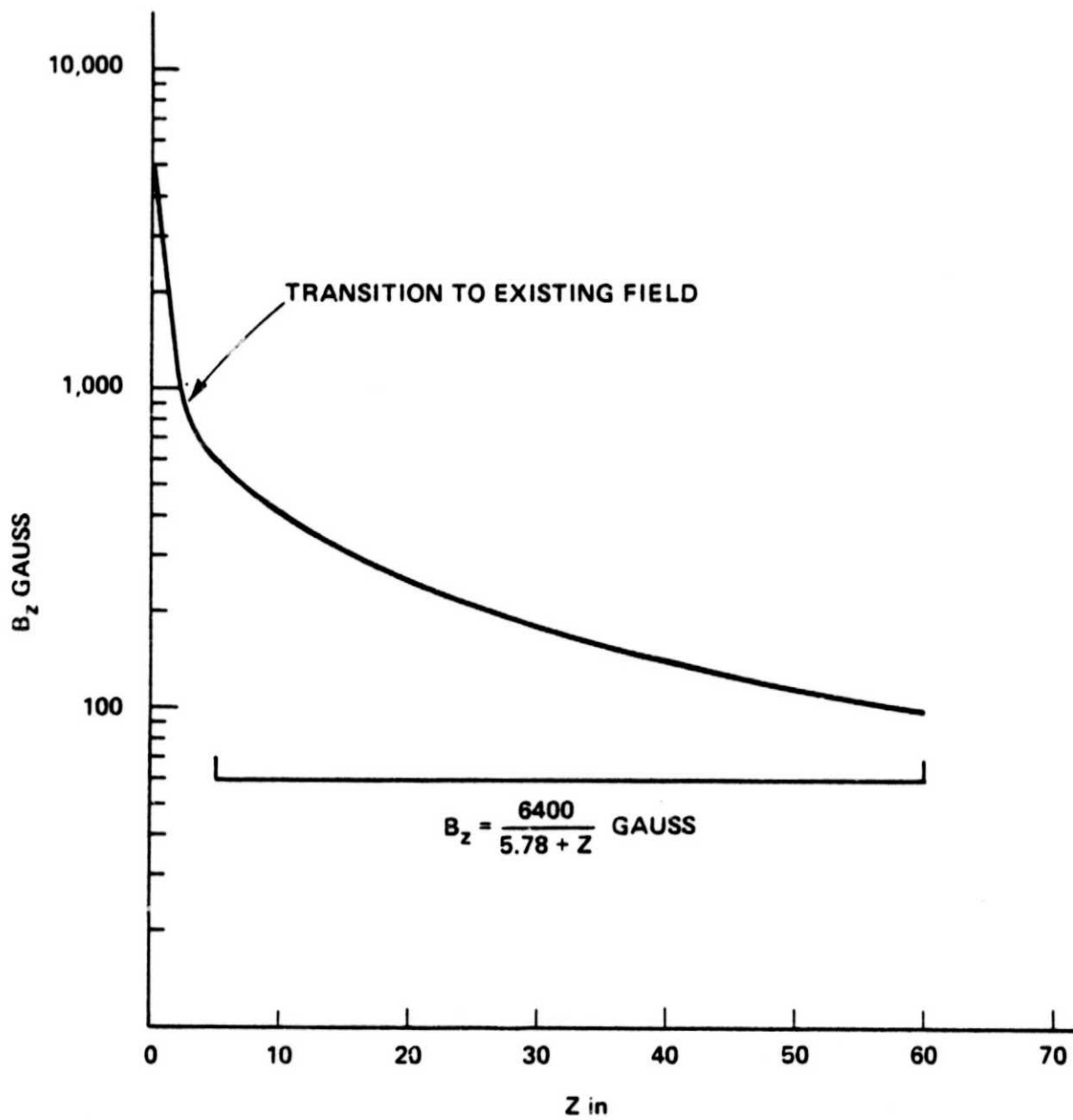
FIGURE 4. MAGNETIC FIELD FOR TRAJECTORIES OF FIGURE 2
