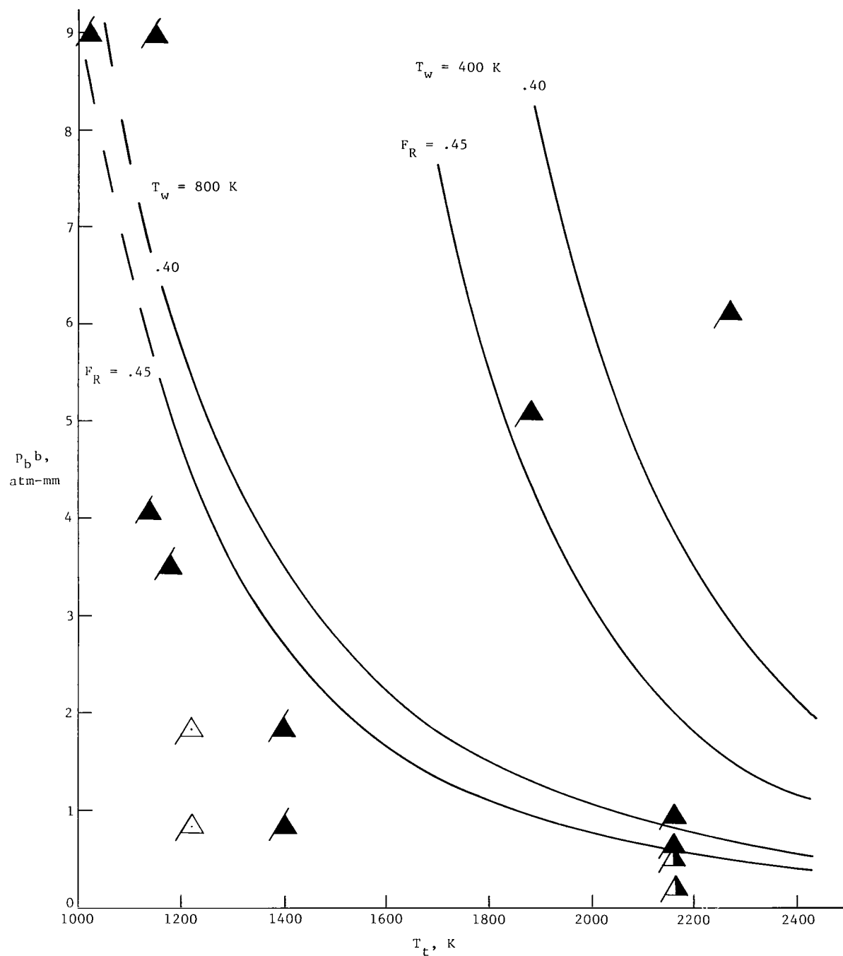
Figure 18.- Data correlation for strut bases (swept base model). See table II for explanation of data symbols.
