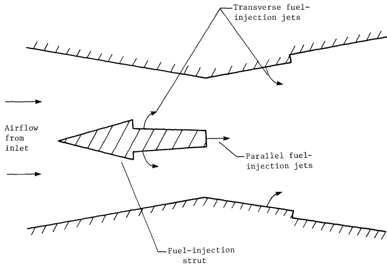
Figure 6.- Probable self-ignition points in a scramjet combustor.
