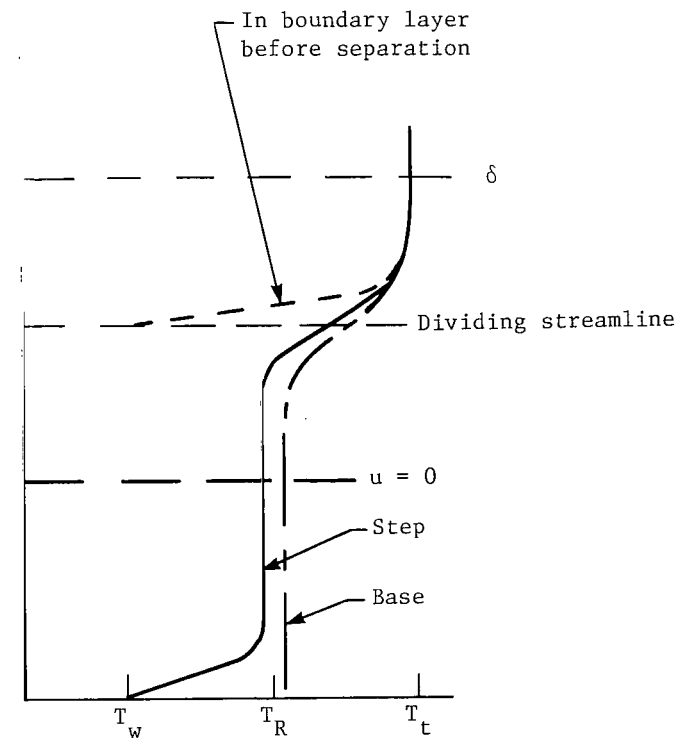
Figure 14.- Temperature profile in step and base recirculation zone.
