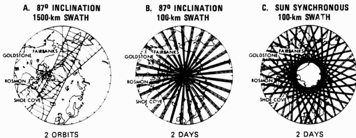
FIGURE 4. SWATH WIDTH EFFECTS ON POLAR COVERAGE
