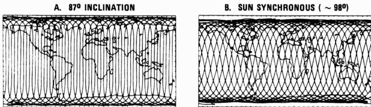
FIGURE 3. INCLINATION EFFECTS ON SWATHING PATTERNS
