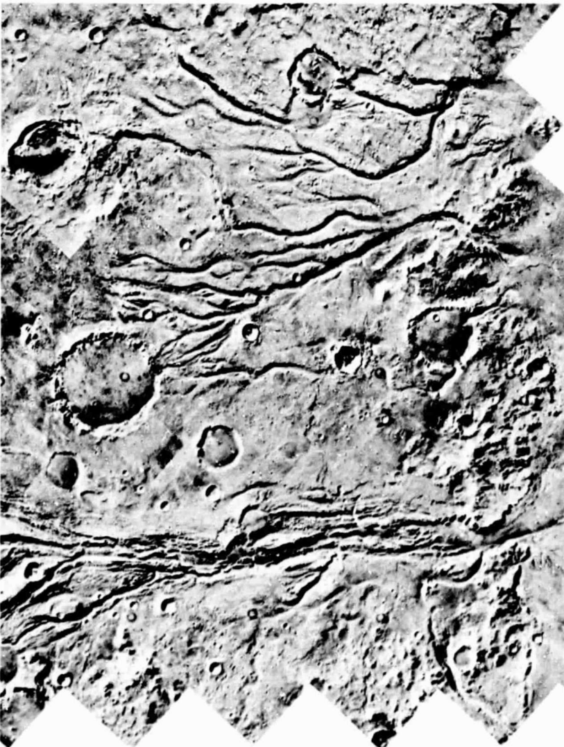
Figure 16. The Vanished Rivers of Mars. Cameras in the Viking 1 Orbiter photographed this maze of wandering channels that cut across the terrain west of the Viking 1 landing site. The surface slopes downward, dropping about 3 kilometers (2 miles) in elevation from left to right. Flood waters once poured across this region from left to right, cutting through a high ridge (right) to pour out into the plains to the east. Older craters were cut, filled, and eroded by this flood. Younger craters, formed after the flood, show sharp outlines. The fate of these torrents is unknown; the water may now be frozen as ice in the polar caps or as permafrost in the Martian soil. Rows of dark circles are photographic flaws.
