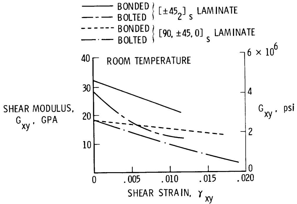
Figure A2.- Effect of rail configuration on shear modulus behavior. (See fig. 11.)
