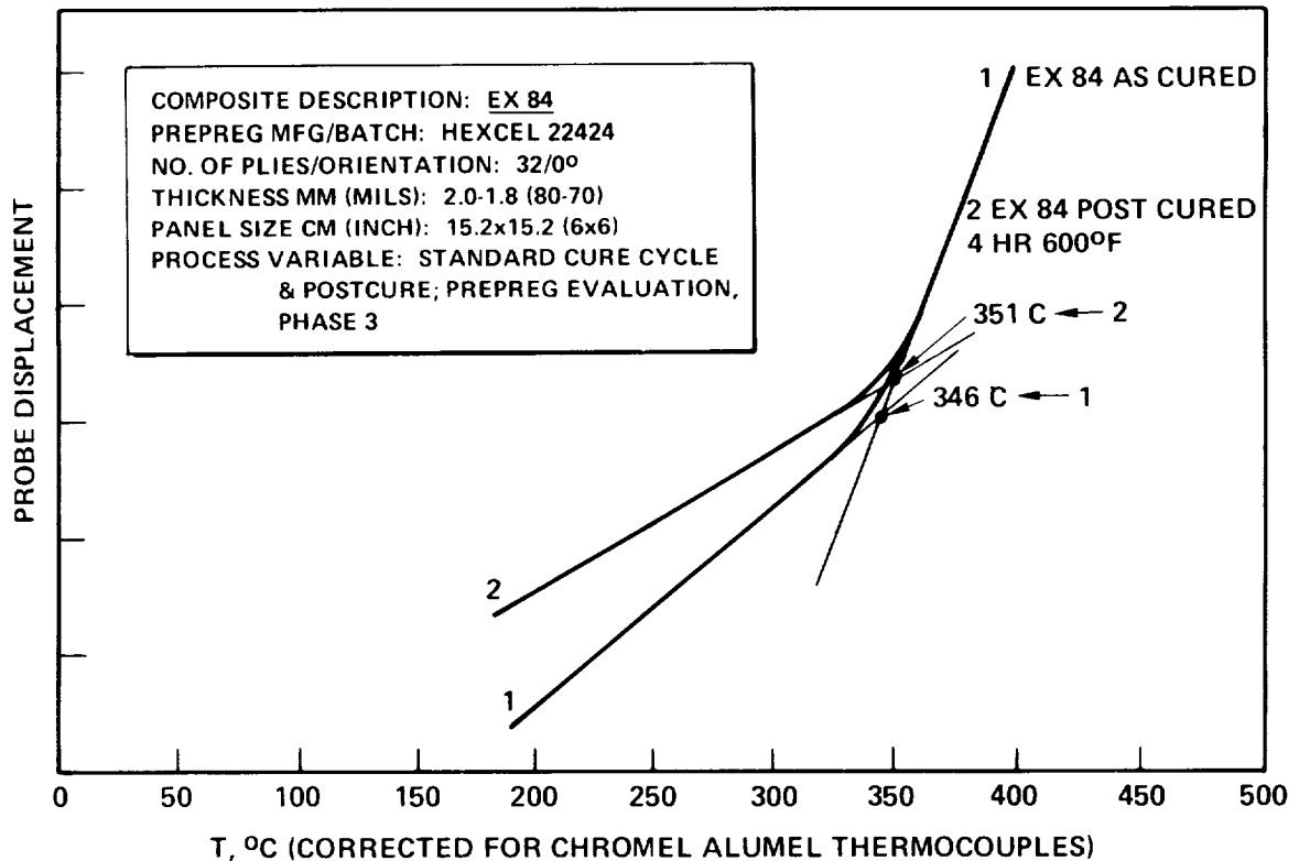
TMA/Tg-TYPICAL RESULTS
