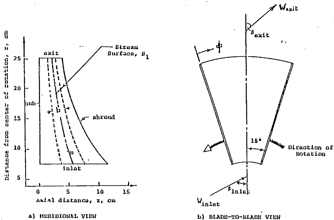
FIG. 12. HUB-SHOULD PROFILE WITH THE STREAM SURFACE, S_1 , USED FOR BLADE-TO-BLADE ANALYSIS (COMPRESSOR CASE).
