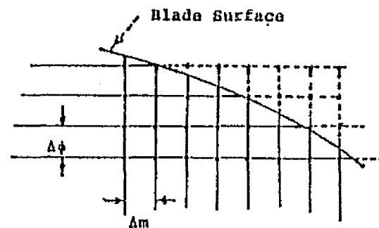
Detail A-A: Grid Points Near the Blade Surface.
