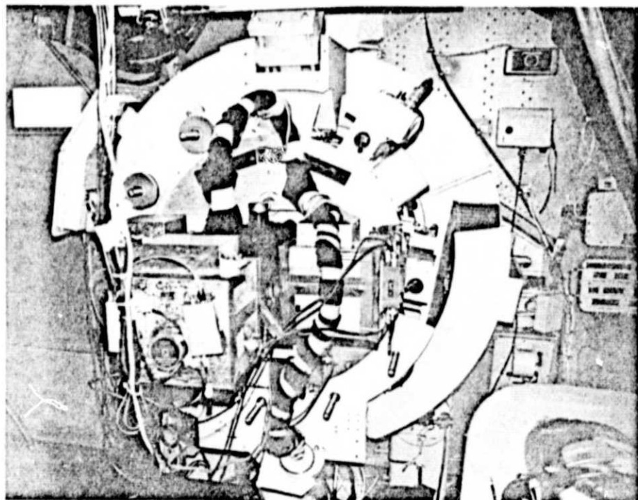
In this view inside the KAO, the photoelectric photometer employed for the occultation is mounted at the bent Cassegrain focus of the 36-inch telescope. Except as noted, all illustrations are from the authors.
