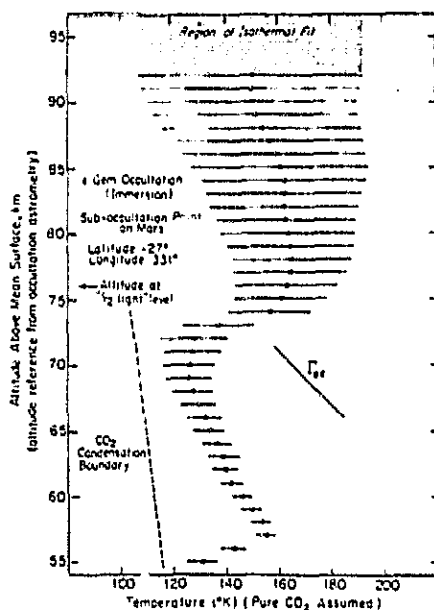
Fig. 1 (left). Temperature profiles for immersion. The plotted points and their error bars were obtained from the immersion light curve for a pure CO 2 atmosphere. A correction for the small amount of N 2 and Ar present would lower the temperatures about 3°K. The uncertainty in the altitude scale is \pm 5 km, and an altitude of 65 km corresponds to a number density of 2.0 \times 10^{14} cm -3 . The shaded region represents the uncertainty in the temperature obtained from the isothermal fit used to establish the boundary condition for the inversion calculation. The largest temperature gradients are subadiabatic ( \Gamma_{ad} = -5^\circ\text{K km}^{-1} ). The wavelike structure strongly suggests the presence of tides in the martian atmosphere. At the time of the occultation, the martian subsolar latitude was +19.2° and the planetocentric longitude of the sun ( L_s ) was 51.6°. Immersion occurred above the suboccultation point on Mars at about 0330 local solar time. Fig. 2 (right). Temperature profile for emersion, which occurred above the suboccultation point on Mars at about 1530 local solar time. For details, see the legend for Fig. 1.
