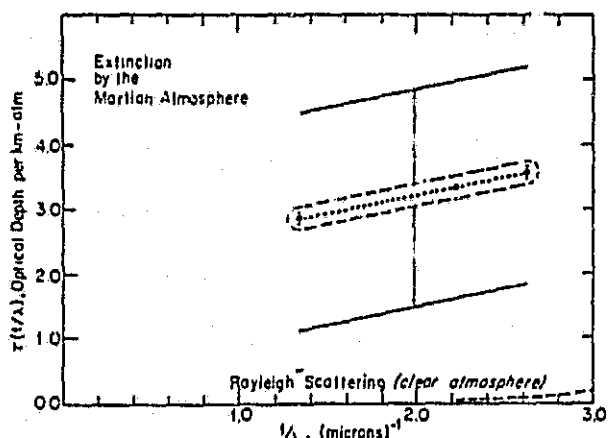
FIG. 18.—Extinction by the Martian atmosphere as a function of wavelength, determined from the central flash. The central flash probes the atmosphere along a slant path whose closest approach to the Martian surface is at an altitude of 25 km. This corresponds to a column density of about 4 Martian atmospheres. The large error bar represents the uncertainty in the absolute optical depth, estimated by comparing synthetic central flash profiles to the data. The small error bars show the uncertainty in the relative extinction from channel to channel, determined from relative fluxes of the central flash in each channel.
