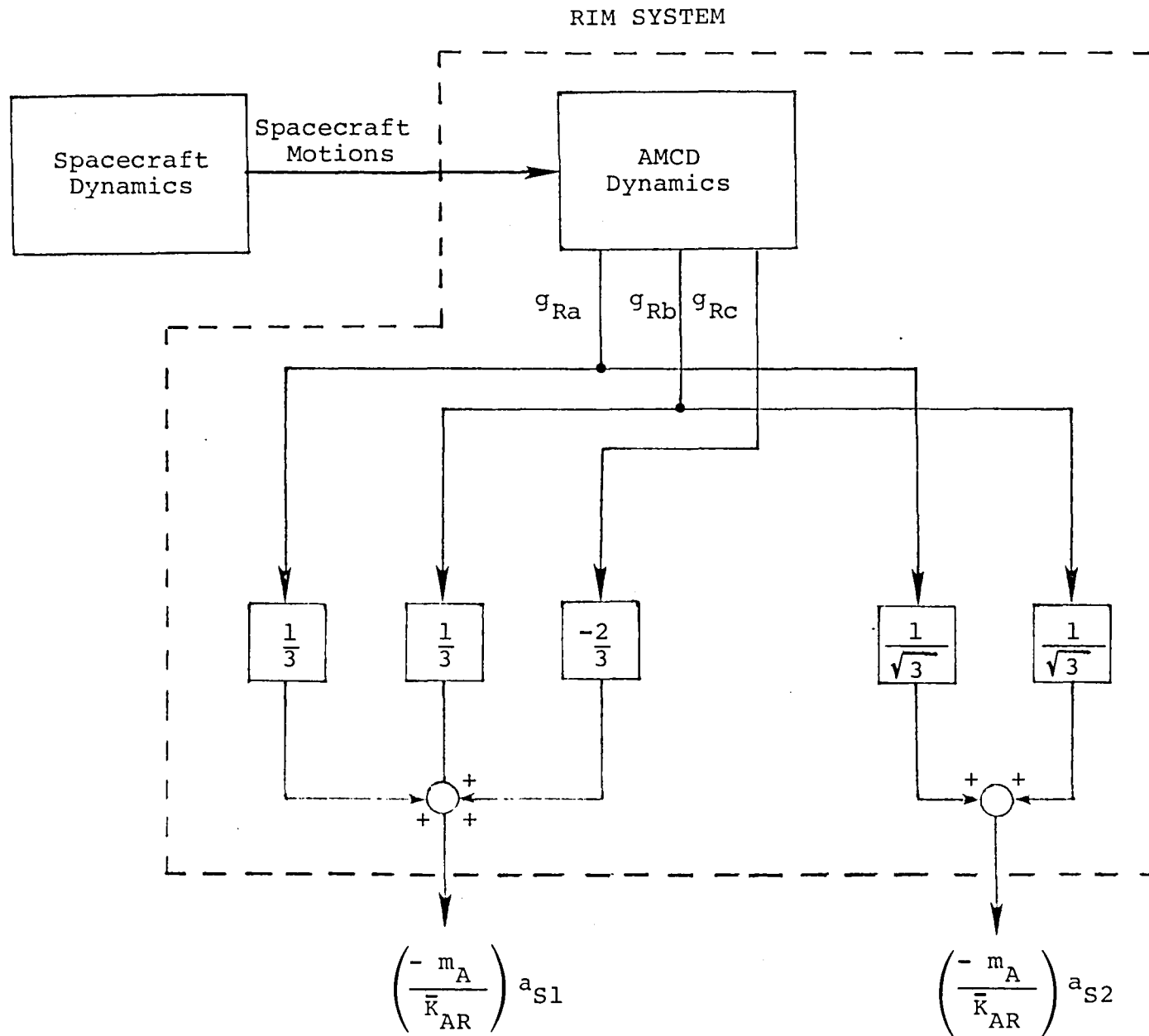
Figure 4.- Measurements from radial components of RIM system.
