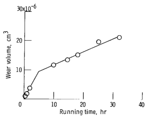
Figure 2. - Typical wear versus time curve. Iron rider on 52100 steel disk; lubricant, hexadecane; atmosphere, nitrogen; sliding speed, 3 rpm; load, 4.9 N (500 g).
