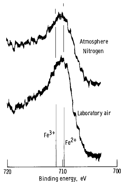
Figure 4. - Fe 2p 1/2 peaks from wear scars. Lubricant, hexadecane; sputter etch duration, 30 seconds.
