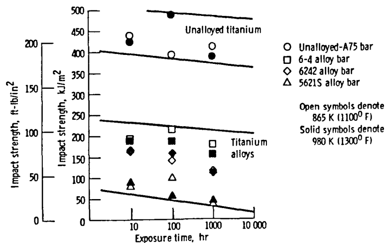
Figure 2 - Room temperature notched, Izod impact strength of unreinforced titanium and titanium alloys after air exposure at 865 K (1100°F) or 980 K (1300°F).
