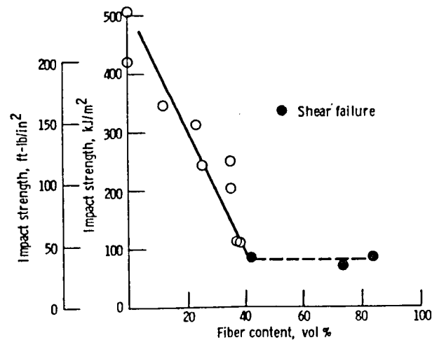
Figure 6. - Room temperature notched Izod impact strength of SiC/A-40 Ti composites containing various amounts of fiber.
