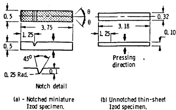
Figure 1 - Configuration and dimensions of notched, miniature Izod impact specimens and unnotched, thin-sheet Izod impact specimens. (All dimensions in centimeters.) Note: Ply angle \theta is the angle between the fiber and the longitudinal centerline of the specimen.
