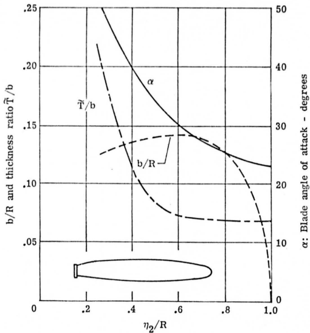
Figure 4. - Blade form curves and the planform for the general aviation propeller used for in-flight acoustic measurement. b = Chord, \tilde{T} = maximum thickness of airfoil, R = blade radius, \eta_2 = distance from propeller center.
