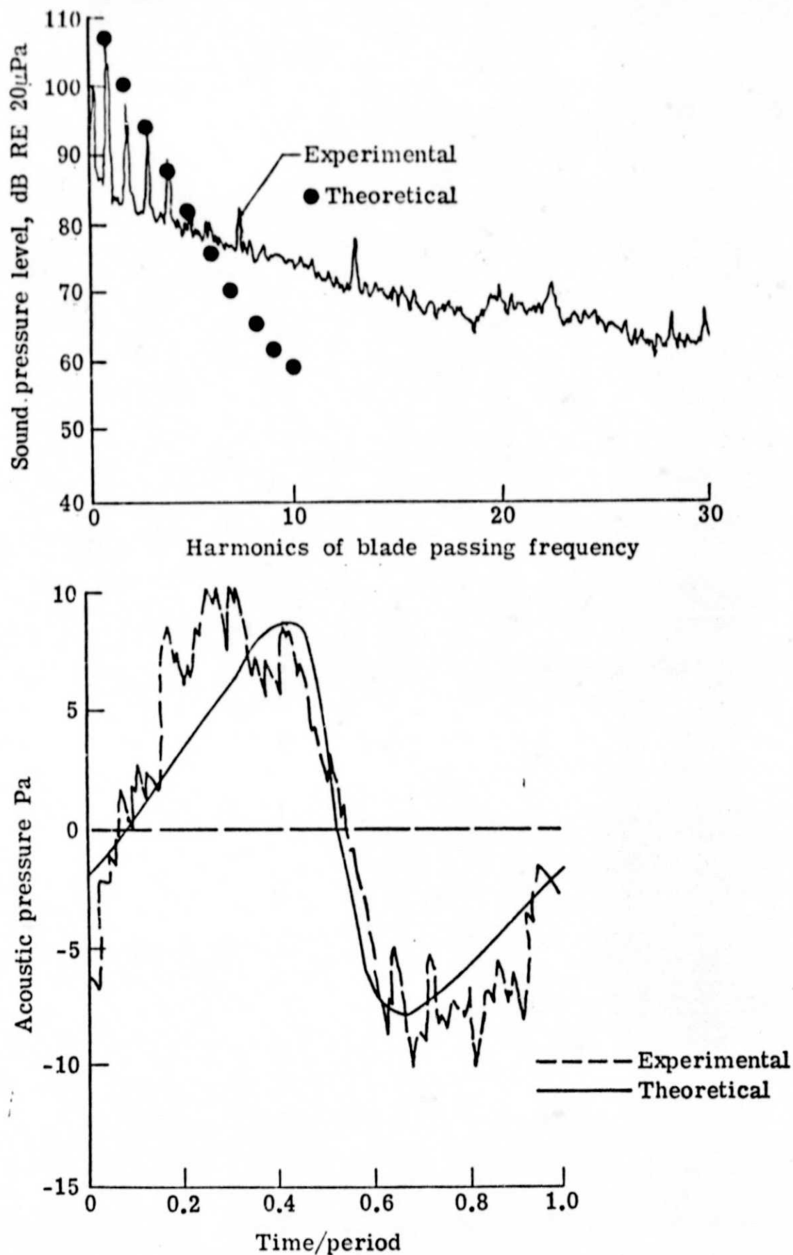
Figure 8(a).- Calculated and measured acoustic pressure signatures and spectra for the general aviation propeller. Run 3A, In-plane microphone, period = 11.36 msec.
