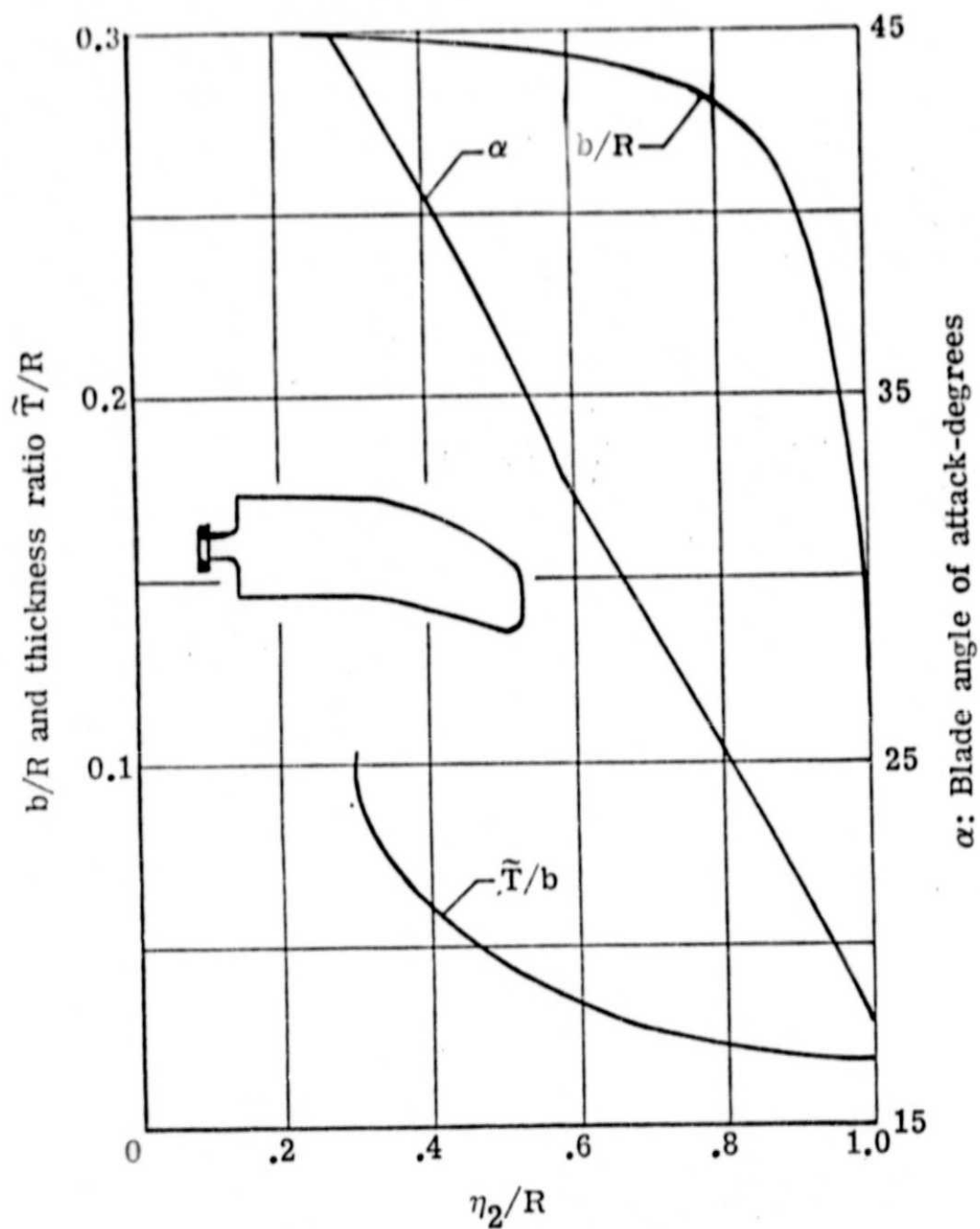
Figure 11.- Blade form curves and the planform for the advanced propeller. b = chord, T = maximum thickness of airfoil, R = blade radius, \eta_2 = distance from propeller center.
