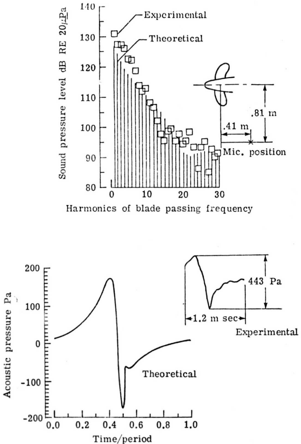
Figure 14.- Comparison of theoretical and experimental acoustic pressure signatures and spectra for the advanced propeller. Period = 2.667 msec, number of blades = 2.
