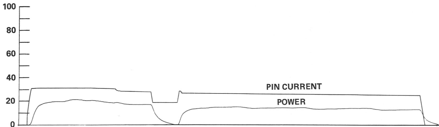
Figure 36(a). Chart Record of Calorimeter and Pin Current (3/28/77, Chart Speed 1" = 60 sec)
