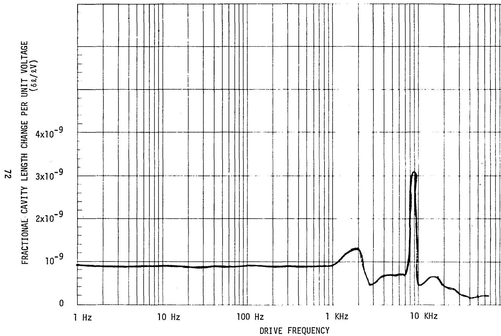
Figure 45. Frequency Response of Cavity Length Tuner
