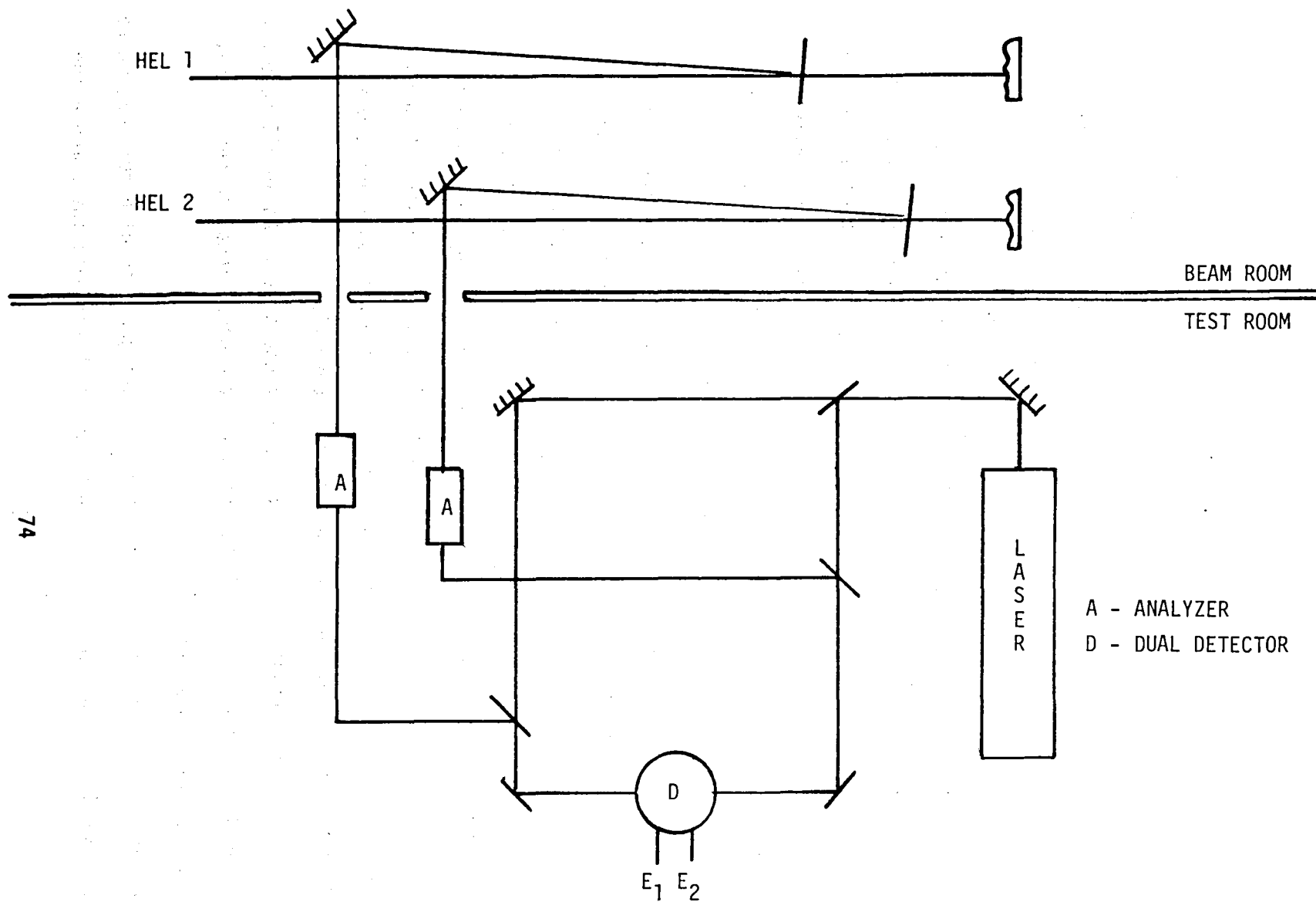
Figure 46. Heterodyne Phase Lock Test System (Simplified)
