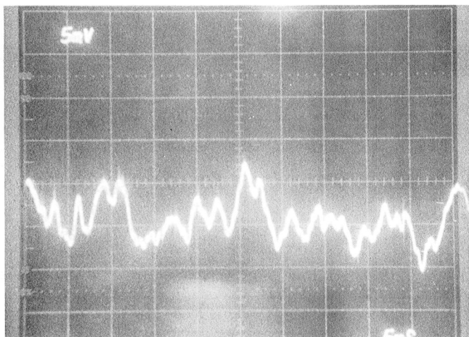
(a) POWER SUPPLY RIPPLE AT ANODE (X1000 PROBE) 5 V/DIV
