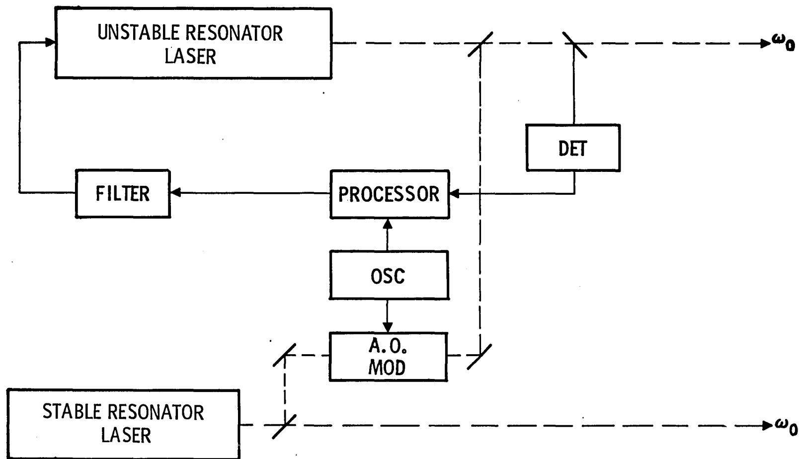
Figure 22. Functional Block Diagram of Unstable Resonator Laser Phase Locking Demonstrator
