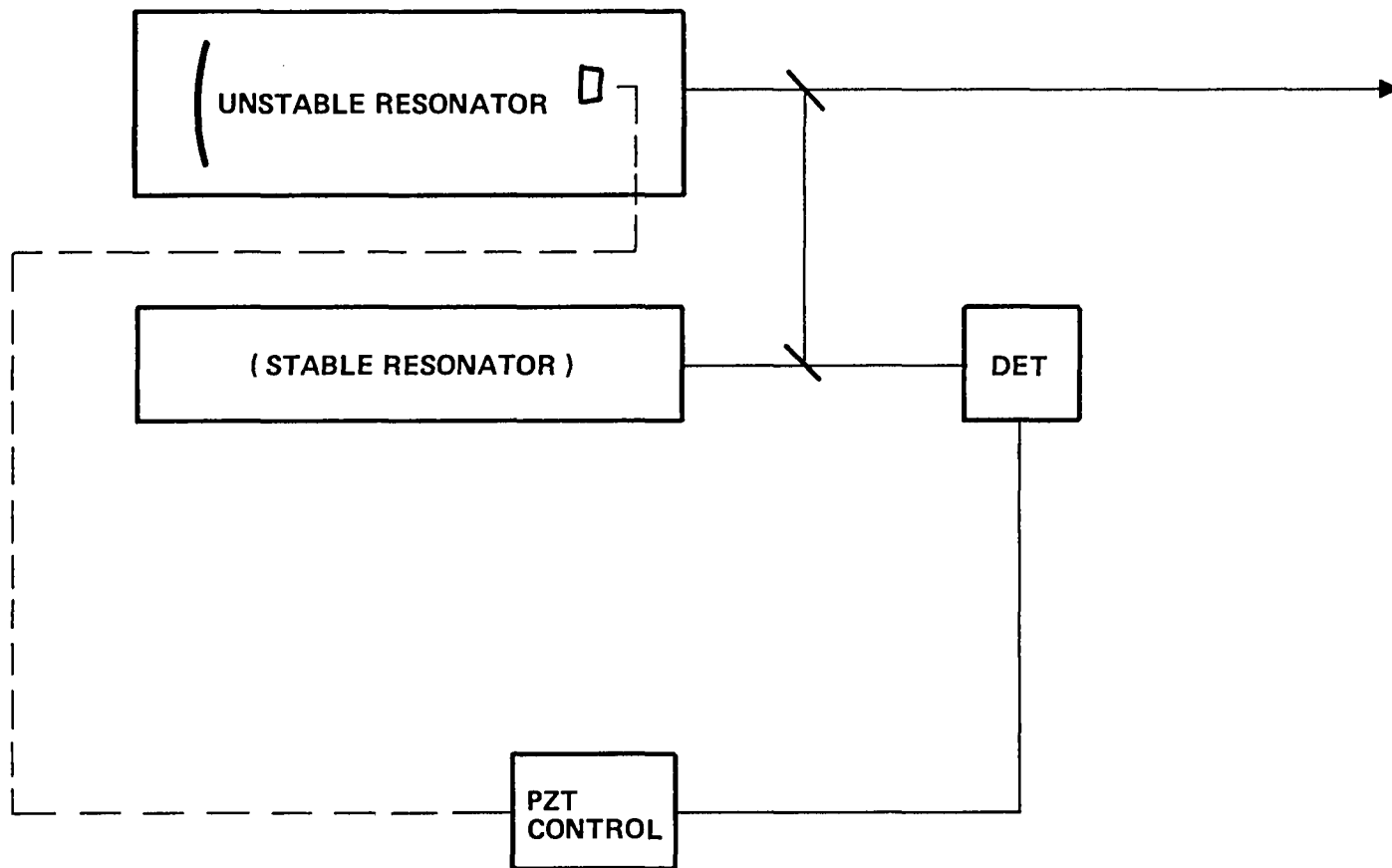
Figure 56. Phase Lock Tests HEL to Low Power Reference
