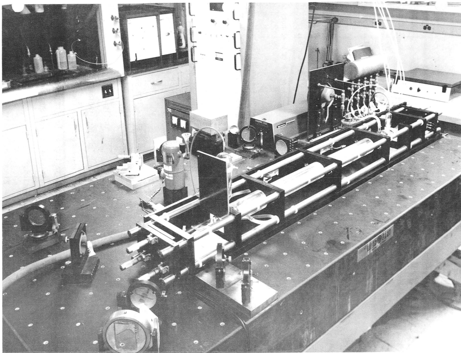
Figure 13. Unstable Resonator for Low Pressure Phase Lock Tests
