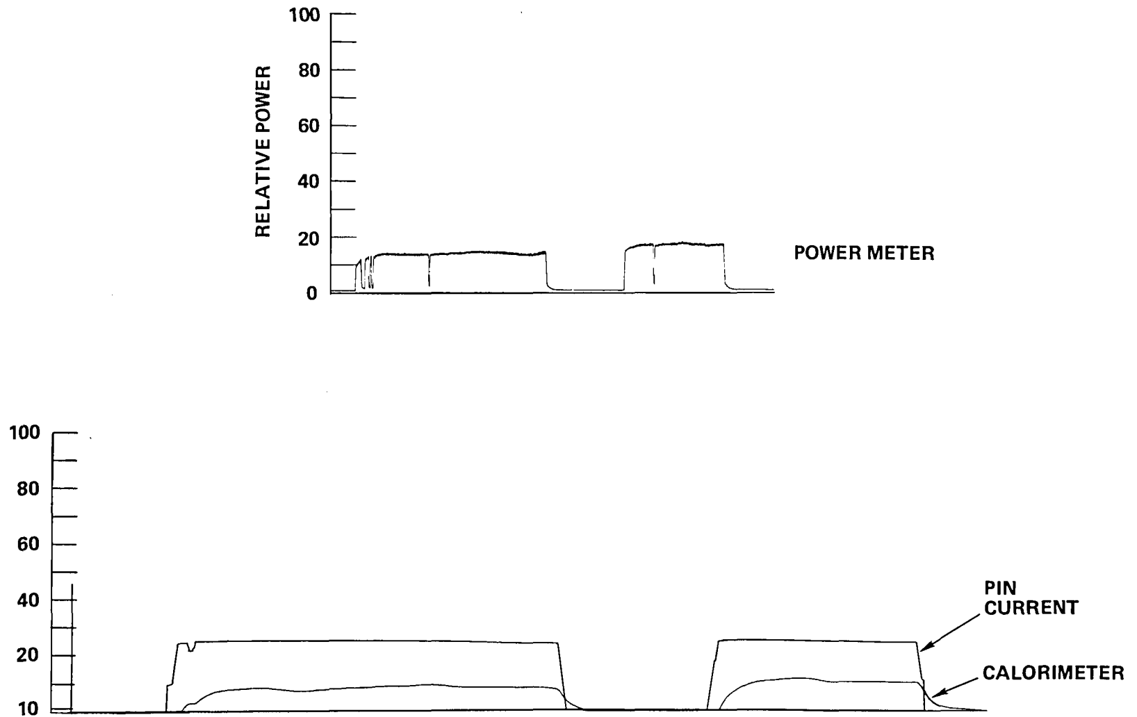
Figure 38. Runs #5 and #6, 3/28/77, Chart Records of Calorimeter and Pin Current (Chart Speed 1" = 60 sec) and Power Meter (Chart Speed 1" = 120 sec)
