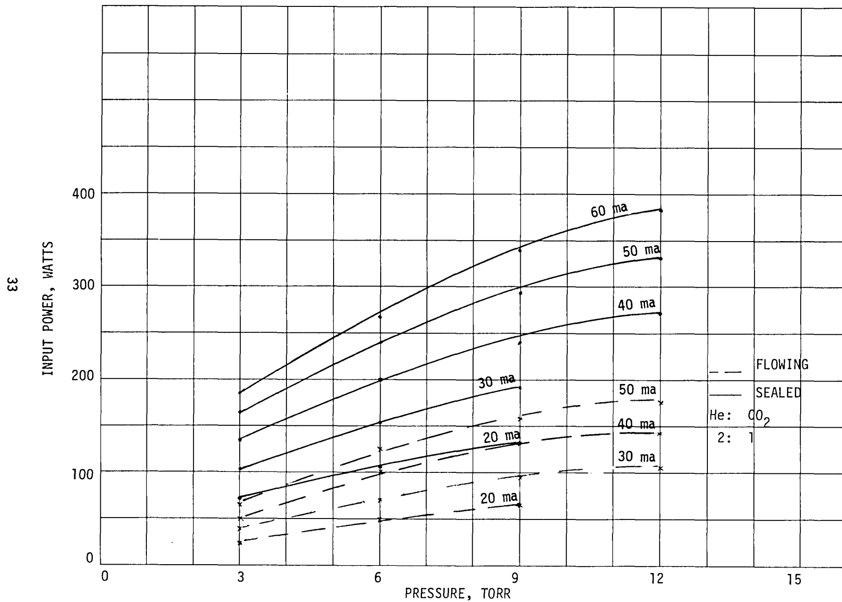
Figure 20. Pressure/Power Dependence for Flowing and Sealed-Off Operation
