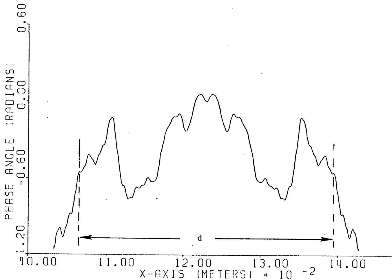
Figure 5. Near Field Phase Distribution of Passive Cavity in the Plane of Mirror 1 When Scraper Mirror is Removed ( d = hole diameter of scraper mirror).
