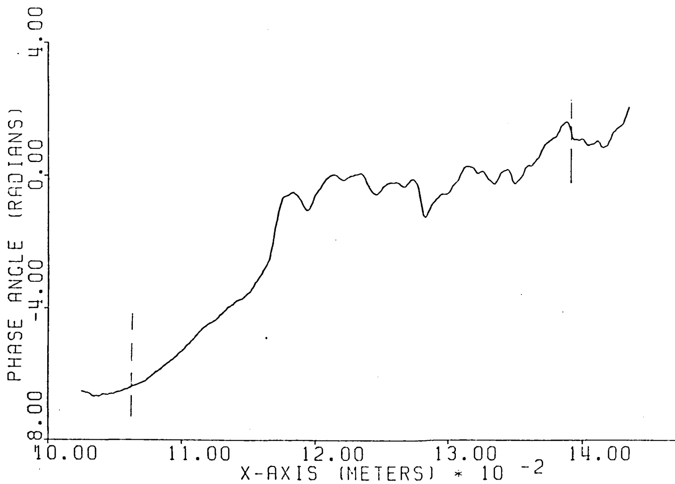
Figure 11. Near Field Phase Distribution (Focus Error \sim 1.5\% ; Tilt Angle of Large Mirror = \lambda/4d_0 )
