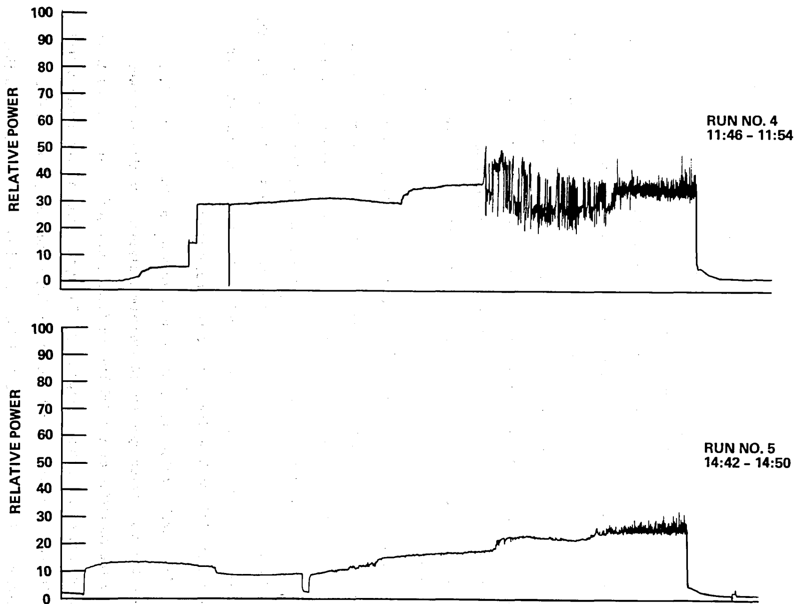
Figure 27. Power Meter Output for Runs #4 and #5, 3/24/77 (Chart Speed: 1" = 40 sec)
