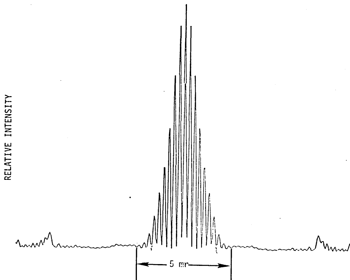
Figure 6. Far Field Intensity Distribution of Passive Cavity
