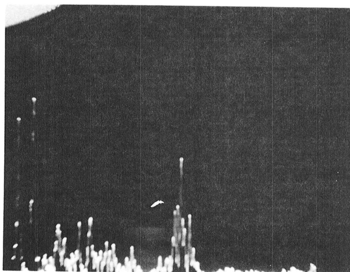
Figure 57. Spectrum of HEL Heterodyne Lock Signal (Frequency Lock Condition)
