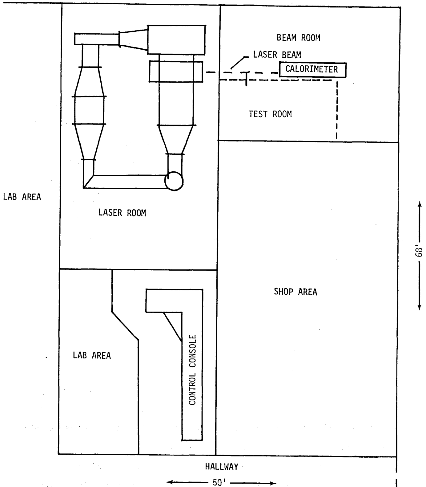
Figure 25. NASA-Lewis HEL Laser Facility
