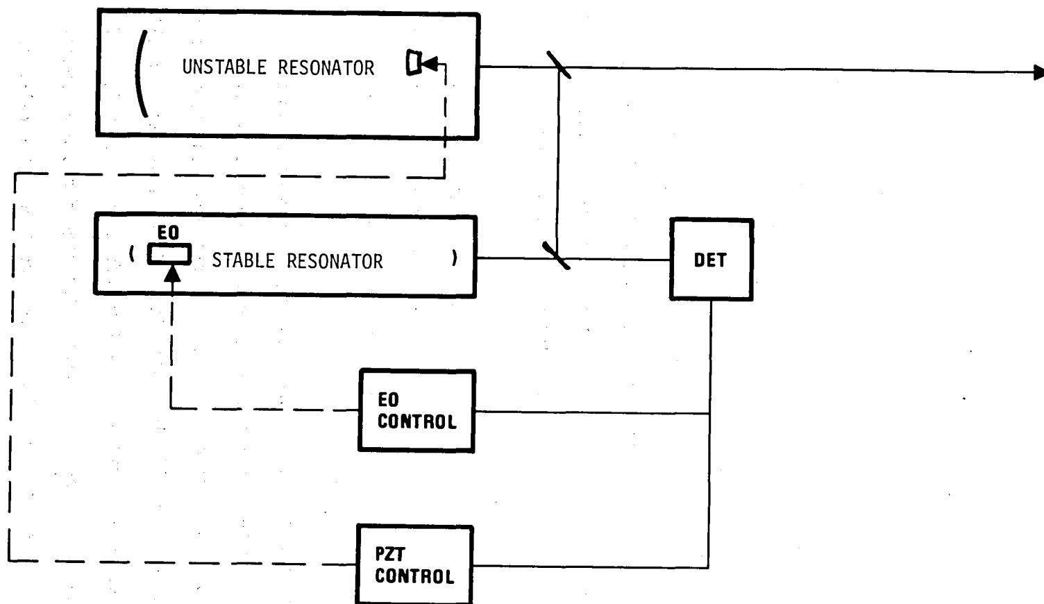
Figure 59. Phase Lock Tests HEL to Low Power Reference
