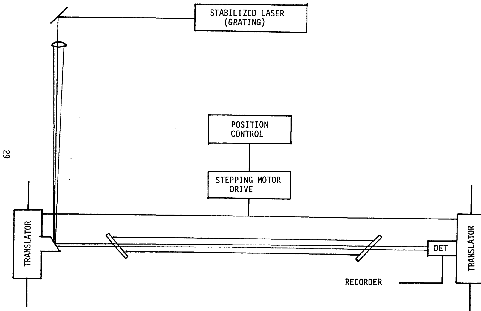
Figure 16. Apparatus for Measuring Radial Gain Profile
