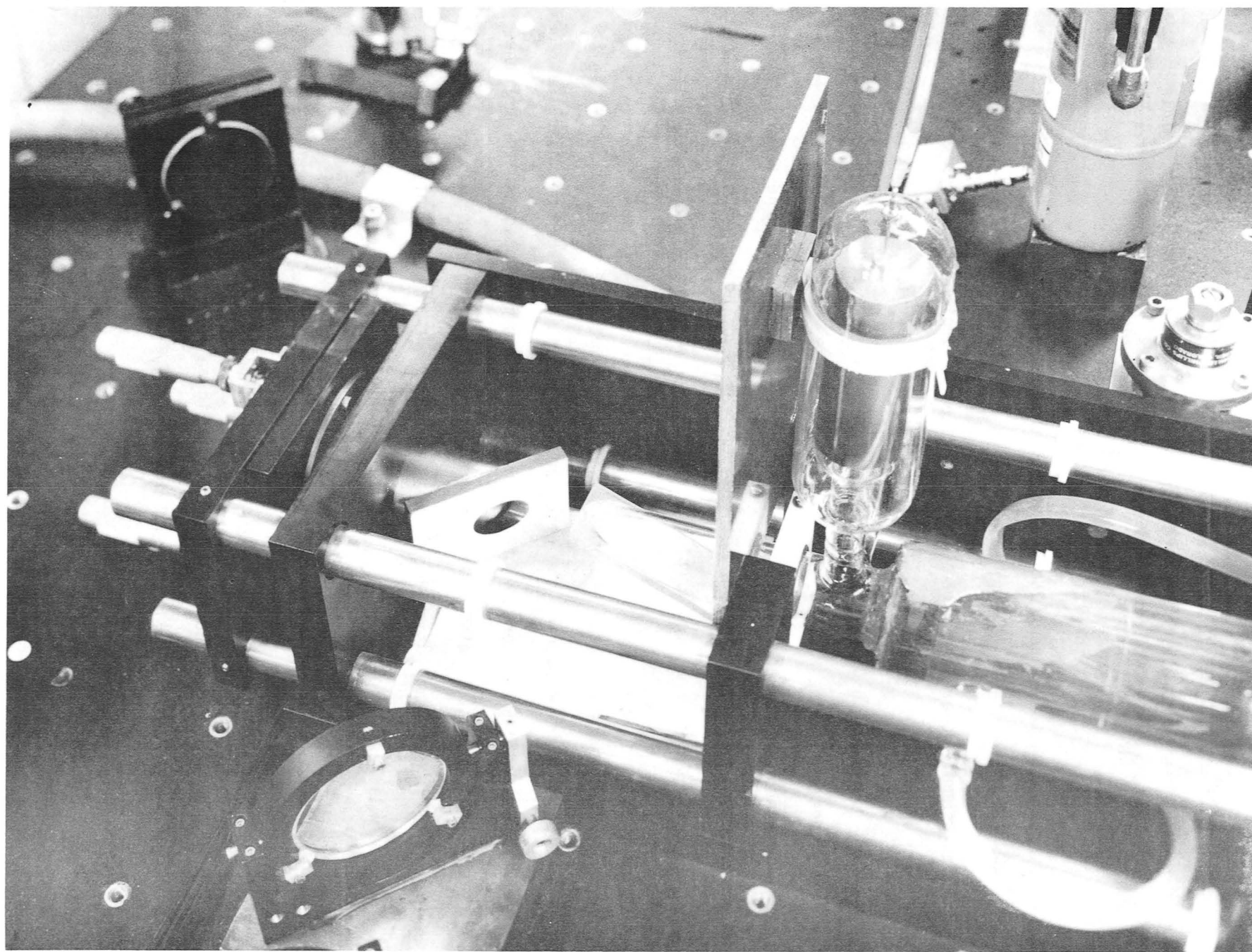
Figure 15. Scraper Mirror Assembly for Unstable Resonator
