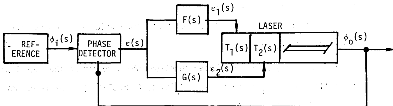
Figure 48. Closed-Loop System
