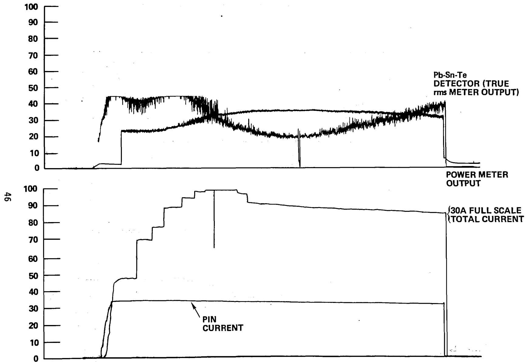
Figure 29. Chart Record of High Speed Detector, Power Meter, and Current Monitor Chart Speed: 1" = 60 sec.
