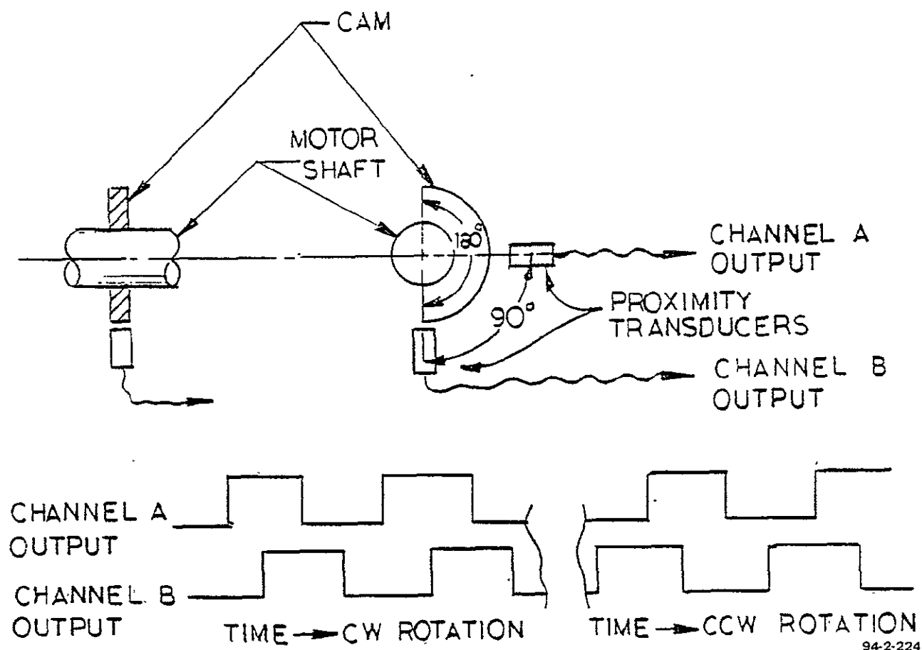
FIGURE 55. INCREMENTAL POSITION TRANSDUCER
