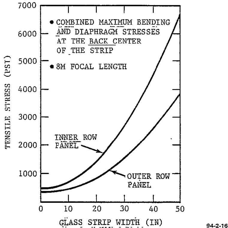
FIGURE 26. MAX TENSILE STRESS DUE TO ELASTIC CURVING
