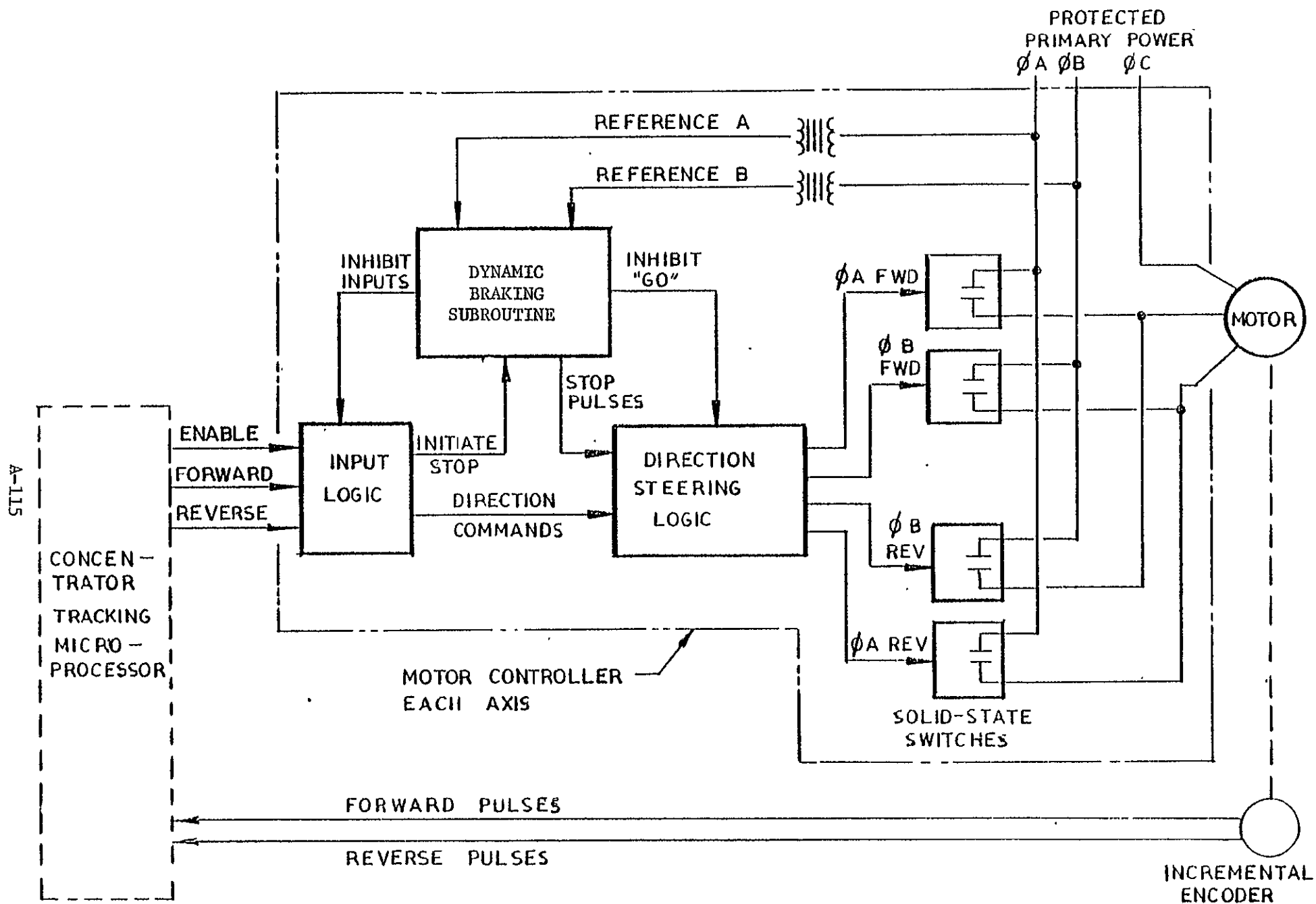
FIGURE 54. DRIVE SYSTEM BLOCK DIAGRAM
