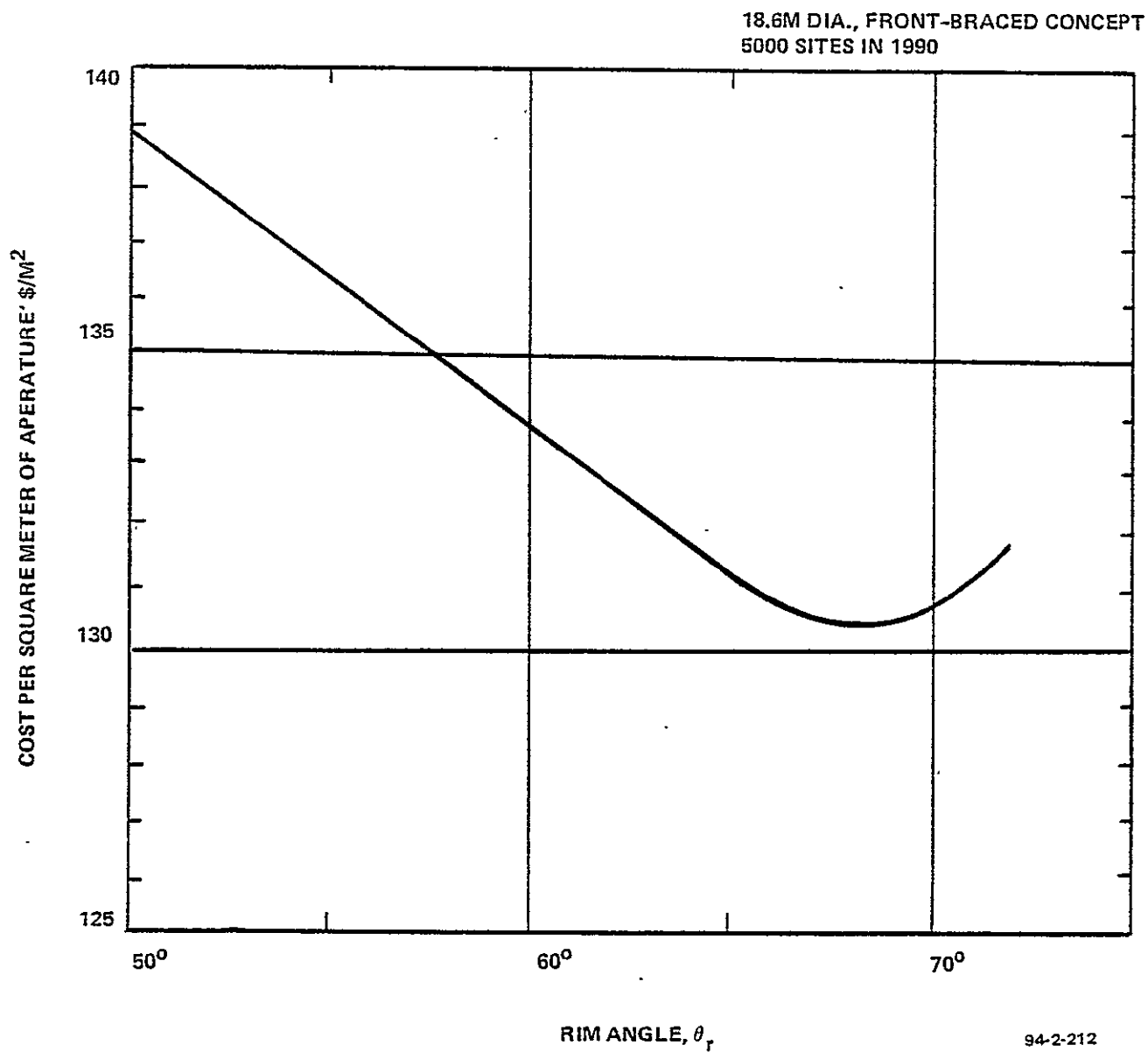
FIGURE 43. EFFECT OF RIM ANGLE ON CONCENTRATOR COST
