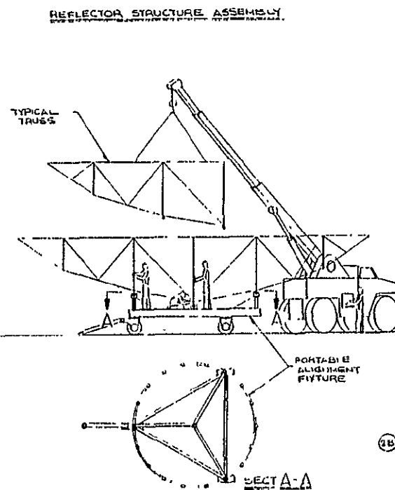
FIGURE 64. TYPICAL CONCENTRATOR INSTALLATION SEQUENCE (SHEET 1 of 2)
