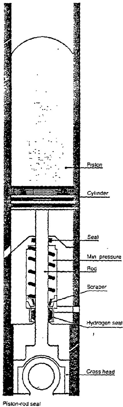
FIGURE 14. SKETCH SHOWING PISTON-ROD SEALS
