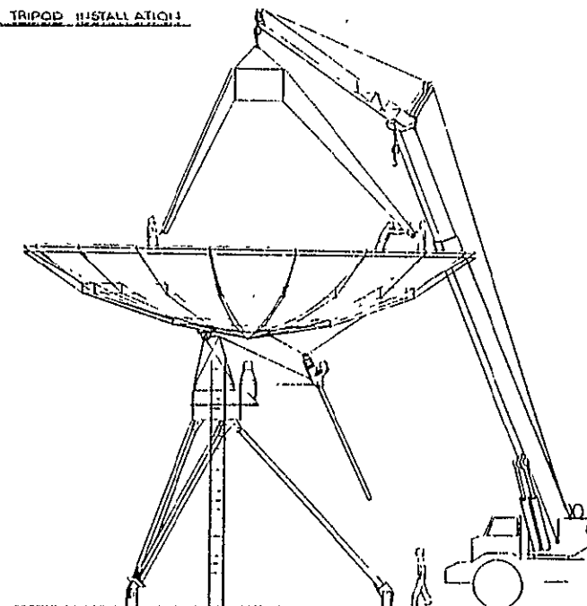
TRIPOD INSTALLATION
