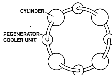
FIGURE 2. DOUBLE ACTING PISTON CONCEPT
