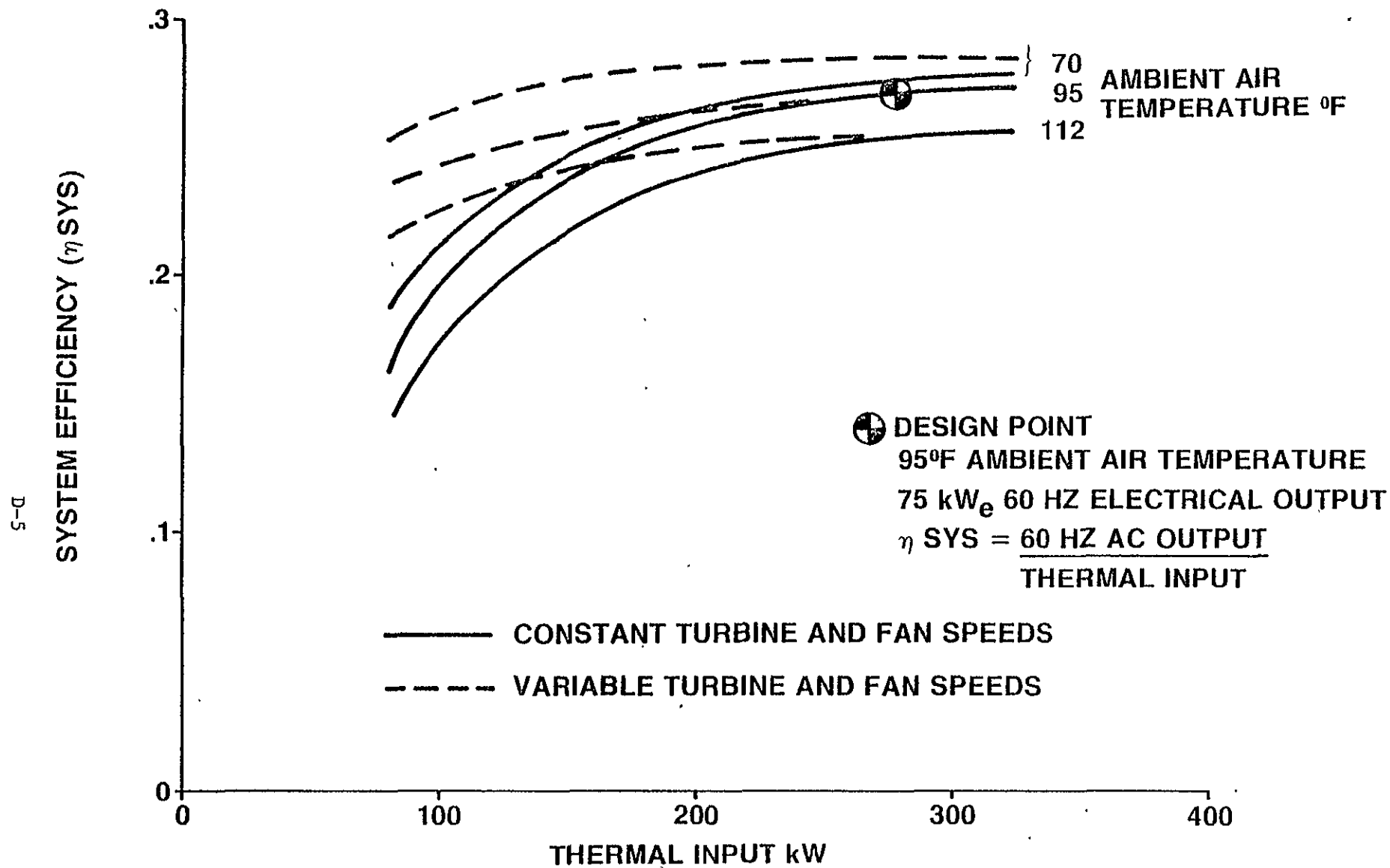
FIGURE 3. SOLAR POWERED ORGANIC RANKINE SYSTEM PERFORMANCE
