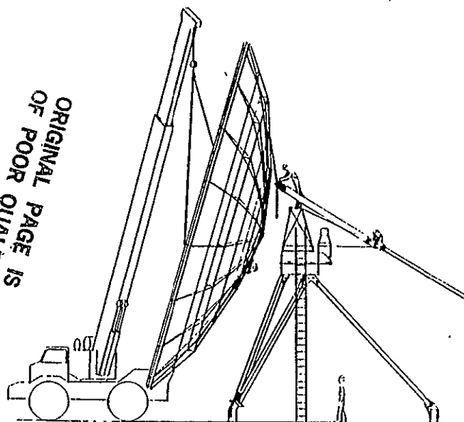
FIGURE 64. TYPICAL CONCENTRATOR INSTALLATION SEQUENCE (SHEET 2 of 2)
