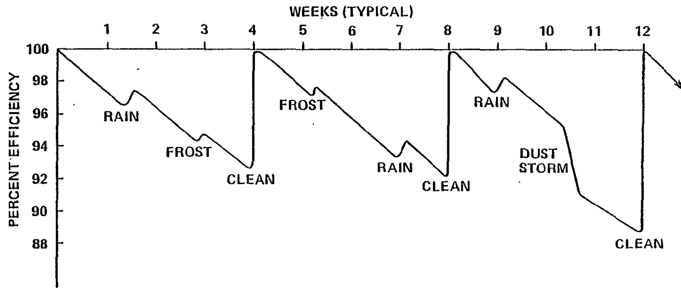
FIGURE 69. TYPICAL DIRT/DUST REFLECTIVITY LOSS
