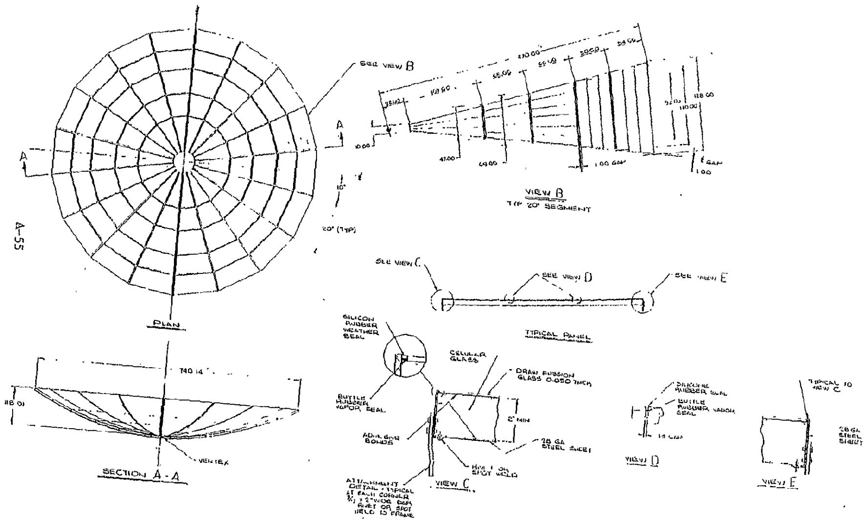
FIGURE 28. CELLULAR GLASS SANDWICH REFLECTOR PANEL DESIGN
