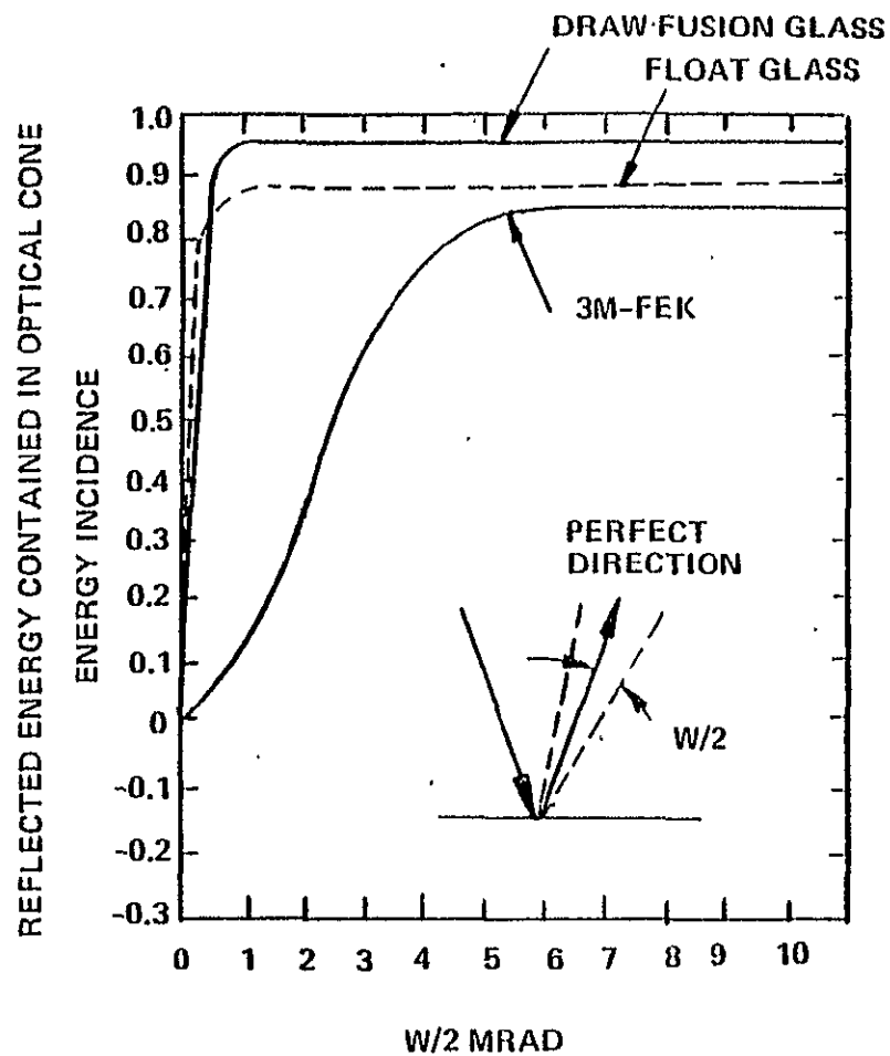
FIGURE 25. SPECULARITY PROPERTIES
