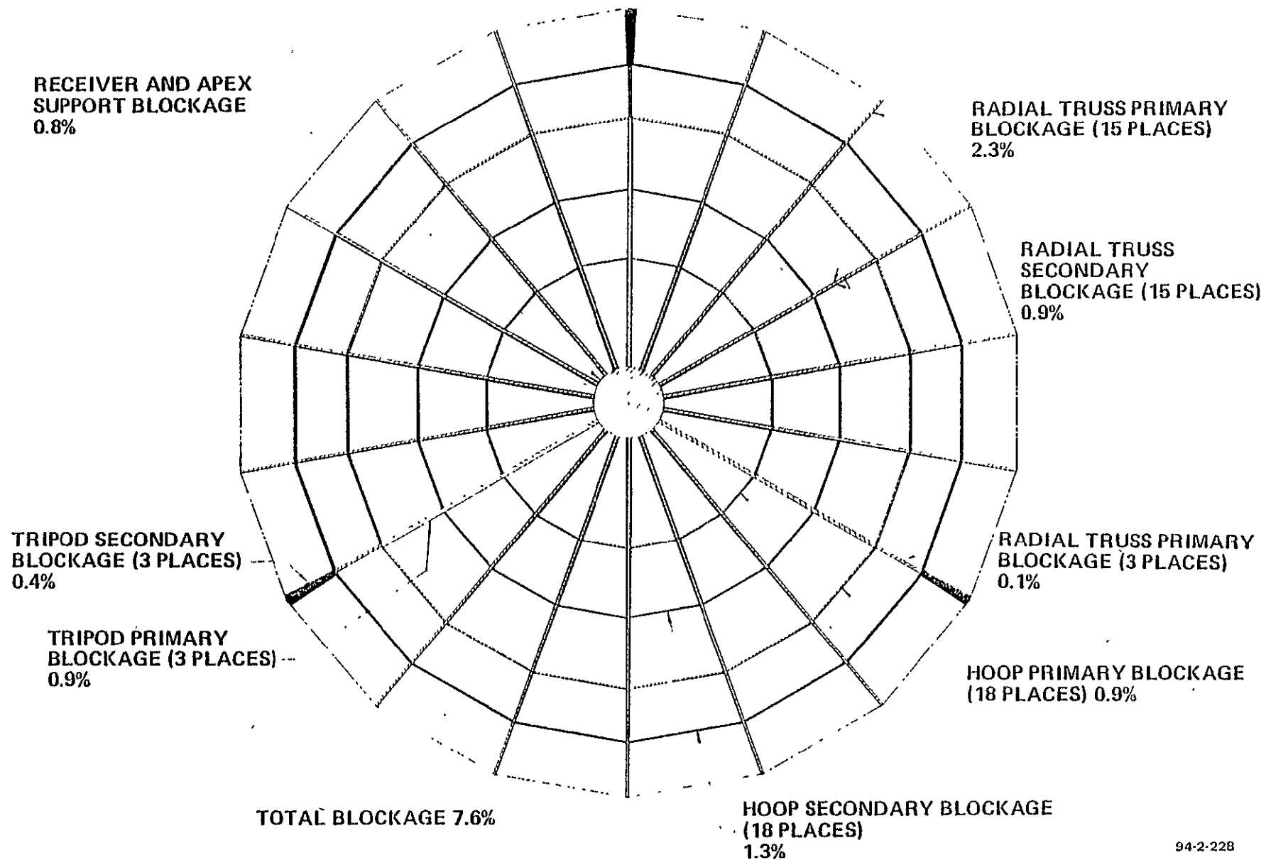
FIGURE 59. SHADOWING AND BLOCKAGE FOR THE BASELINE 18.6 METER CONCENTRATOR
