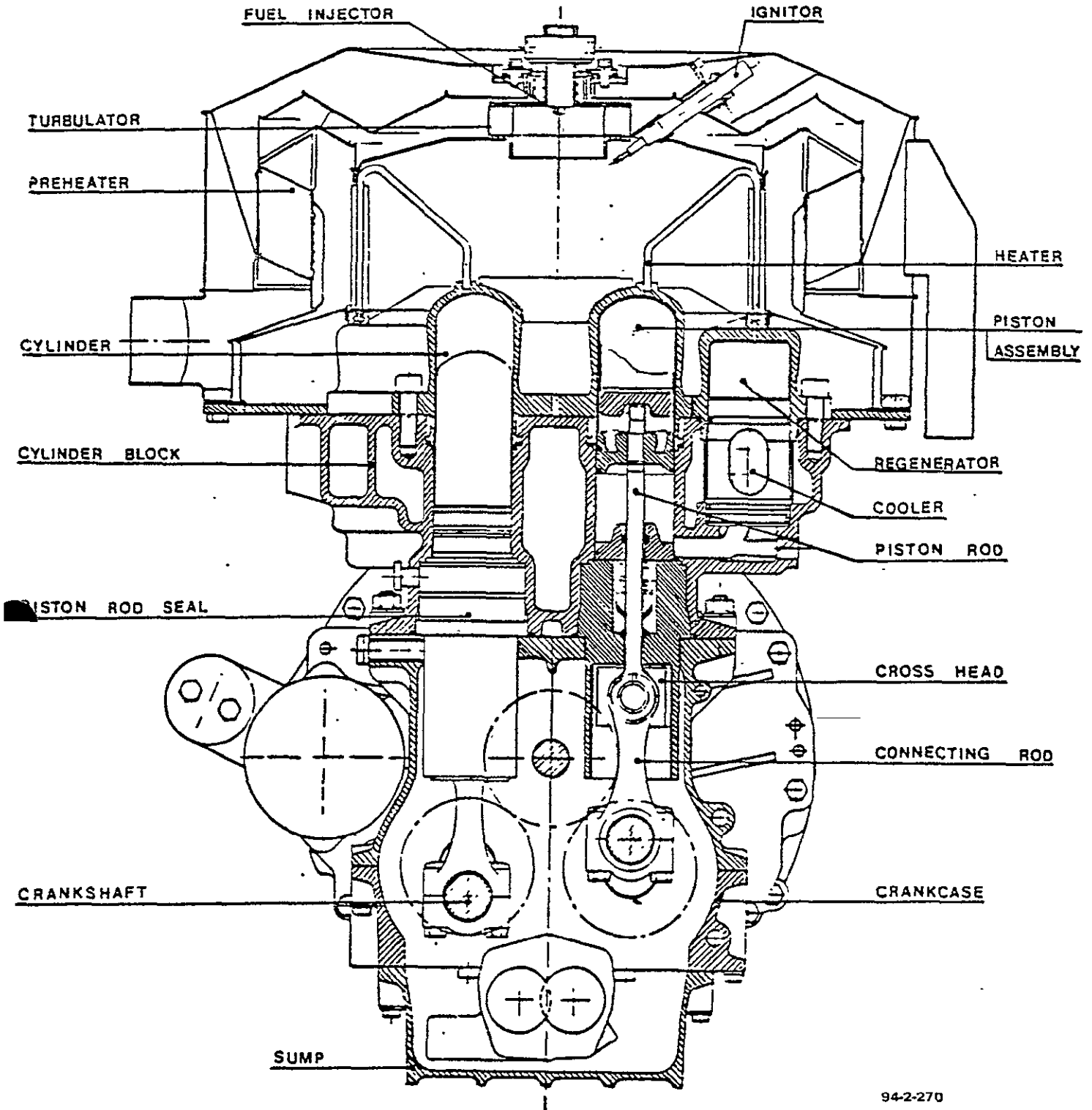
FIGURE 7. SCHEMATIC OF USS P-40 STIRLING ENGINE; U-CRANK CONFIGURATION
