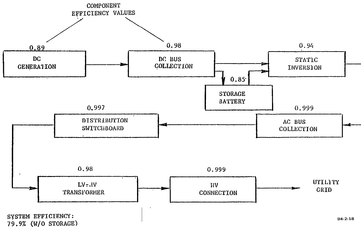
FIGURE 1. SYSTEM CONFIGURATION A
