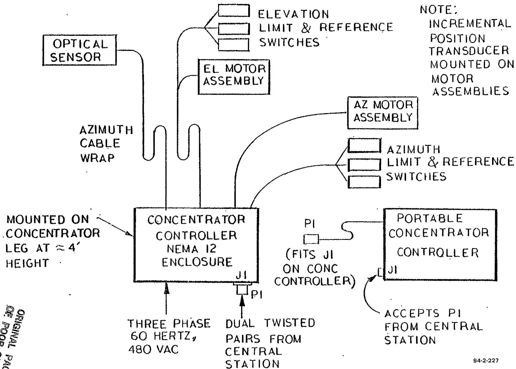
FIGURE 58. CONCENTRATOR CONTROL AND CABLING ARRANGEMENT
