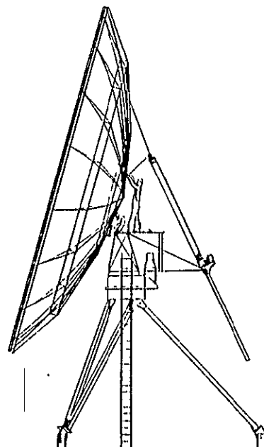
REFLECTOR TO TURRET CONNECTION
