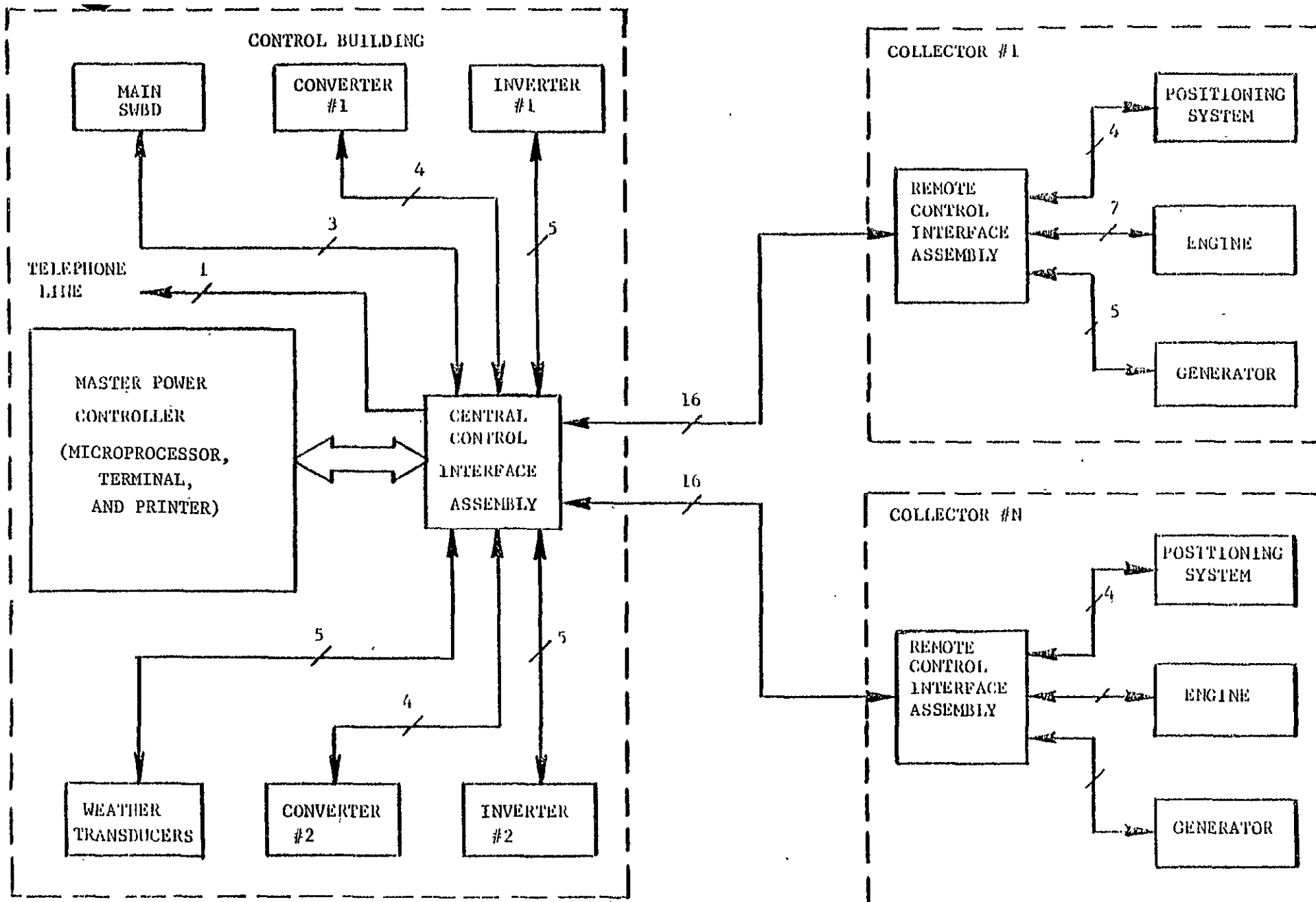
FIGURE 18. CONTROL SUBSYSTEM HARDWARE BLOCK DIAGRAM
