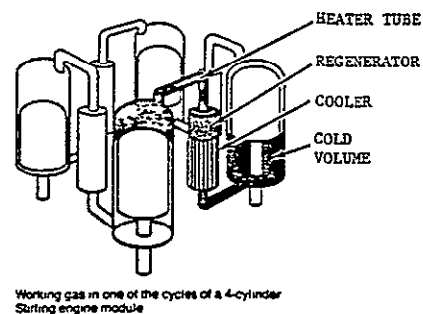
FIGURE 4. PISTON ARRANGEMENT OF DOUBLE ACTING CONCEPT
