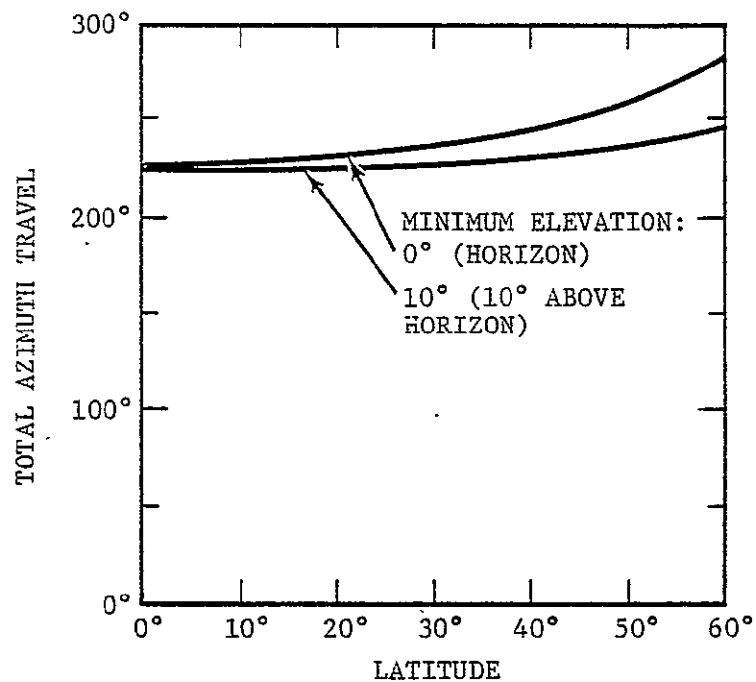
FIGURE 7. AZIMUTH COVERAGE
