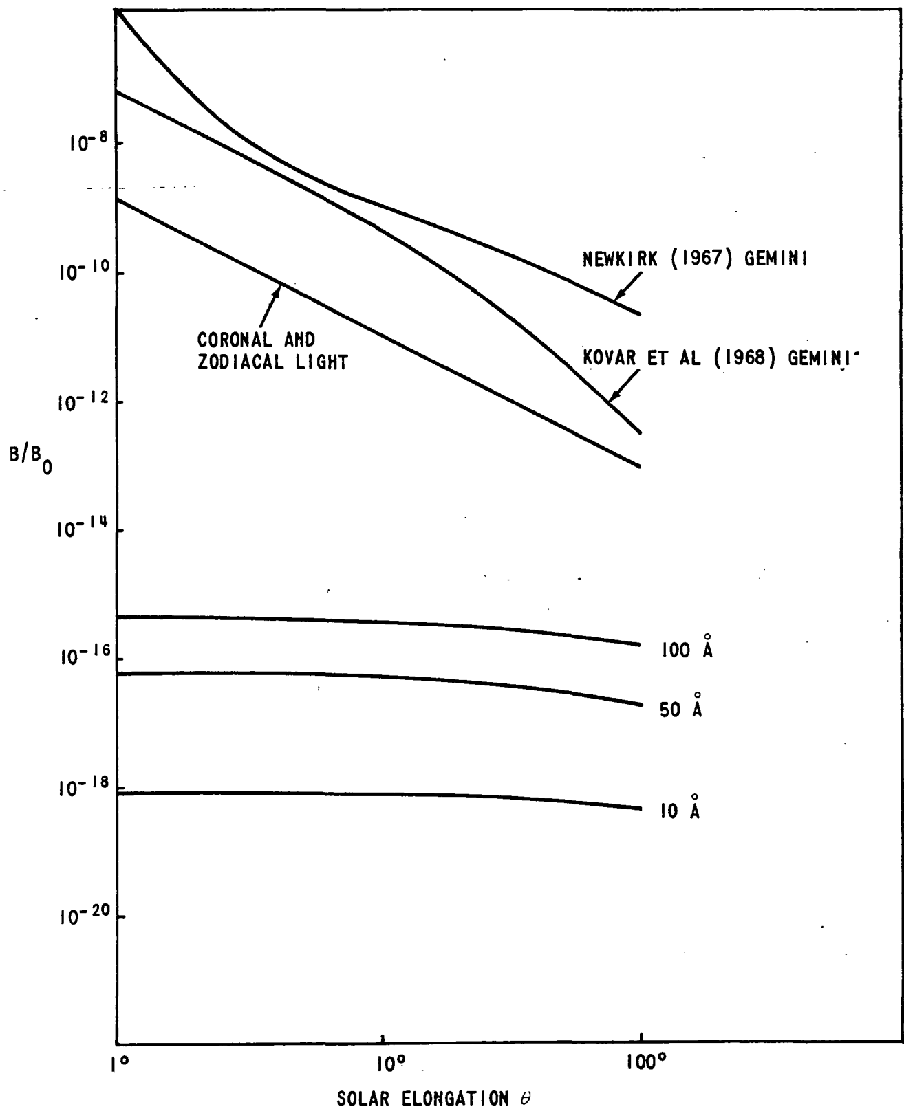
FIGURE 2 - DEBRIS CLOUD RADIANCE AS A FUNCTION OF SOLAR ELONGATION
