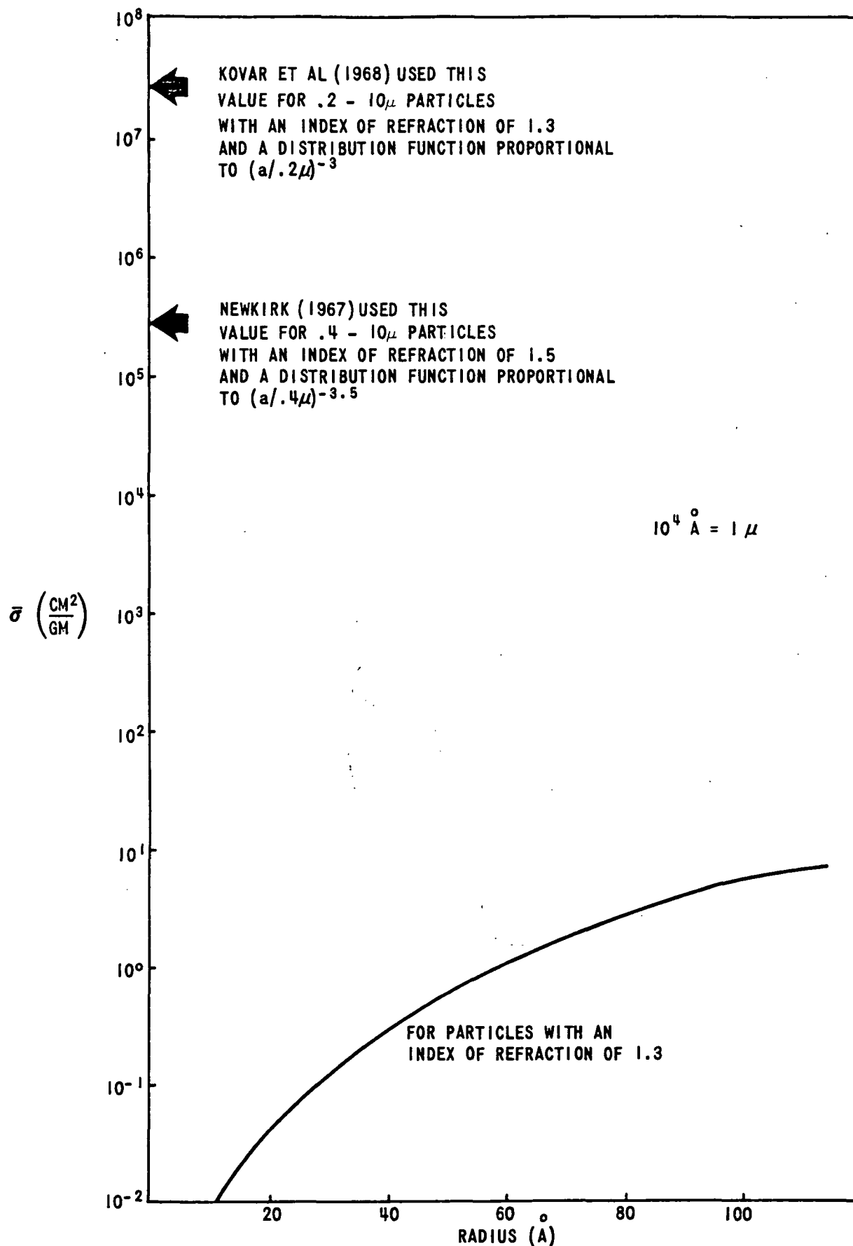
FIGURE 3 - THE TOTAL SCATTERING CROSS SECTION PER UNIT MASS AS A FUNCTION OF PARTICLE SIZE
