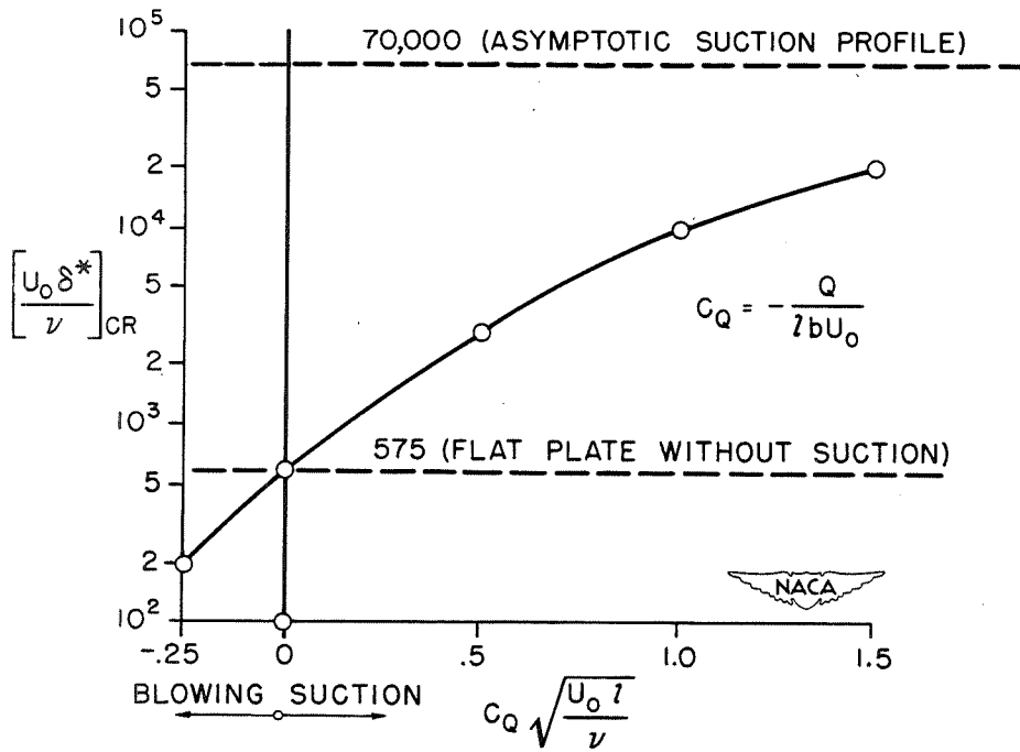
Figure 3.- Flow over a flat plate (V_0 \propto \frac{1}{\sqrt{x}}) .
