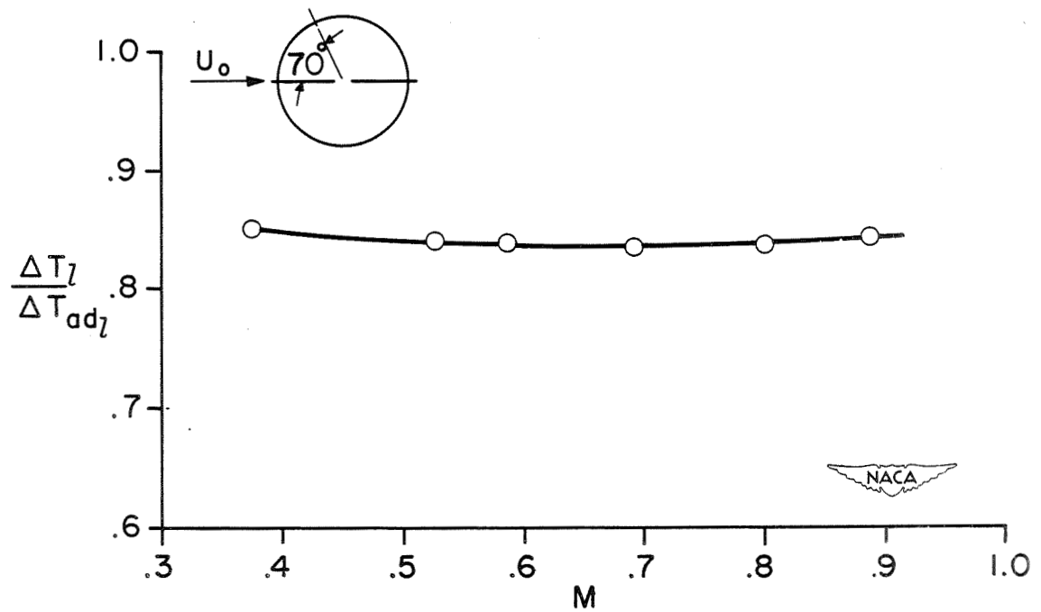
Figure 7.- Temperature recovery at 70° station on circular cylinder at various free-stream Mach numbers.
