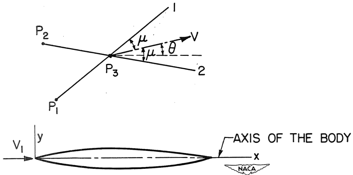
Figure 4.- Diagram illustrating scheme of characteristics method.
