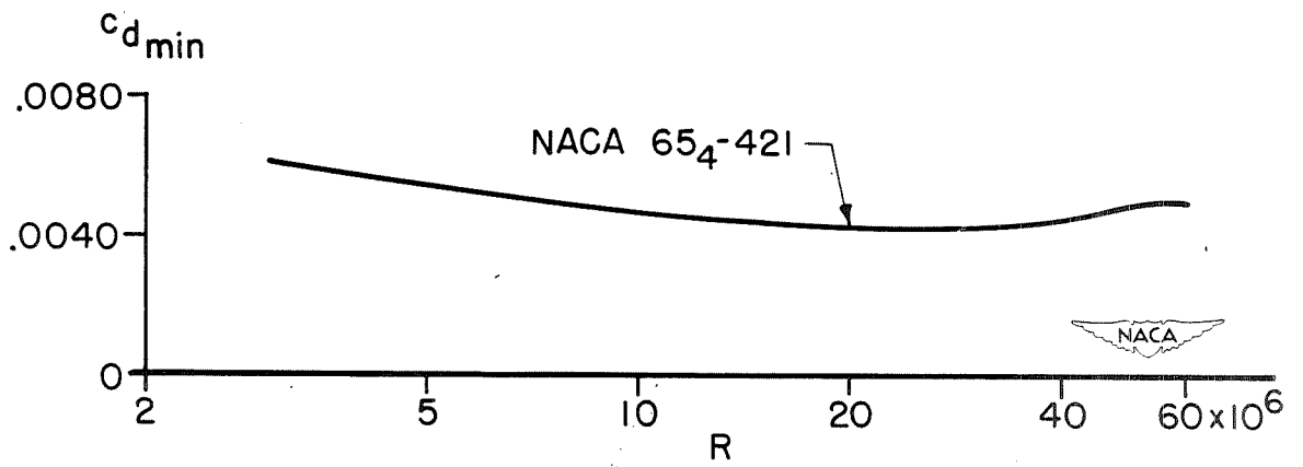
Figure 8.- Effect of Reynolds number on the minimum drag of the NACA 65 4 -421 airfoil section.
