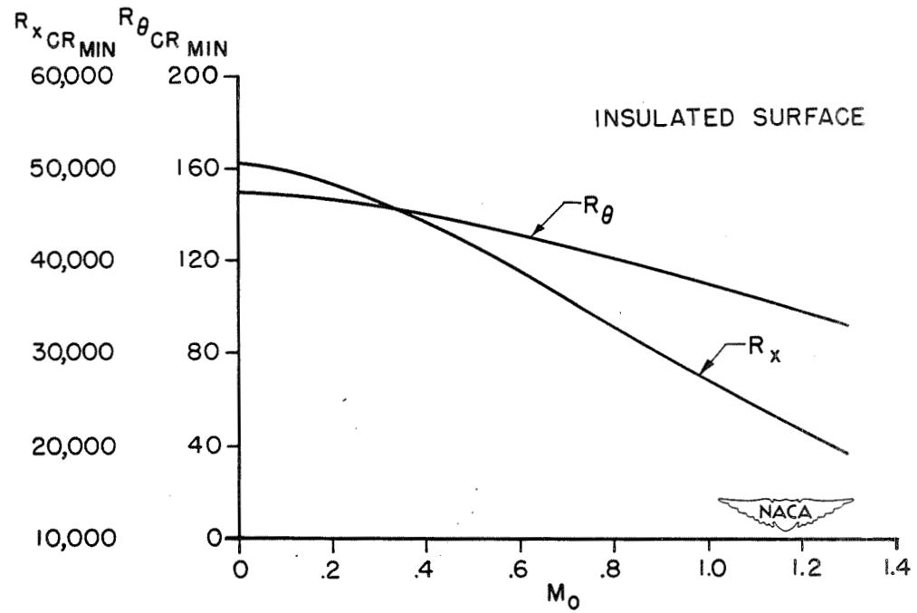
Figure 6.- Critical Reynolds number against Mach number.
