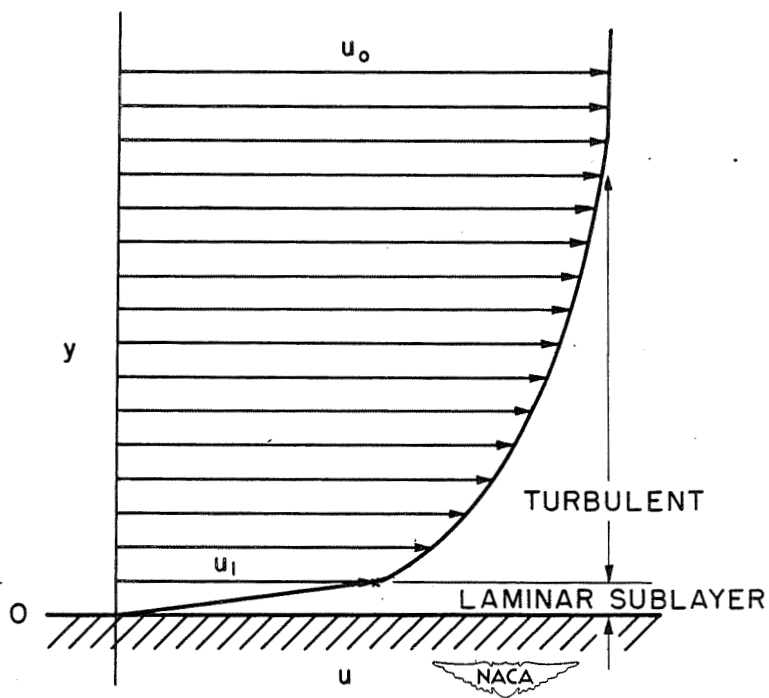
Figure 4.- Assumed turbulent-velocity profile.
