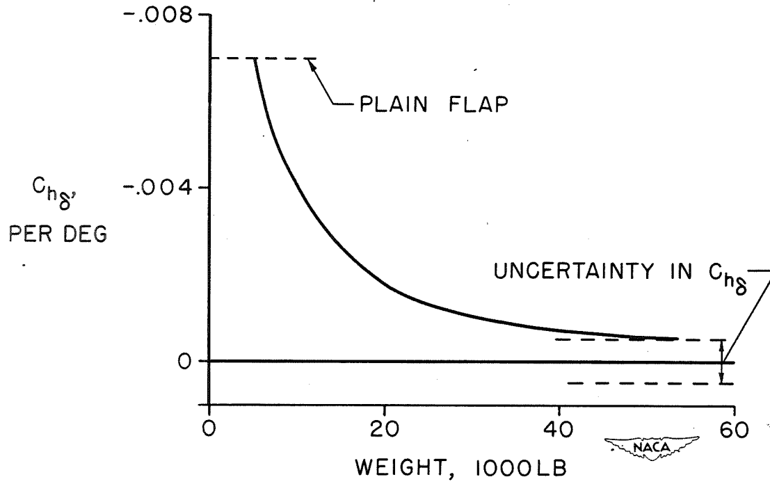
Figure 5.- Elevator balance.
