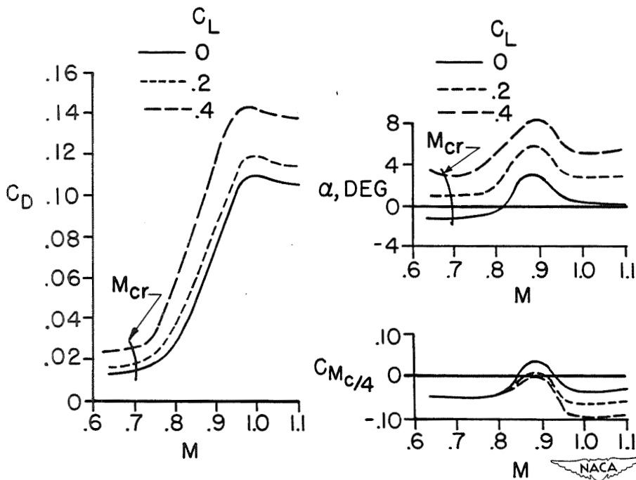
Figure 2.- Transonic force data for a typical wing. NACA 65 (112) -213, a = 0.5 airfoil; aspect ratio, 6.4.
