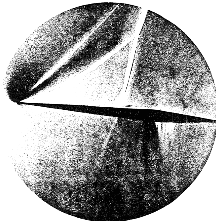
Figure 15.- Schlieren flow photograph of NACA 1S-(70)(03)(70)(03) airfoil. \alpha = 5.5^\circ ; M = 0.75 .
