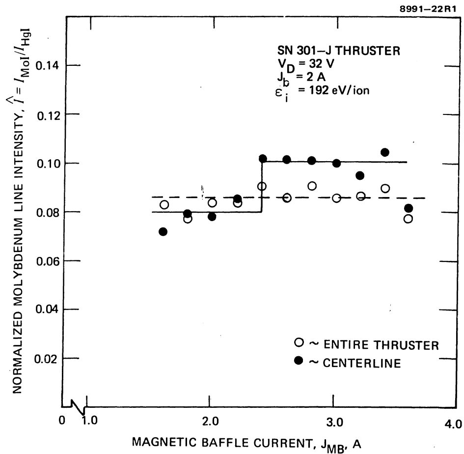
Figure 2-24. Variation of normalized molybdenum line intensity with magnetic baffle current. ( \lambda_{\text{MoI}} = 3798.3 \text{ \AA} , \lambda_{\text{HgI}} = 3801.7 \text{ \AA} ).
