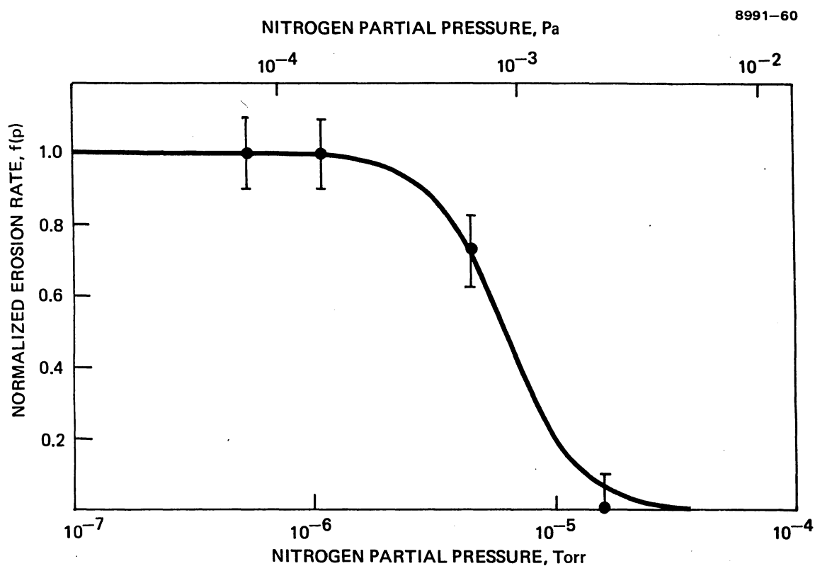
Figure 2-38. Variation of the normalized sputtering-rate function with the partial pressure of nitrogen; comparison of experimental values and curve-fit based on the model. The curve-fit is described by f(p) = (1 + 3.6 \times 10^{14} p^{2.8})^{-1} for the pressure p in Torr.
