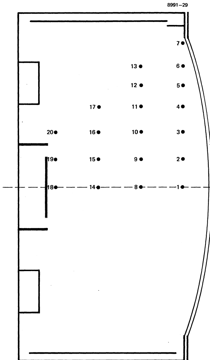
Figure 2-27. Locations of Langmuir-probe measurements performed in the SN 301-J thruster.
