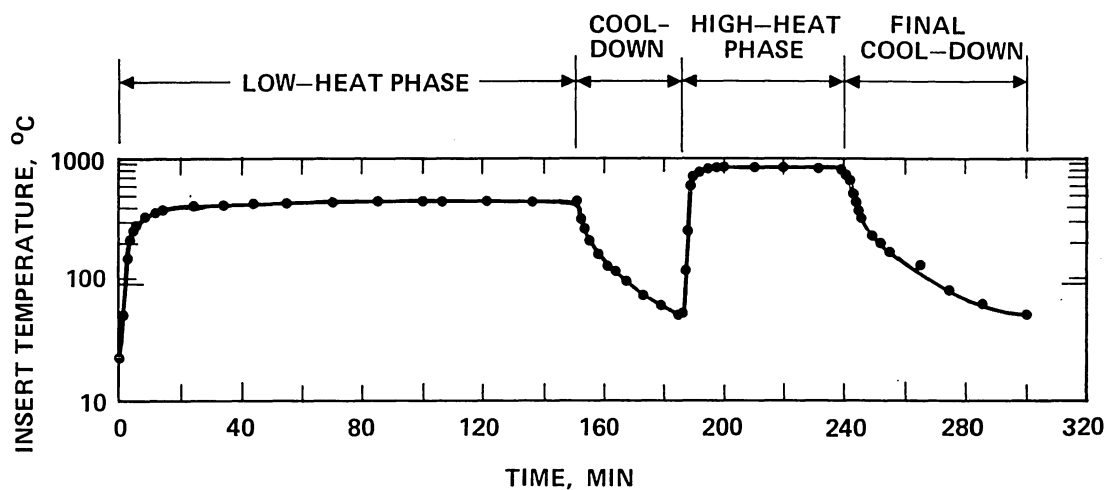
Figure 3-12. Time history of insert temperature during cathode conditioning cycle (upstream thermocouple location, T_2 ).
