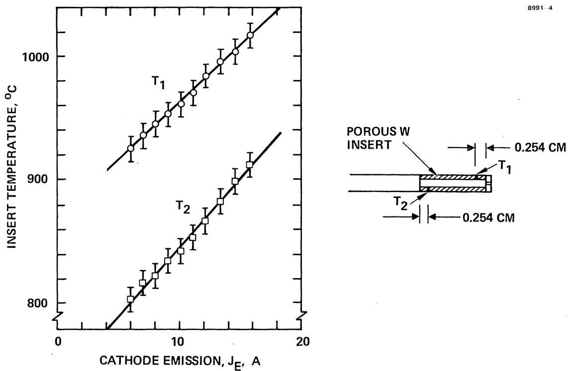
Figure 3-5. Variation of porous-tungsten insert temperature with cathode emission current J_E . ( V_D = 32 V, J_b = 0.2 J_E - 0.4 A).
