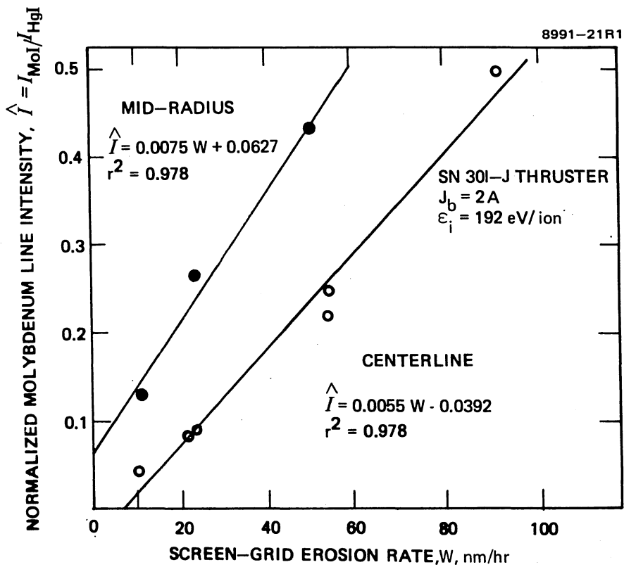
Figure 2-17. Correlation of molybdenum line intensities with screen-grid erosion rates. ( \lambda_{\text{MoI}} = 3798.3 \text{ \AA} , \lambda_{\text{HgI}} = 3801.7 \text{ \AA} ).
