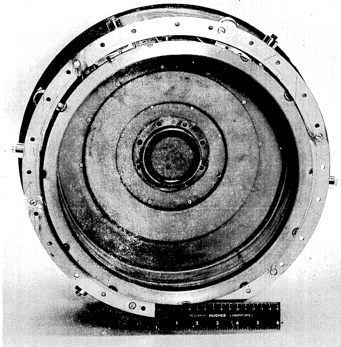
Figure 2-1. Photograph of SN 301-J thruster.
