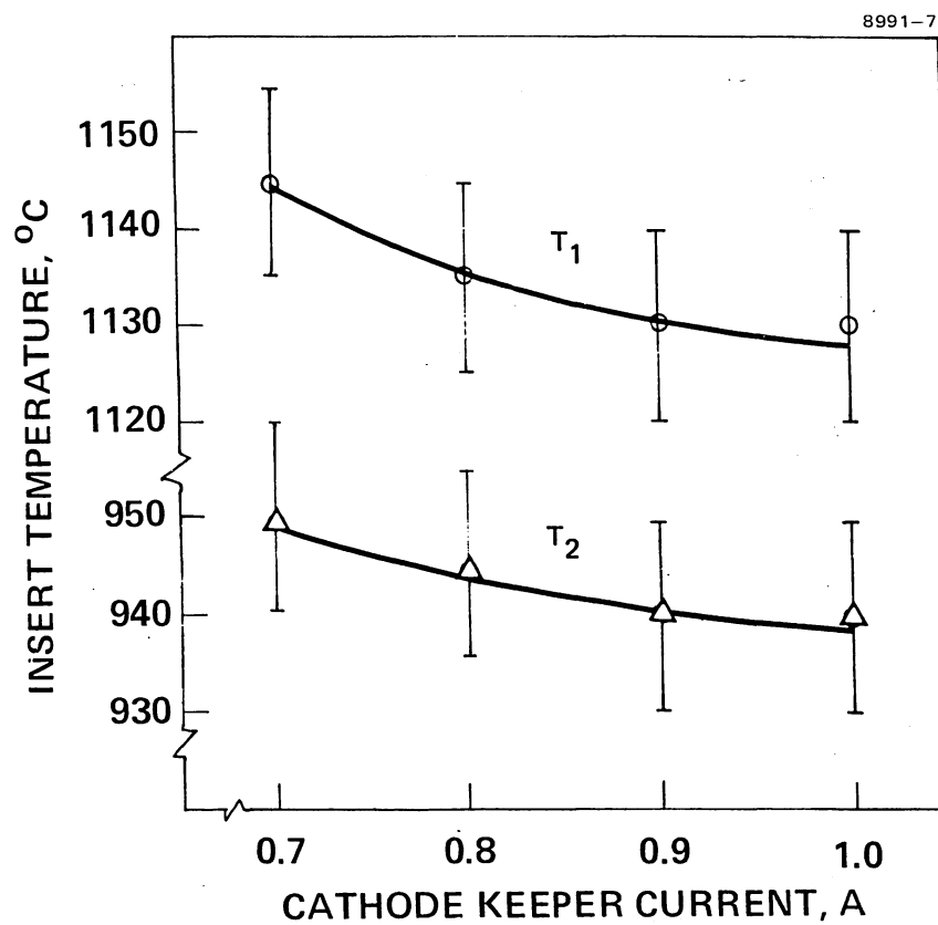
Figure 3-8. Variation of insert temperature with cathode-keeper current, keeper voltage also varied, other parameters constant. ( J_E = 12 A, V_D = 32 V, J_b = 2 A).
