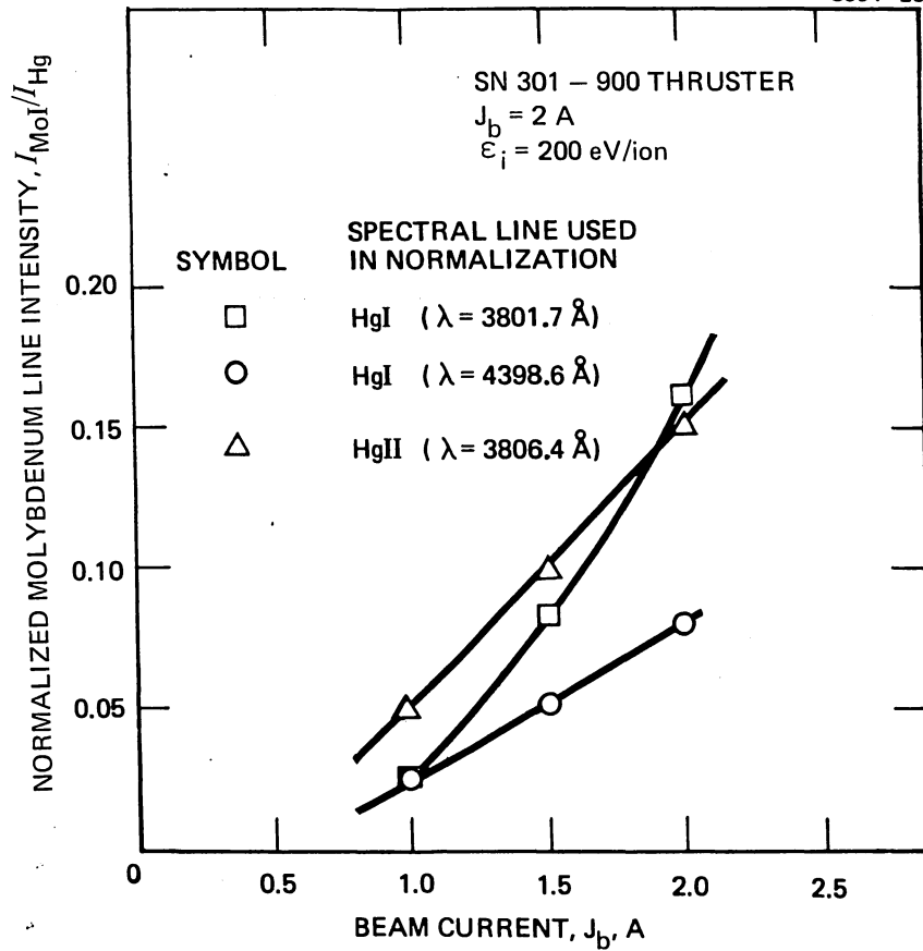
Figure 2-13. Variation of molybdenum line intensity with beam current. (MoI line measured at a wavelength of \lambda = 3798.3 \text{ Å} ).
