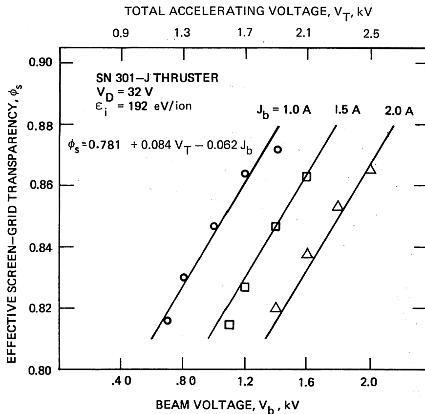
Figure 2-26. Variation of screen-grid transparency with beam current and beam voltage. (The optical or geometric transparency of the screen electrode is \phi = 0.674 .)
