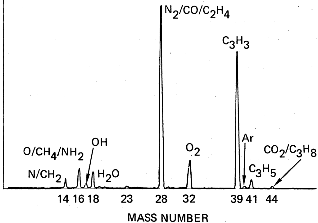
Figure 2-5. Typical mass spectra recorded in the Hughes 9-ft vacuum test chamber.
