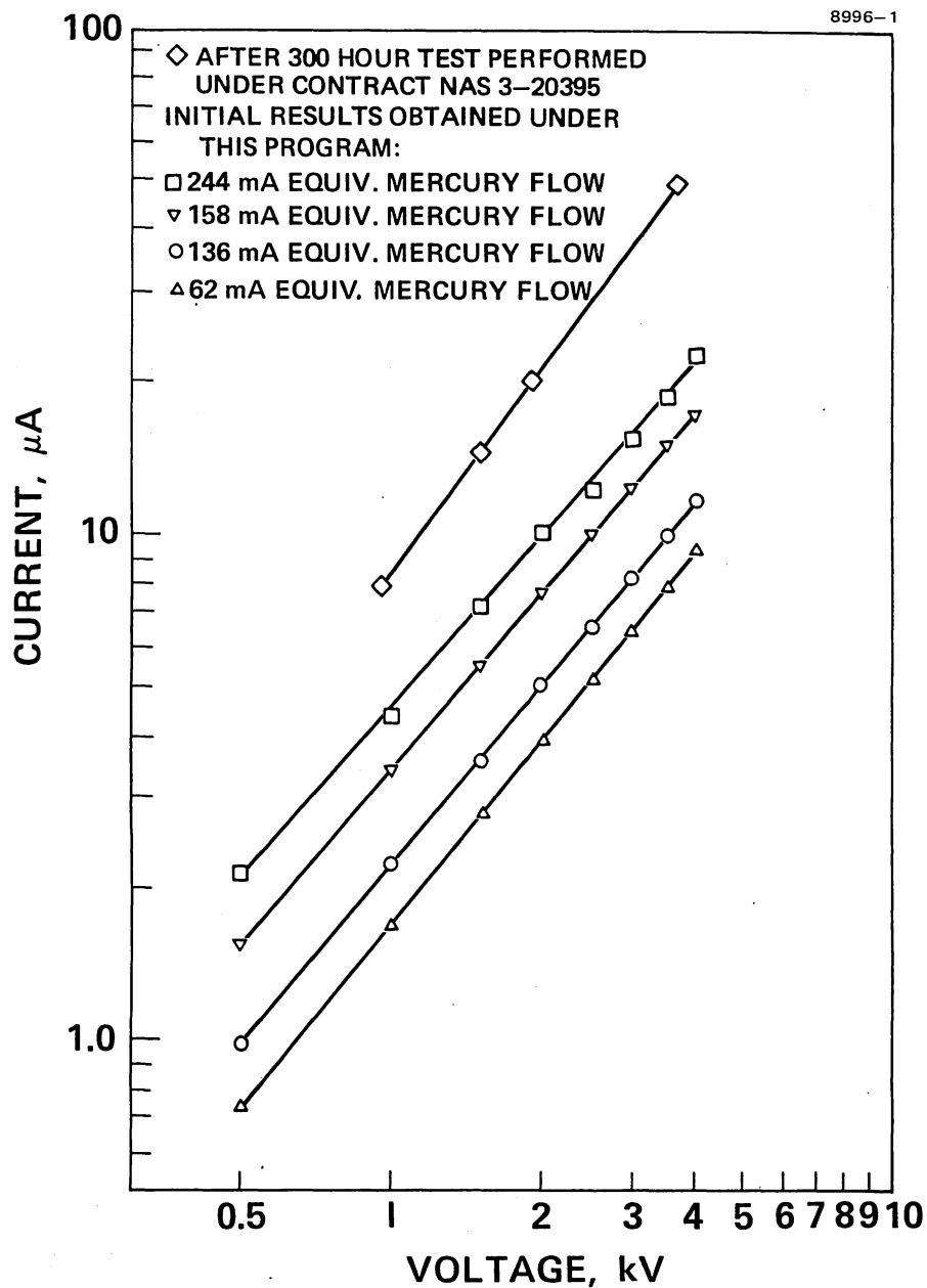
Figure 5-5. Comparison of leakage current versus voltage for test performed after 300-hr test and for initial tests performed under this program. (This isolator was later found to be contaminated.)
